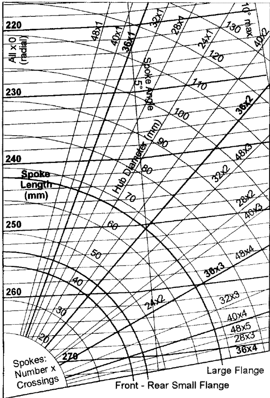
Spoke Length Chart for 559 (26mtb) Rims
