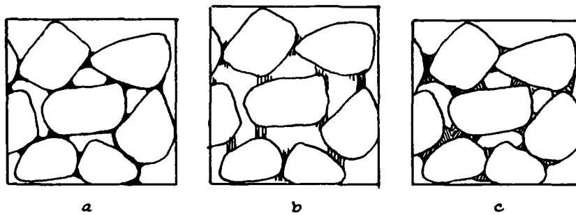
Figure 31. Diagram showing two different possibilities of freezing of non-saturated soil (moist sand) a = the sand before freezing. Its funicular water ("Por-winkelwasser") at freezing may form either expanding ice needles between the particles (b), causing the soil to expand much greater than the 10% increase due to water freezing, or the ice crystals may grow in the free spaces of the pores (c), and the soil specimen not expand. Between these extremes, all kinds of transitions may occur. The experiments have shown that the phenomenon depends on the pressure. For no pressure [surcharge load], noticeable expansion can occur, but even a small pressure will reduce this expansion practically to zero.
