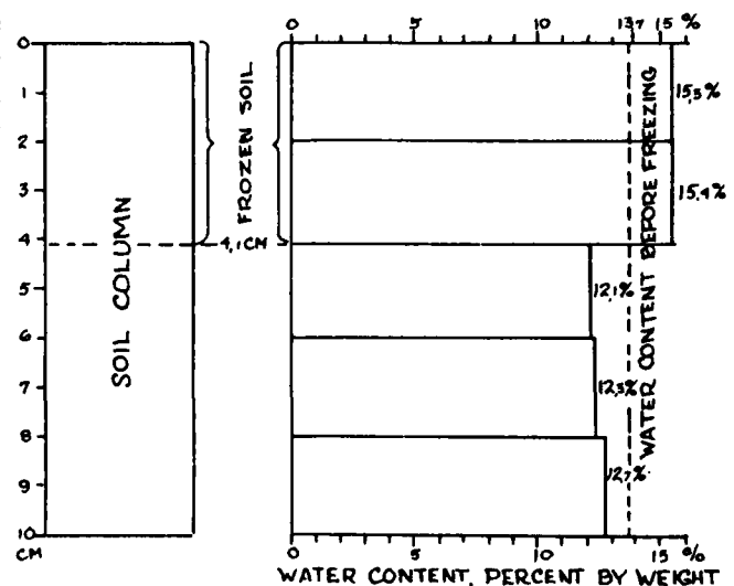
Figure 33. Water distribution after freezing of a column of moist (13.7% water) silt (BW 19). Surcharge load = 50 \text{ gr/cm}^2 ; freezing time 3\frac{1}{2} hours. No trace of heaving. Compare with Figure 32.
