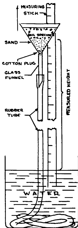
Figure 72. Simplified type of capillarity intended for field use for the determination of the capillarity of sand and coarse silts, and thus distinguished between frost heaving and non-frost-heaving sediments (from Beskow 1933a, 1934b). Mercury is not used in this apparatus; instead the whole system is filled with water. After the soil sample is placed at a consistency about the liquid limit (during which the tube is kept closed by a clamp), the excess water is sucked out by holding the funnel a few decimeters above the water surface. The funnel is then raised slowly, and the level at which the air breaks through is observed. By using a table, ladder, etc., capillarities up to 3 m can be determined, which is a large enough range to determine the degree of frost-heaving danger.
