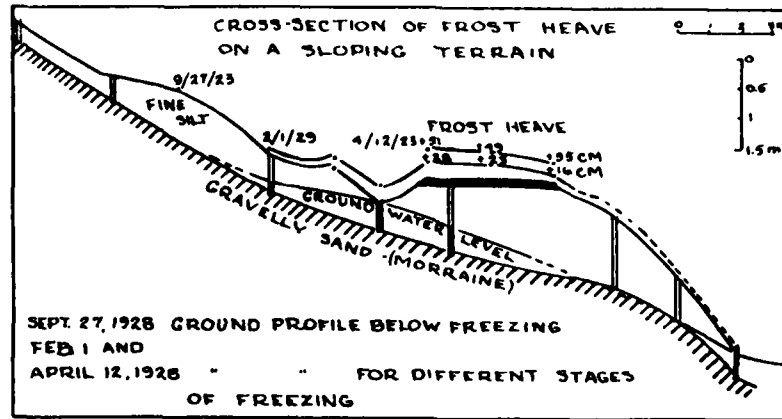
Figure 50. Cross sectional profile of a road on a steep slope, showing uneven heaving, caused by the sloping groundwater table. Soil: fine silt with gravel and sand layers. It is seen that the amount of frost heave is approximately inversely proportional to the distance to groundwater. [The numbers +28, and +16 are the heaves in centimeters of the left edge, center and right edge respectively of the road on Feb. 1, '29. Likewise, +51, +42, +35 are heaves on March 12, '29. The lowest solid line is the profile of the ground including the road surface before frost heaving.]
