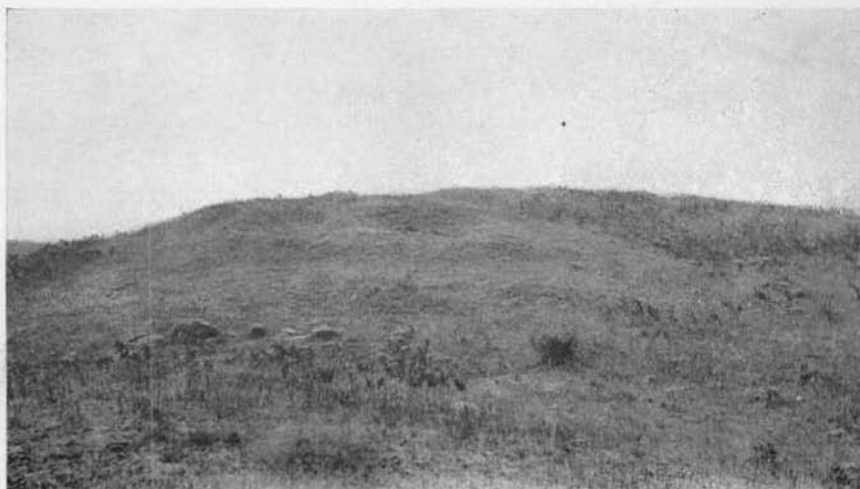
FIG. 1. Ford Type Mound on Grand Mound Prairie.
