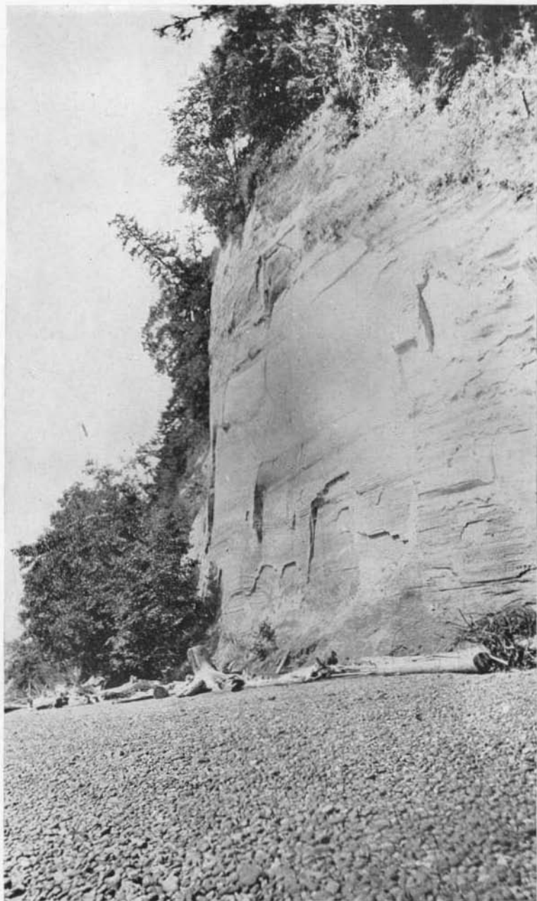
Cole Point, Anderson Island.
