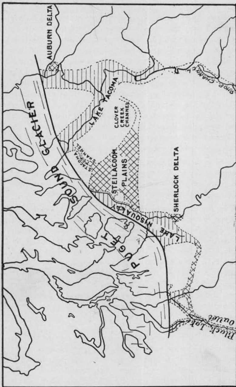
FIG. 10. Lake Tacoma, Lake Nisqually and Early Lake Russell.
