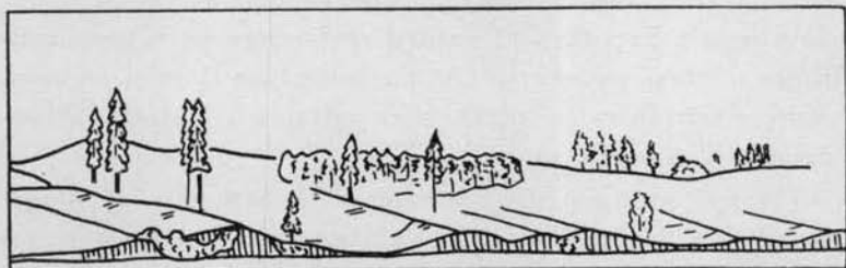
FIG. 24. North Shore of Hales Passage, showing drumlinoid till ridges truncated by sea cliffs. Drawn from a photograph.
