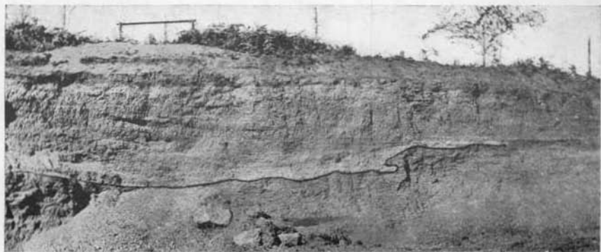
FIG. 3. Section of Red Gravel in Satsop Terrace.
