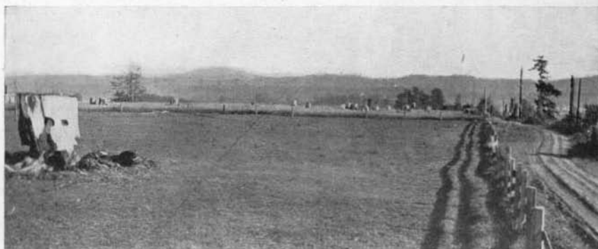
FIG. 2. Surface of Satsop Red Gravel Terrace.
