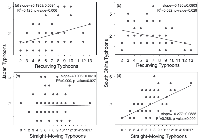
Fig. 5. Annual number of Japan and south China typhoons vs recurving and straight-moving typhoons. (a) Japan vs recurving, (b) south China vs recurving, (c) Japan vs straight-moving, and (d) south China vs straight-moving. Lines indicate the best linear fit. Slope values and standard errors along with R 2 and p-values corresponding to the best fit are given in each panel
