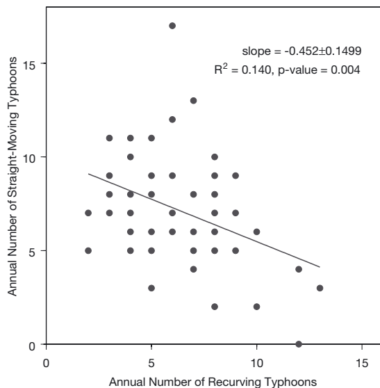
Fig. 3. Annual number of recurving vs straight-moving typhoons. The line indicates the ordinary least-squares best fit. The slope and SE along with the R^2 and p-value are given in the figure
