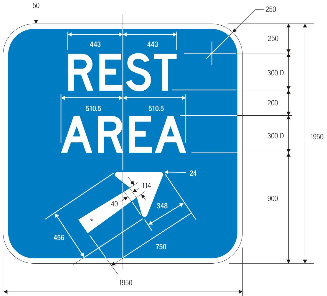
D5-2b REST AREA GORE SIGN
