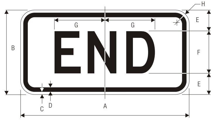
M4-6 END AUXILIARY
