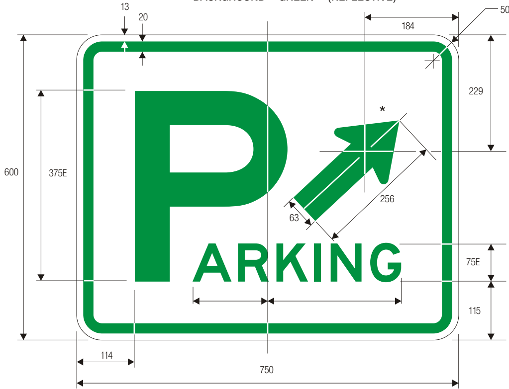
D4-1 PARKING AREA
