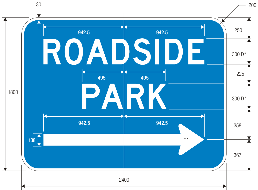
D5-5b ROADSIDE PARK ARROW
