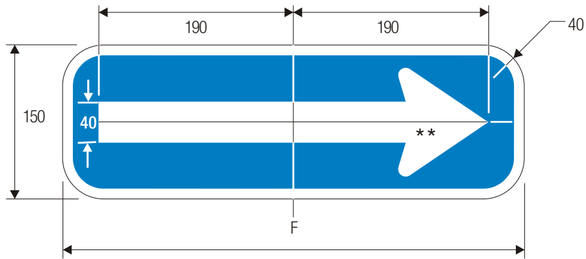
ROADSIDE TABLE SYMBOL
