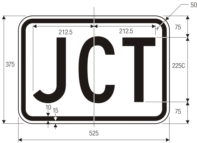
M2-1 JUNCTION AUXILIARY
