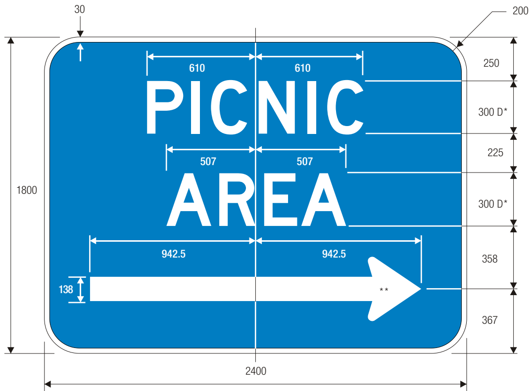
D5-5c PICNIC AREA
