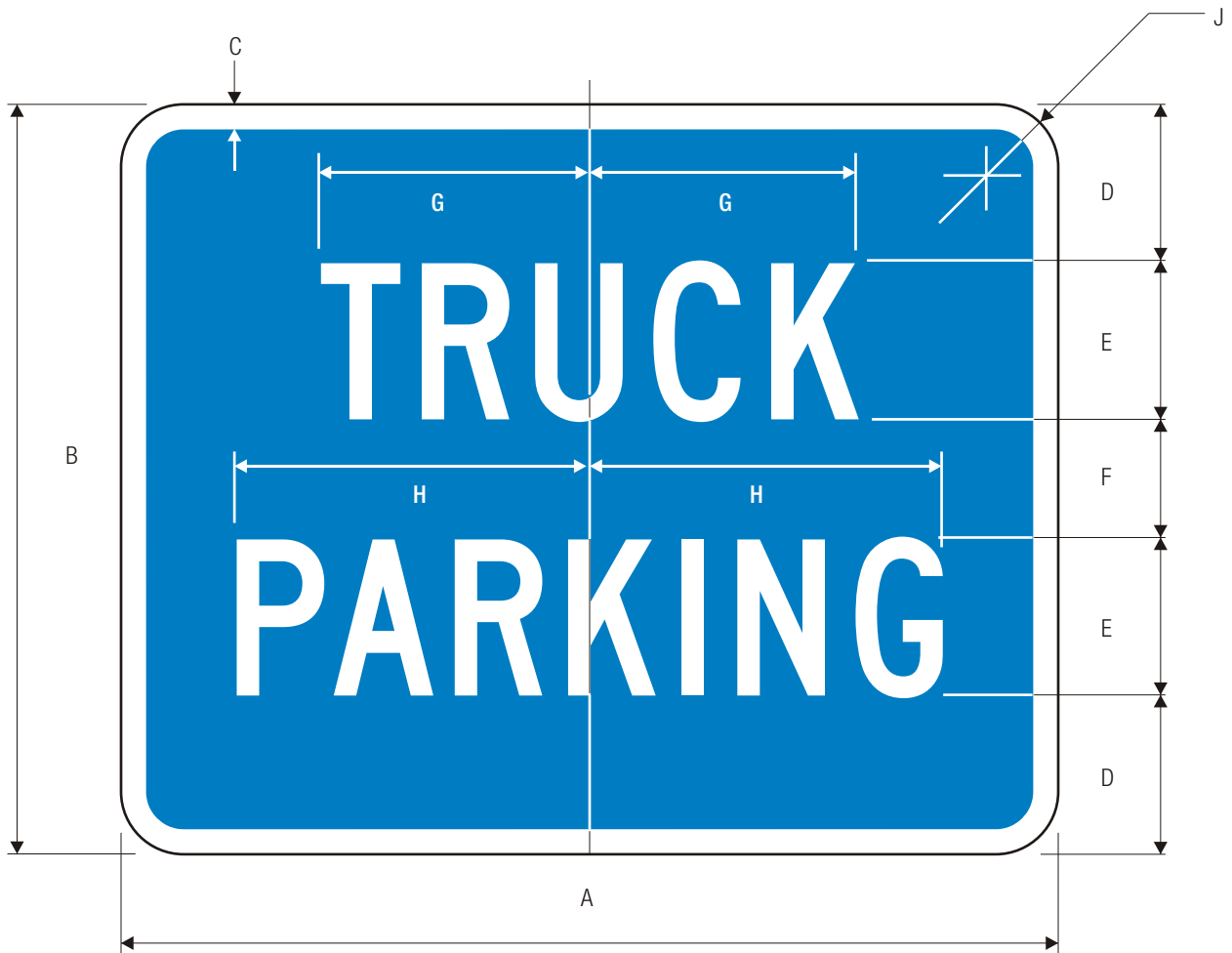
D9-16 TRUCK PARKING
