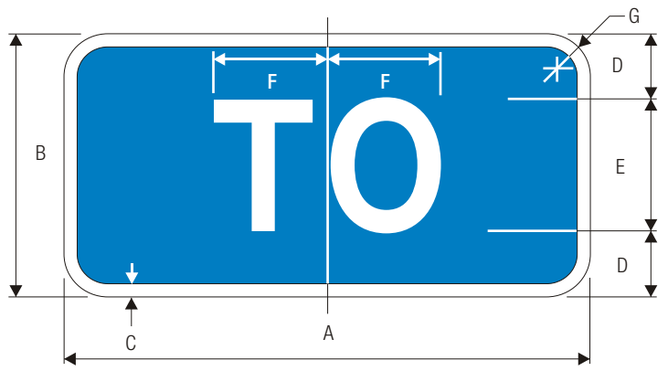
M4-5 (INTERSTATE) TO AUXILIARY
