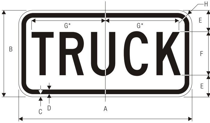
M4-4 TRUCK AUXILIARY
