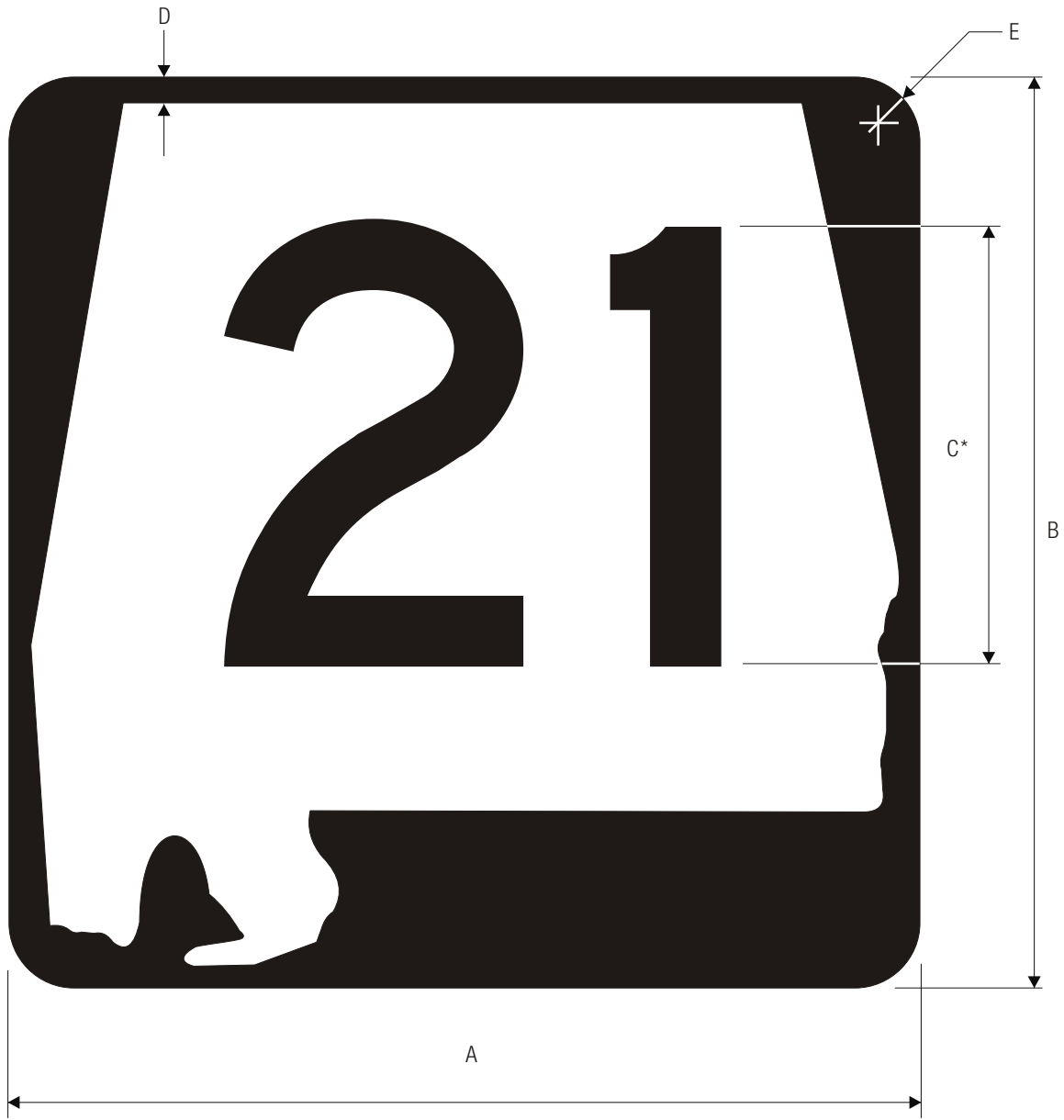
M1-5 STATE ROUTE
