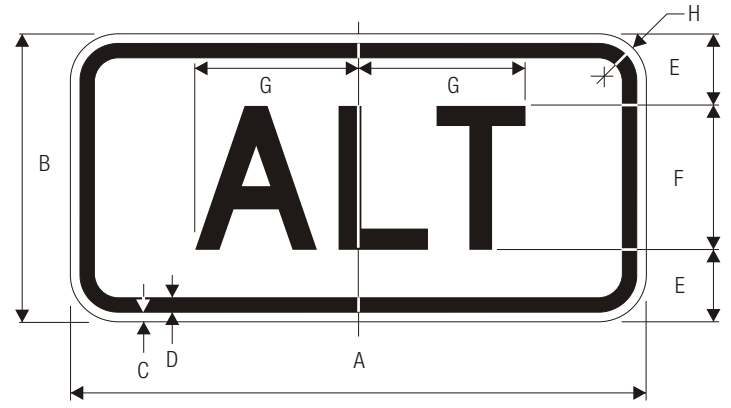
M4-1a ALTERNATE AUXILIARY
