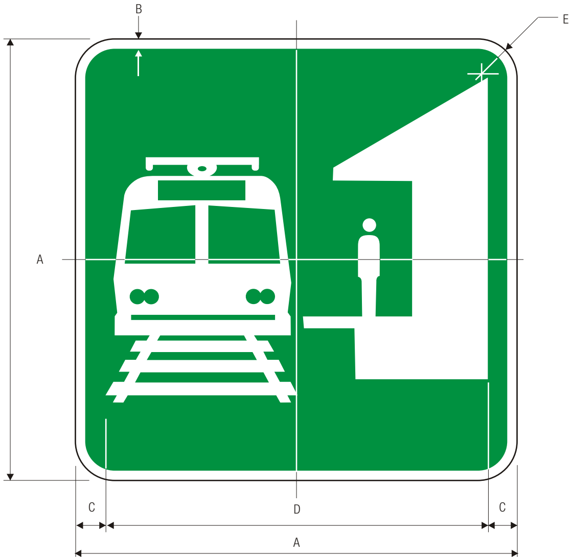
I-12 LIGHT RAIL STATION
