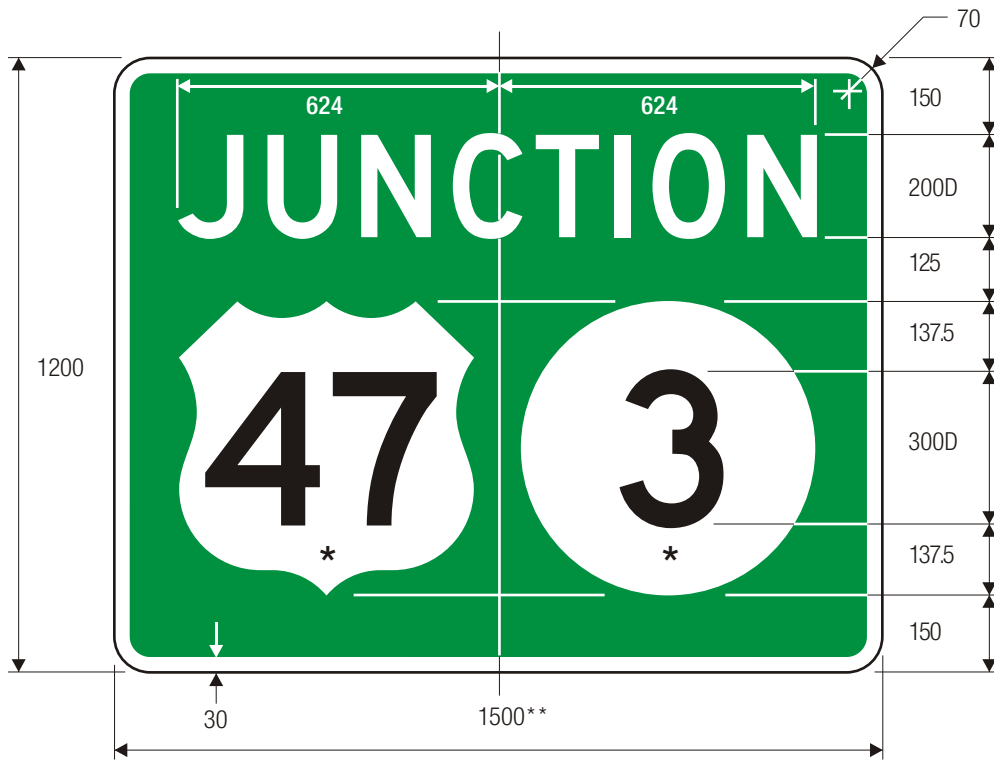
M2-2 COMBINATION JUNCTION
