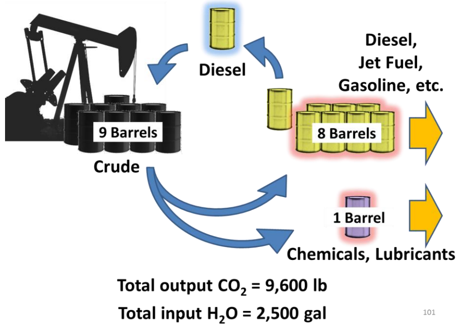
Figure 4. Petroleum Motor Fuel Lifecycle
