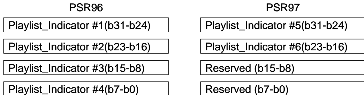
Figure 6-5 Data format of PSR
