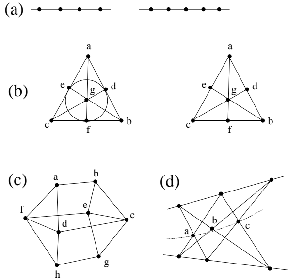
FIGURE 17. Some examples of matroids that are not representable over various fields. (a) The uniform matroids U_{2,4} and U_{2,5} . (b) The Fano and non-Fano matroids, in which def are collinear (resp. non-collinear). (c) The Vámos matroid, in which abcd, abef, cdgh, efgh are coplanar quadruples, but there are no other non-obvious coplanarities. (d) The non-Pappus matroid, in which abc are non-collinear.
