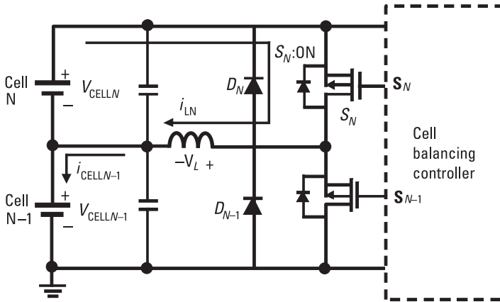
Figure 4.10 Buck-boost converter based cell-balancing circuit implemented in a bq76PL537A active cell-balancing IC.
