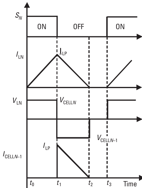
Figure 4.11 Switching waveform of active cell-balancing circuit.
