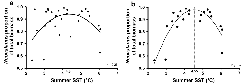
Fig. 5 The proportion of Neocalanus copepods in Least Auklet food loads was related quadratically to summer SST around all three breeding colonies ( a r^2 = 0.25 ), and at Buldir and Kasatochi only ( b r^2 = 0.71 )
