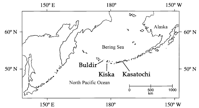
Fig. 1 We studied auklet food loads at Buldir, Kiska, and Kasatochi islands, Aleutian Islands, Alaska, from 1994 to 2006
