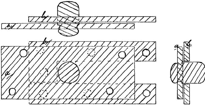
Plan showing mountings for fastening of ribb-stalls. a) A piece of metal whose top (riveted on) is screwed fast to the ribb-stall posts; b) the metal screwed fast to the beam.
