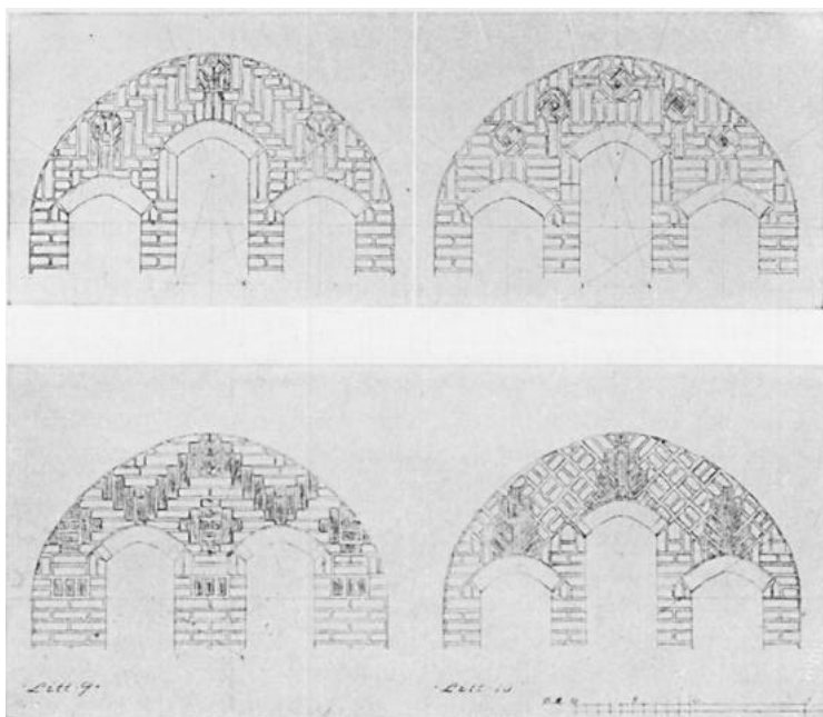
Some of the brickwork patterns.
