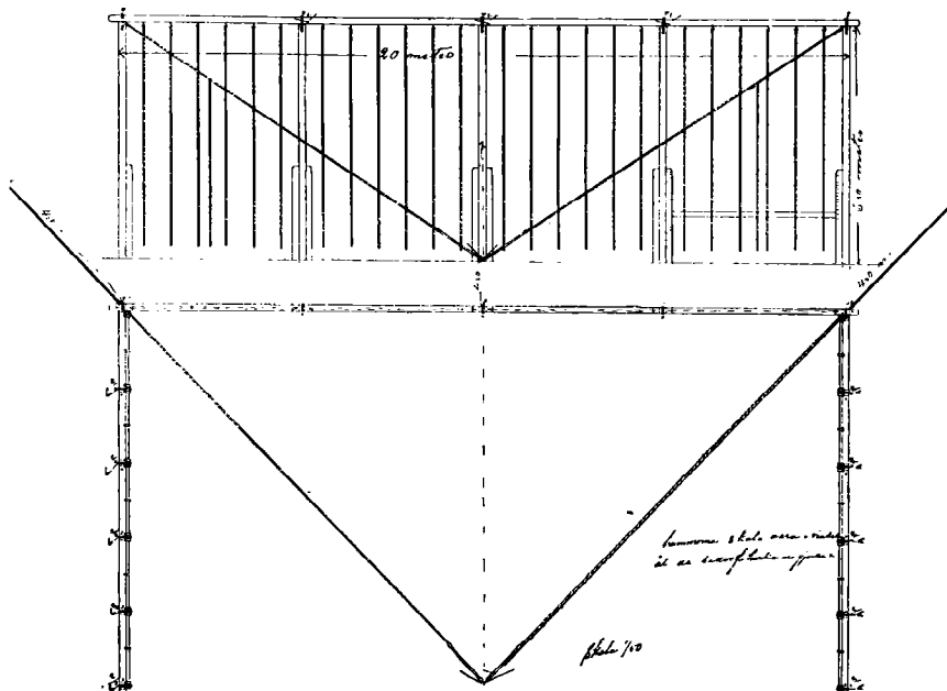
Plan of the removable gymnastic apparatus, with one side turned outwards. Gymnastic apparatus shown: 20 sets ribb-stalls; 4 beams, with double beams and canals for d:o; 2 single inclined ropes with guide ropes: 26 vertical ropes.
