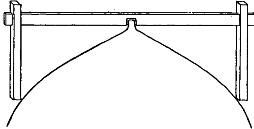
Apparatus for measuring a Four-oared Inrigger.
