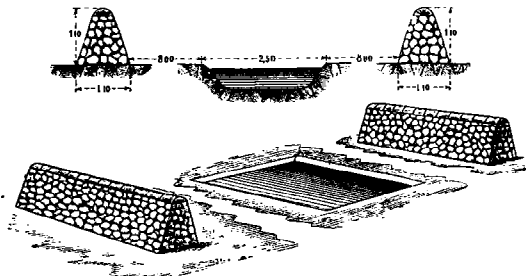
No. 13. Stone-wall—Dike—Stone wall.
