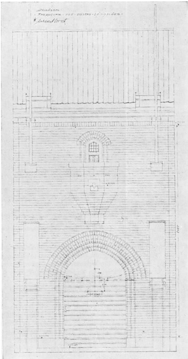
Elevation of one of the side entrances.
