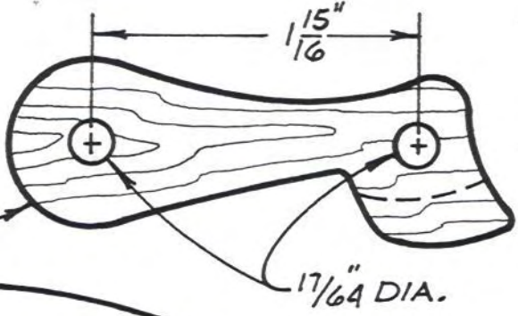
FRONT LEG \frac{1}{2} " THICK (2 REQ'D)
