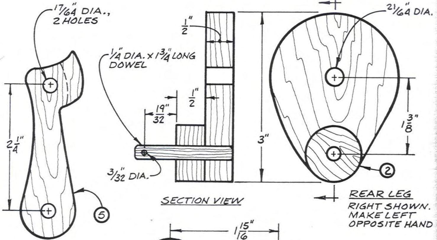
REAR LEG \frac{1}{2} " THICK (2 REQ'D)
