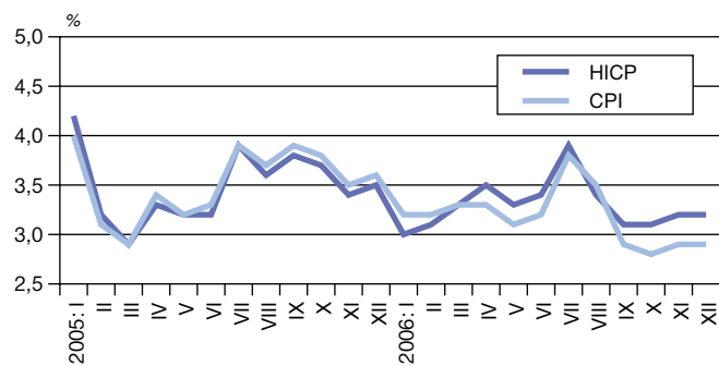
Comparison of the twelve-month rates of change of the HICP and CPI: 2005 and 2006
