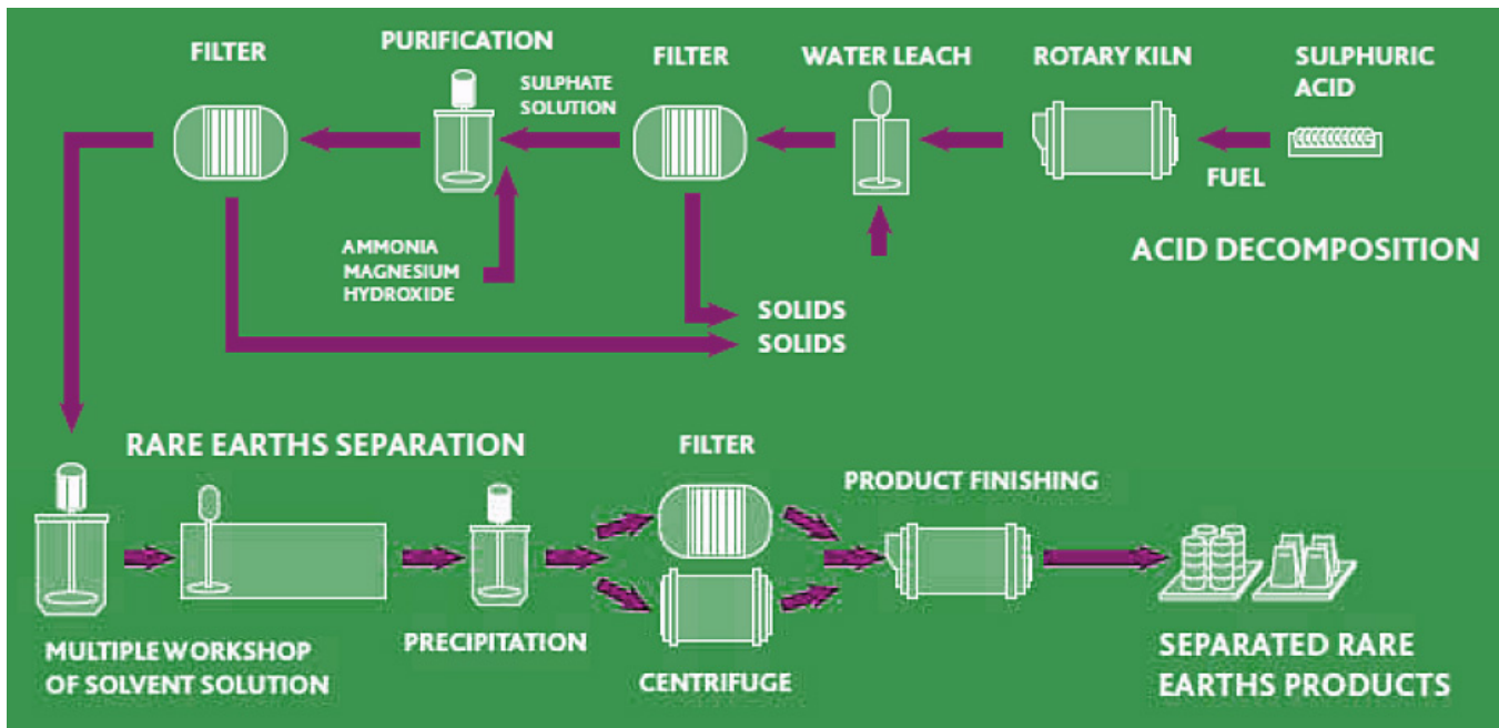
Figure 19. Refining Process of rare earths. Source: Lynas Corporation.
