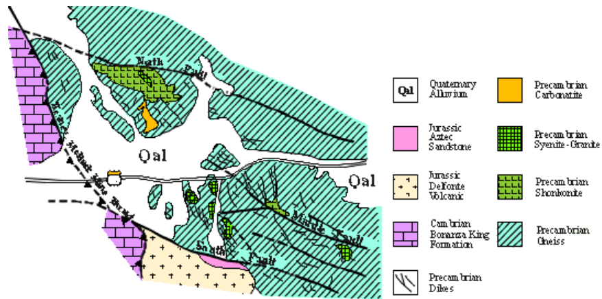
Figure 13. Geological map of the Mountain Pass Deposit.
