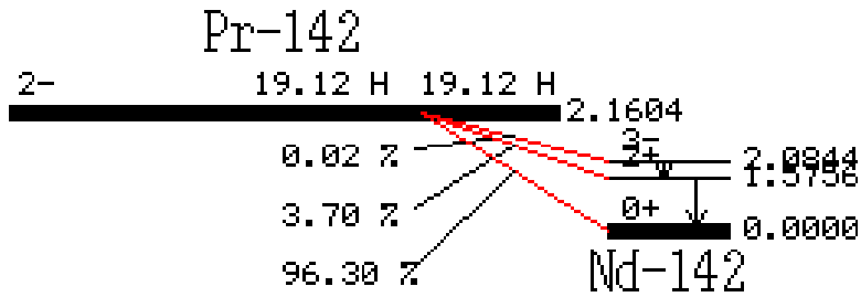
Figure 23. Decay scheme of the _{59}\text{Pr}^{142} radioactive daughter of the _{58}\text{Cerium}^{142} isotope. Gamma photons of 1.5756 MeV and 0.5088 MeV are emitted.
