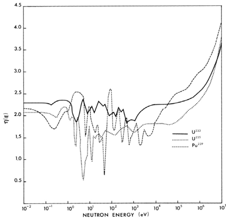
Figure 5. Regeneration factor as a function of neutron energy for the different fissile isotopes.
