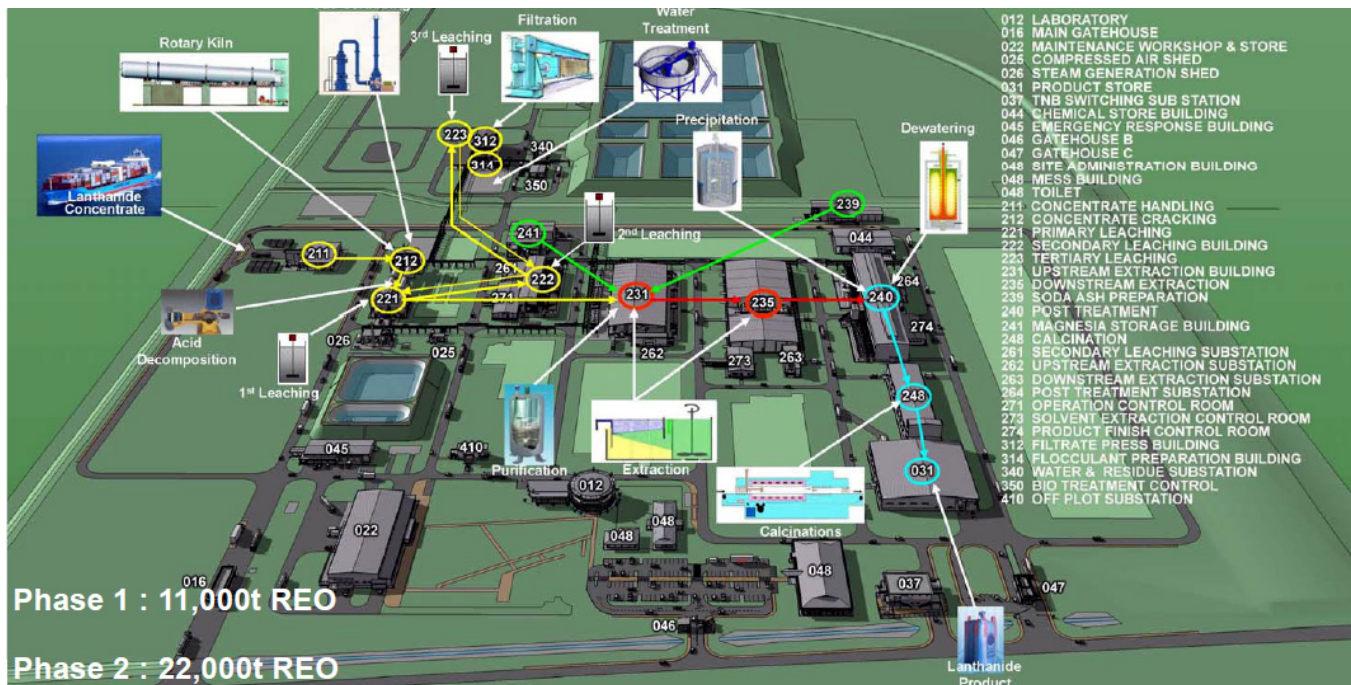
Figure 17 Lynas Advanced Materials Plant, LAMP layout.
