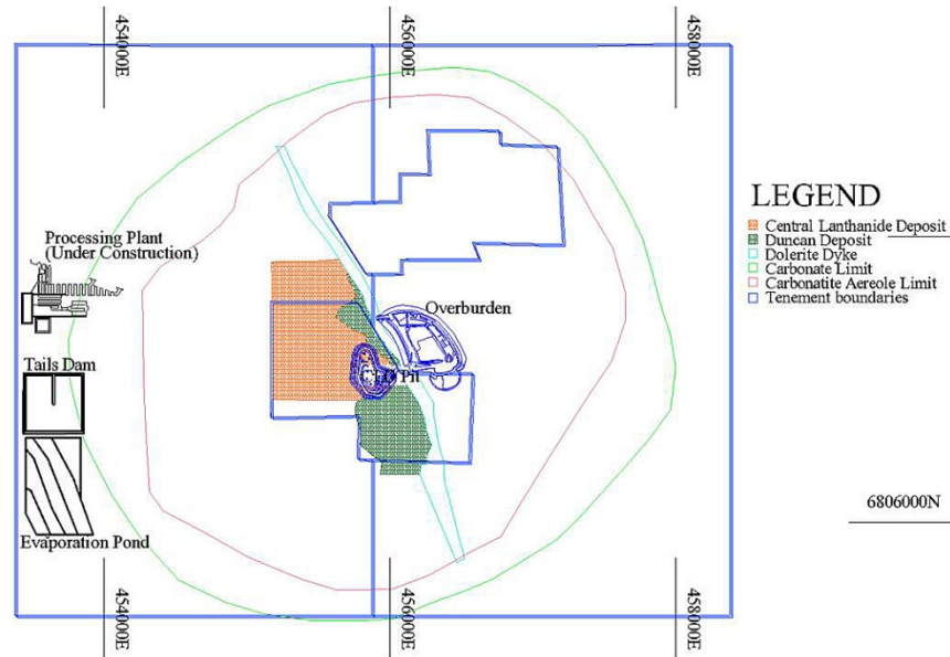
Figure 15. Mount Weld Rare earths deposit, Australia. Source: Lynas Corporation.
