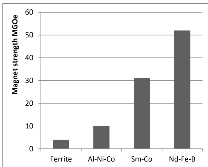
Figure 4. Enhanced field strength in rare earth permanent magnets in Mega Gauss Oersted (MGOe).
