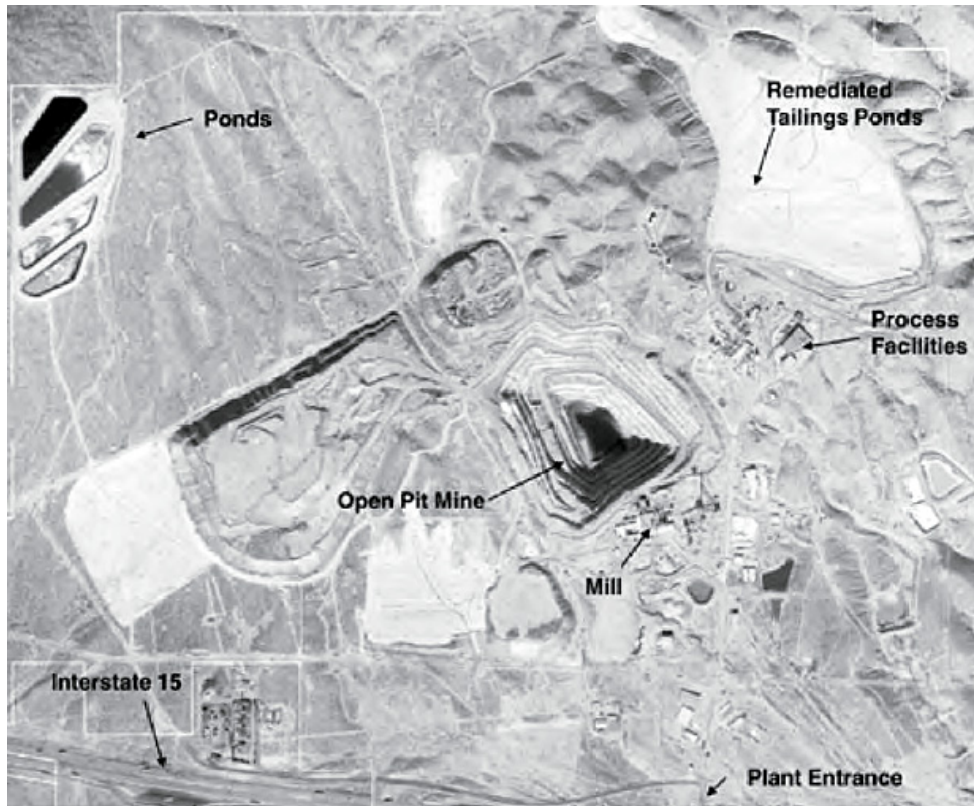
Figure 14. Aerial view of the Mountain Pass deposit, mill and processing plant. Source: Molycorp.
