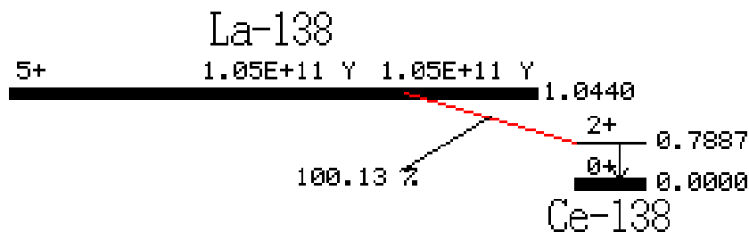
Figure 25. Beta decay of the \text{La}^{138} isotope to the stable \text{Ce}^{138} isotope. It emits a 0.7887 MeV gamma ray photon.
