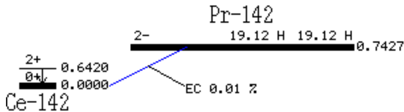
Figure 24. Electron capture in \text{Pr}^{142} into \text{Ce}^{142} . A gamma photon of 0.642 MeV is emitted.
