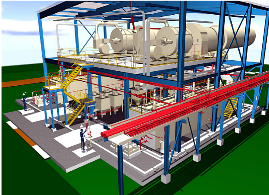
Figure 18. Primary leaching process (221). Source: Lynas Corporation.
