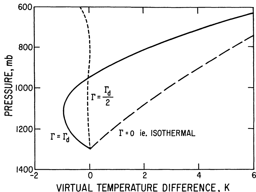
Figure 8 Buoyancy of a methane-saturated parcel versus pressure level, from ST. The buoyancy is positive for a positive virtual temperature difference. The three curves correspond to three different values of the environmental temperature gradient, expressed as a fraction of the dry adiabat \Gamma_D .
