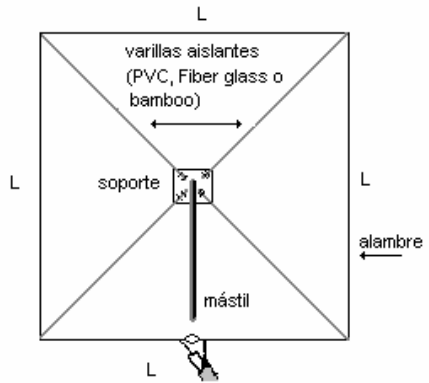
Fig. 32: Antena "Loop"
