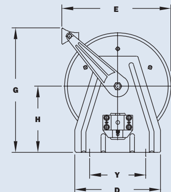
Model HGR50/HGR100/MHGR50 HGR shown
