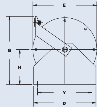
Model GR75/MGR75 GR75 shown
