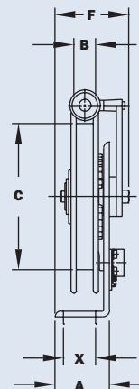
Model HGR50/HGR100/MHGR50 HGR shown
