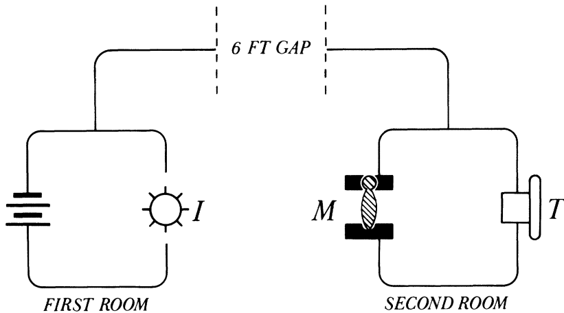
FIGURE 2. The first wireless receiving circuit
