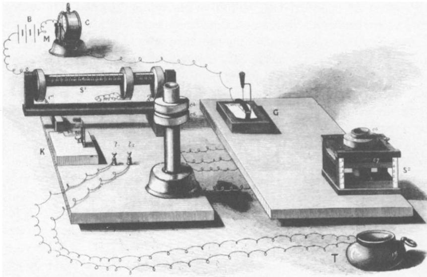
FIGURE 1. The Induction Balance and Sonometer From The Telegraphic Journal , Vol. 7, p. 180, June 1879
