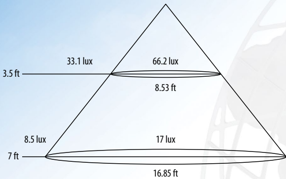
Illuminance (lx)
