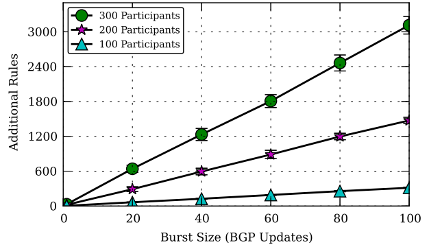
Figure 9: Number of additional forwarding rules.
