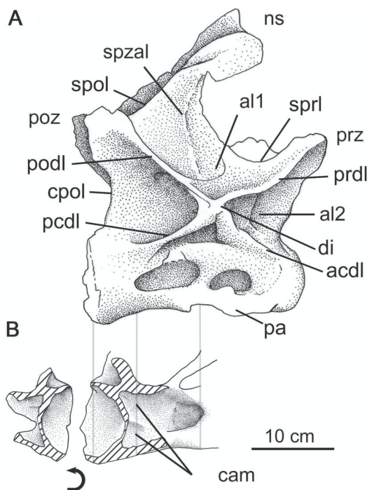
Fig. 2. Cathartesaura anaerobica gen. et sp. nov. Posterior cervical vertebra. A, right lateral view; B, detail of the centrum showing internal cavities. Abbreviations: acdl, anterior centrodiapophyseal lamina; al1, accessory lamina 1; al2, accessory lamina 2; cam, camerae; cpol, centropostzygapophysial lamina; di, diapophysis; ns, neural spine; pa, parapophysis; pcdl, posterior centrodiapophyseal lamina; podl, postzygodiapophysial lamina; poz, postzygapophysis; prdl, prezygodiapophyseal lamina; prz, prezygapophysis; spol, spinopostzygapophysial lamina; sprl, spinoprezygapophysial lamina; spzal, suprapostzygapophysial accessory lamina.
