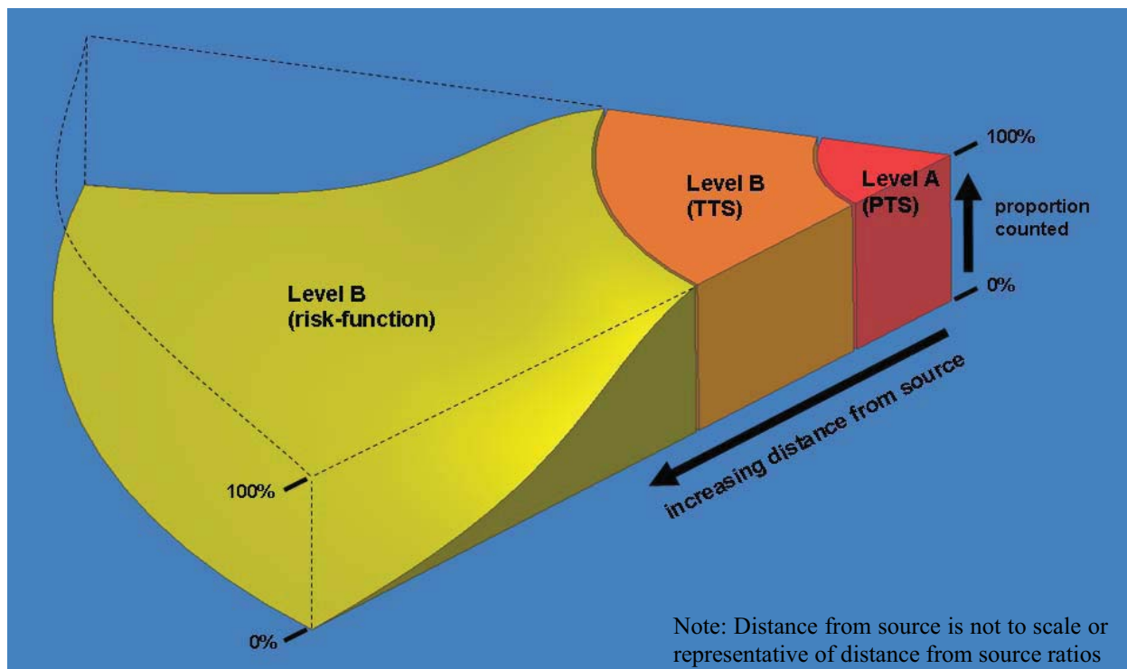
Figure 3.8-5: Exposure Zones Extending from a Hypothetical, Directional Sound Source
