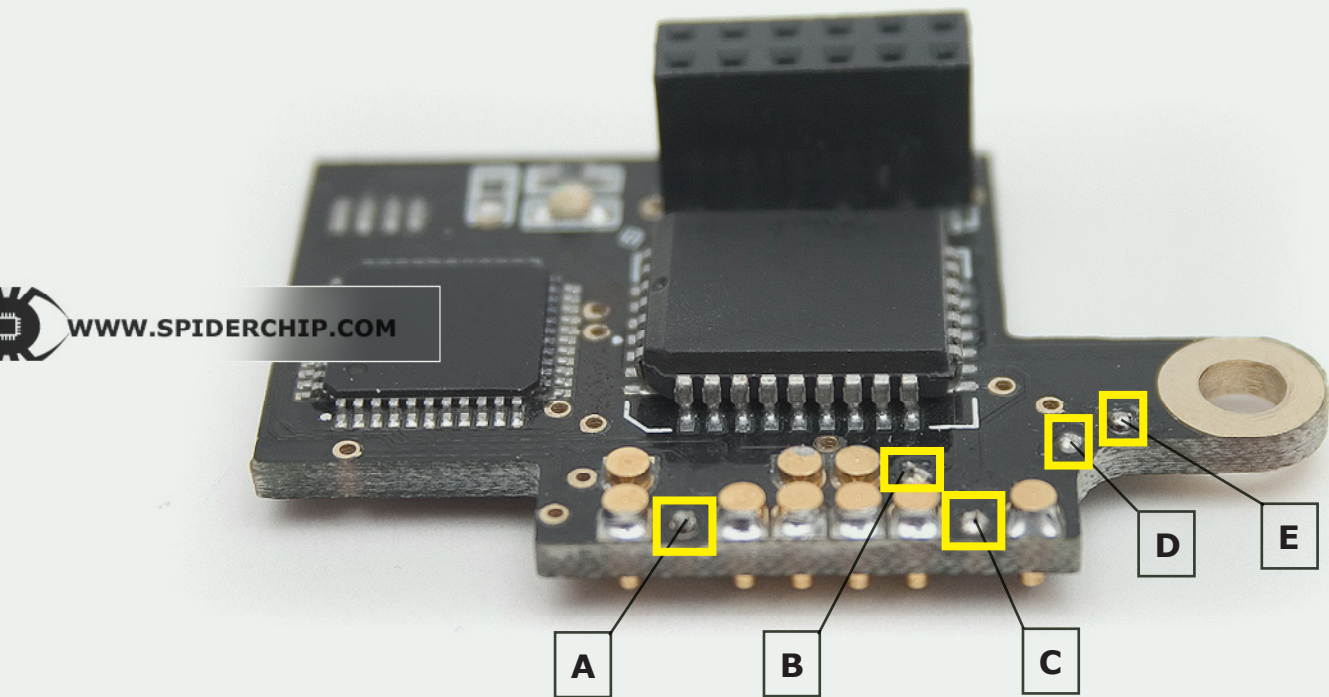
Figure 3. Wire identification on the chip.
