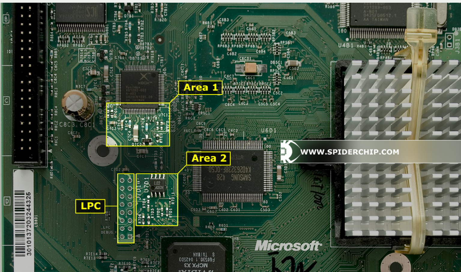
Figure 1. LPC port (16 large holes) and Area 1 & 2 for the wire installation.
