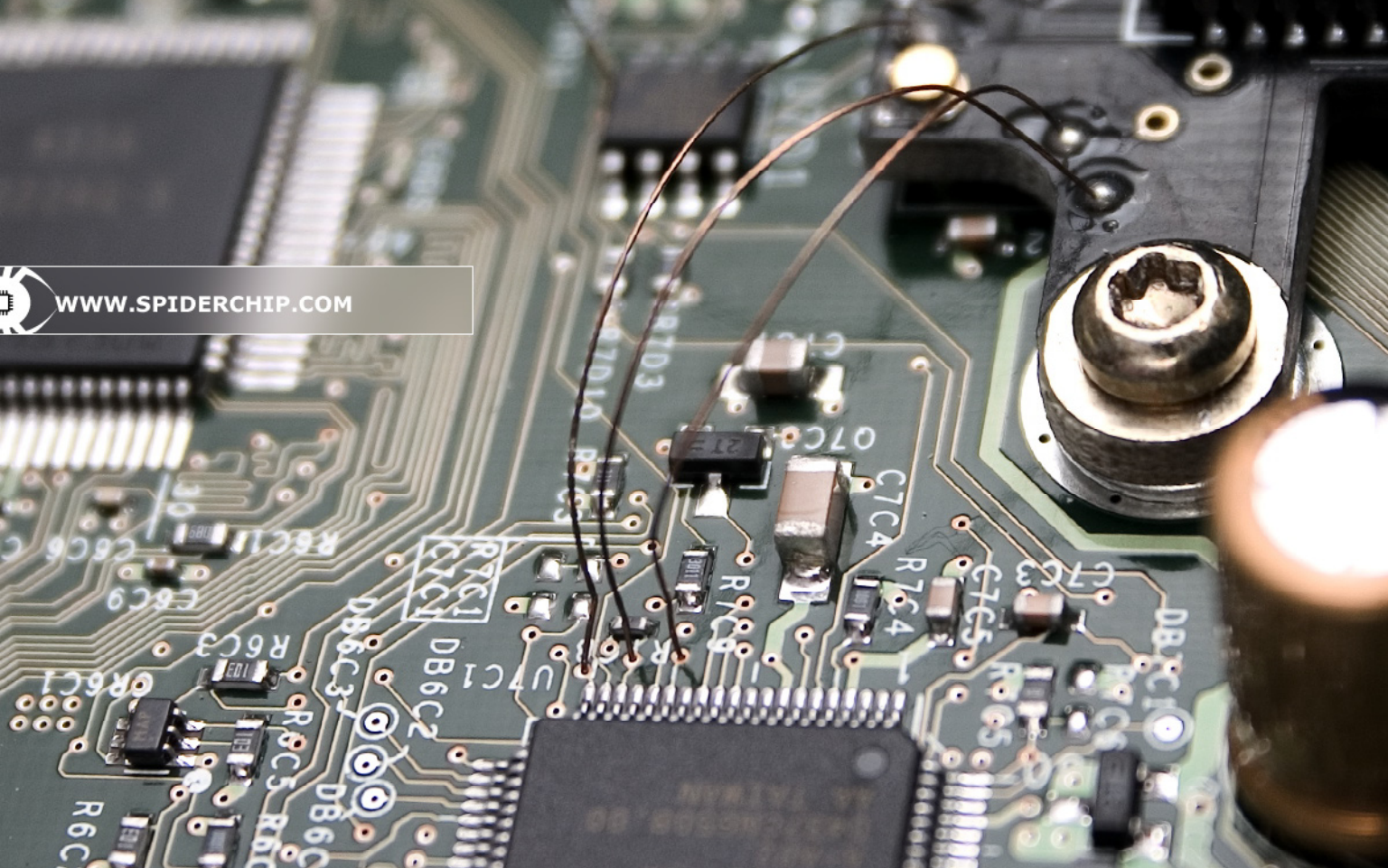
Figure 9. Actual placement of the wires in the Area 2 (Xbox 1.6).
