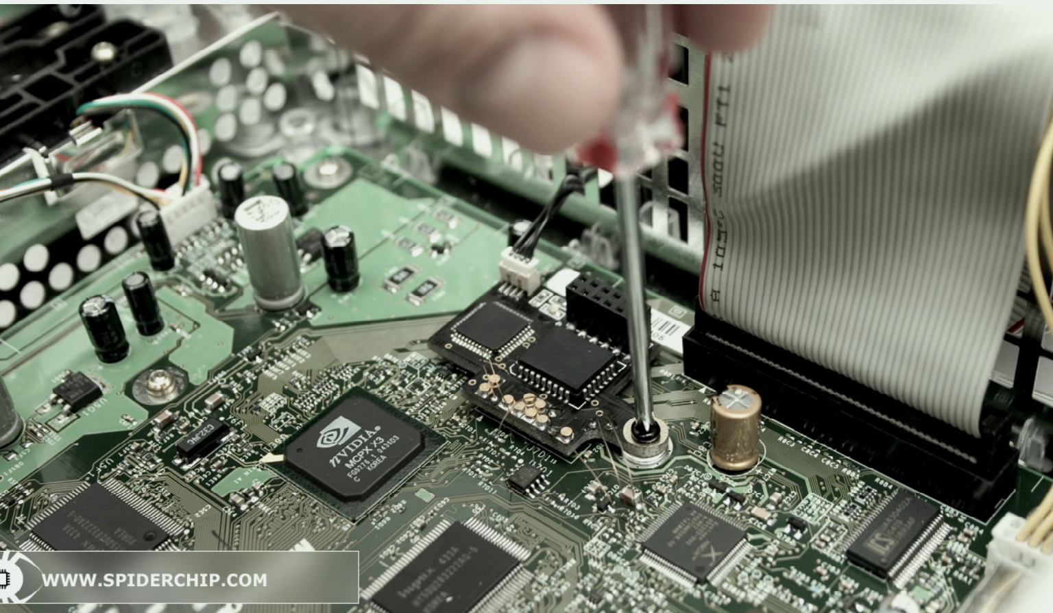
Figure 2. Screwing the chip and alignment on the LPC port.
