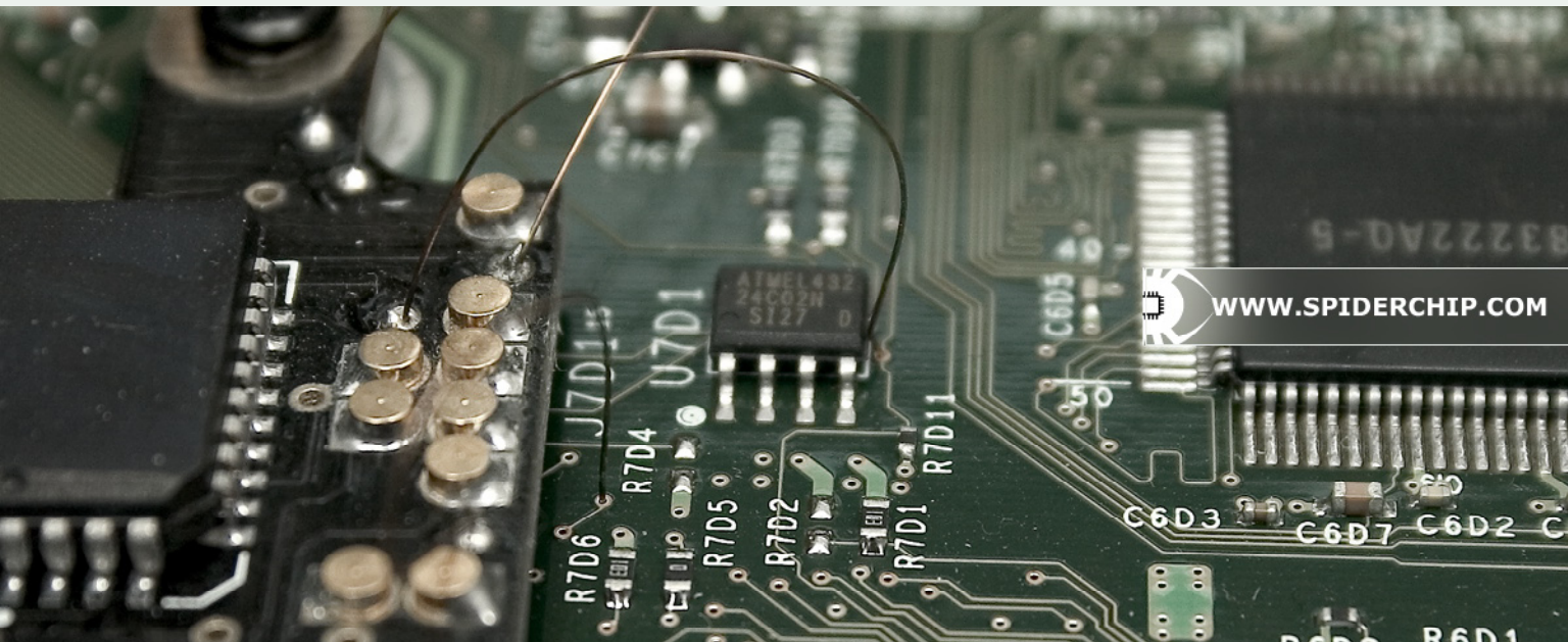
Figure 8. Actual placement of the wires in the Area 1 (Xbox 1.6).
