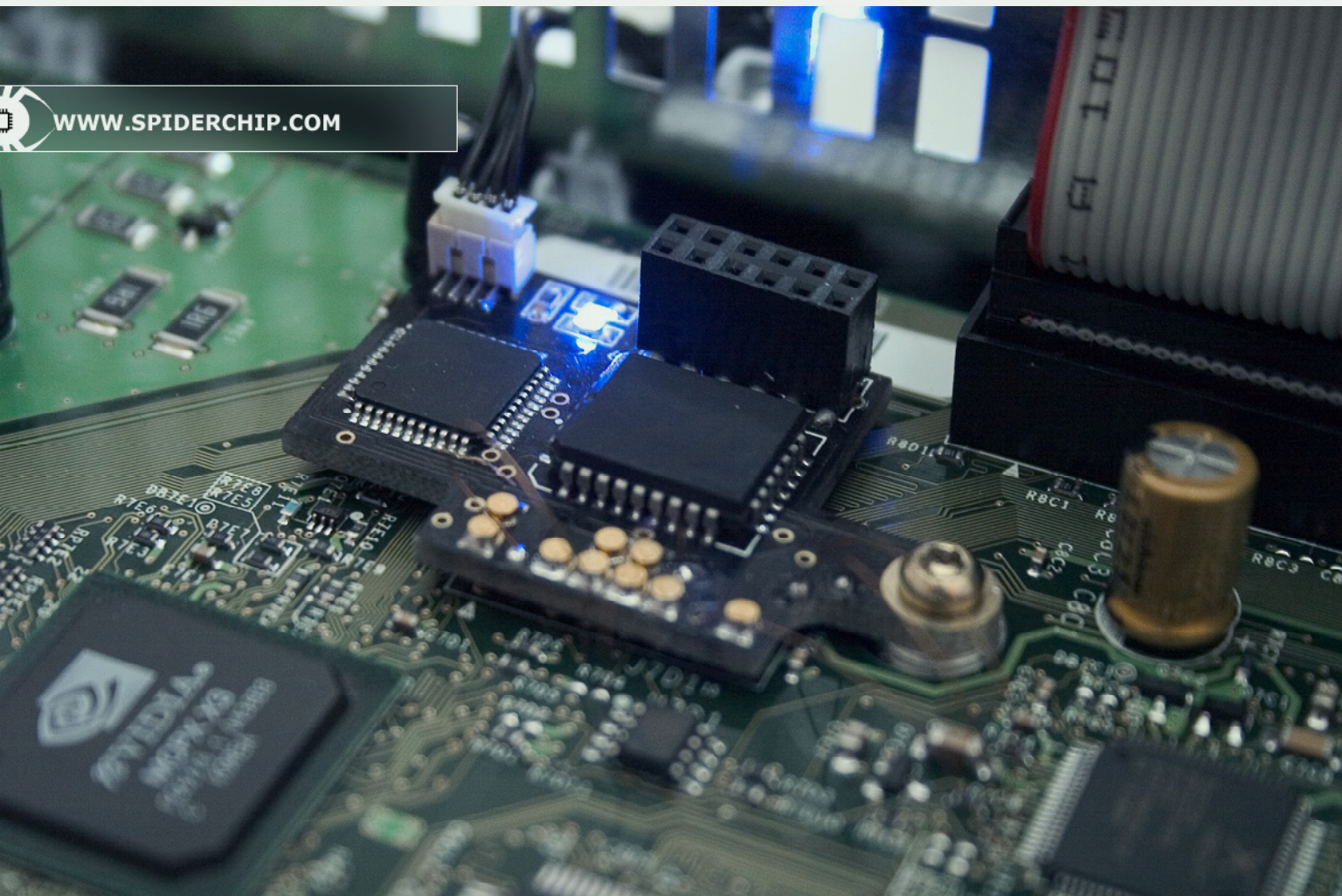
Figure 10. Spider chip blue LED when the Xbox is powered up.
