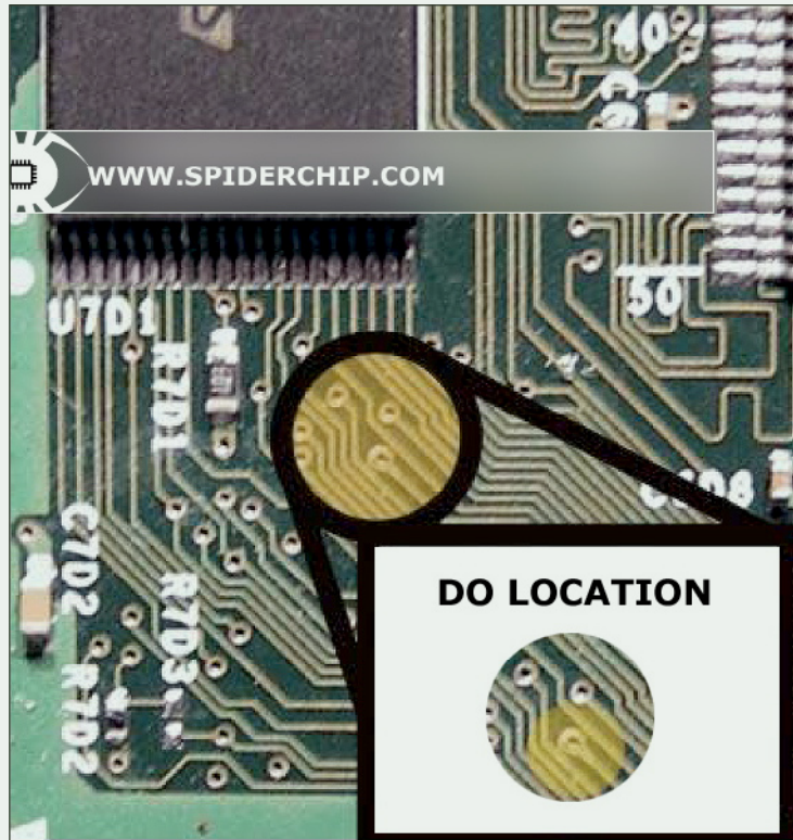
Figure 4. Wire location in Area 2 for Xbox 1.0-1.1.
