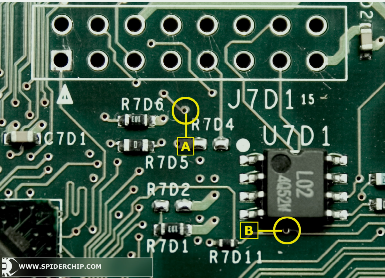
Figure 6. Wire location in Area 1 (Xbox 1.6).
