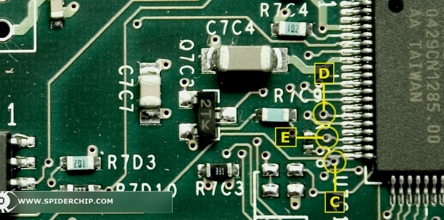
Figure 7. Wire location in Area 2 (Xbox 1.6).
