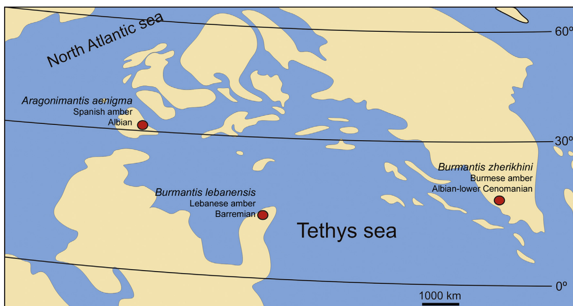
Fig. 1. Palaeogeographic map showing the provenance of the studied specimens (map after Blakey, 2011). In the text there are detailed information from geology of the outcrops, and the fossil record associated to the new taxa.
