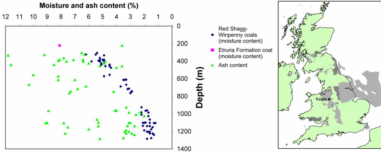
Fig. 13 Moisture and ash content of coals in Keele 1 borehole, showing a general decline in moisture with depth. Different samples of the same seam have moisture content differences of about 1% (Millott et al. 1946). Compare this with other maturity plots (Fig. 9, and of the same borehole Fig. 10).
