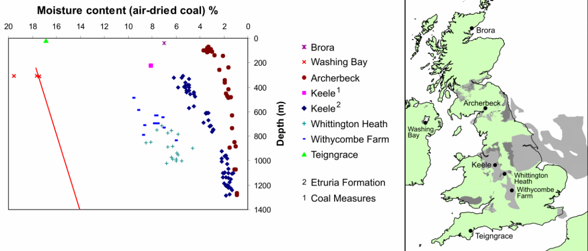
Fig. 14 Plots of moisture content of coals with depth
