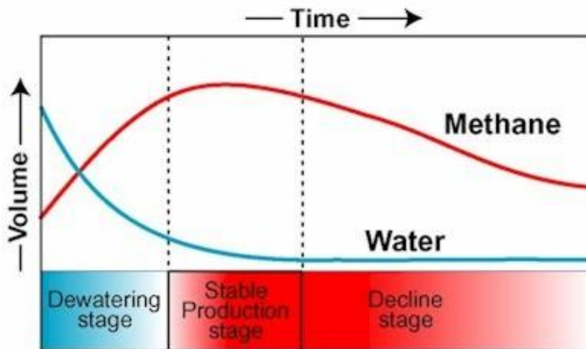
Fig. 21 Typical CBM production profile – derived from http://www.empr.gov.bc.ca /MINING/GEOSCIENCE/COAL/COALBC/CBM/Pages/CBMBrochure.aspx
