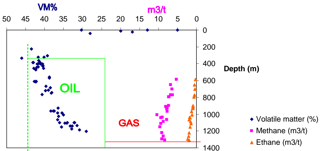
Fig. 10 A plot of volatile matter (VM) in the Keele borehole (Milot et al. 1947) and gas content of coals in the nearby Hobgoblin borehole (data in Creedy 1986). The range of coals analysed in both boreholes is broadly the same. The lowest coal (Winpenny) is 40 m deeper in Keele, whereas the highest coal (Great Row) is 70 m deeper in Hobgoblin. The oil window is defined as in Figure 9. The ethane content in coals rises below a depth of 550 m, indicating that wetter gases are being formed within the lower part of the oil window. Volatile matter values of less than 37% are considered the most favourable for gas generation, corresponding to the values in Cedar Cove CBM field.
