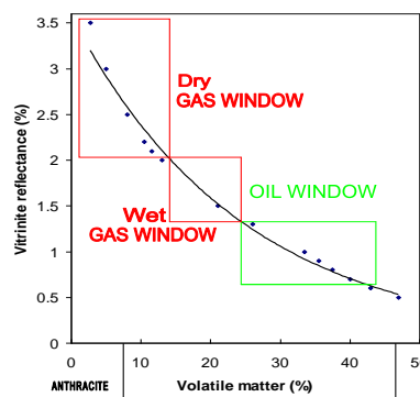
Fig. 9 Hydrocarbon maturity windows and main coal maturity indices. The oil window ranges from 25-43% volatile matter, and the wet gas window ranges from 14-25% volatile matter. The USA Black Warrior Basin CBM fields occur within coals of the Pottsville Formation (Pennsylvanian age) lie in the oil window (Winston 1990).
