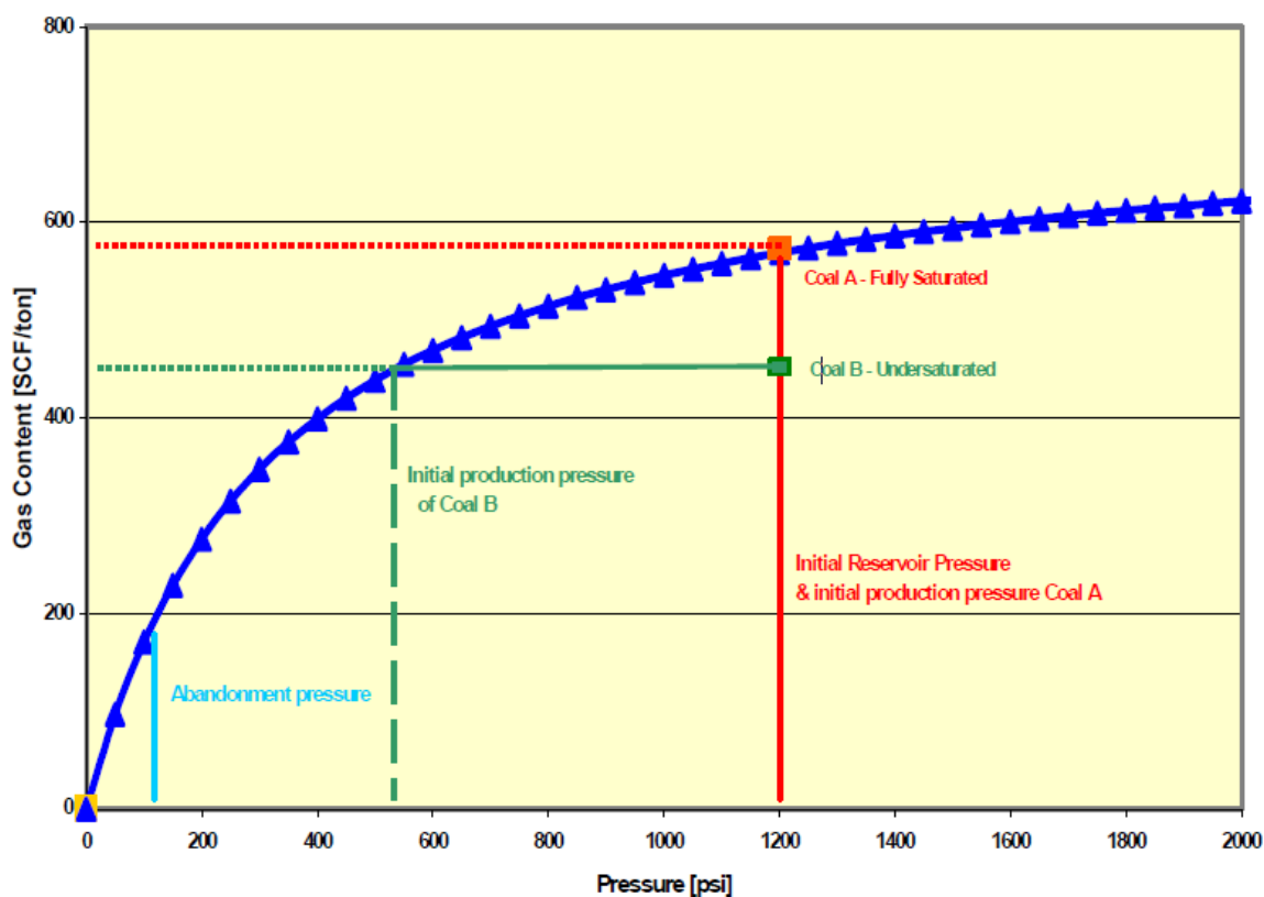
Fig. 22 The relationship of gas content and the adsorption isotherm determines the gas recovery factor
