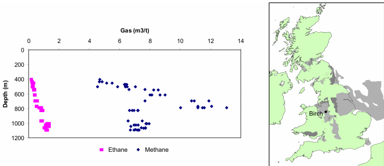
Fig. 5 Methane and ethane content in the Birch borehole, as measured and recorded in the National Coal Board database. Coals below 800 m have lower than expected methane contents (about 4m 3 /t lower), which are partially offset by the more rapid increase in ethane content below this depth.
