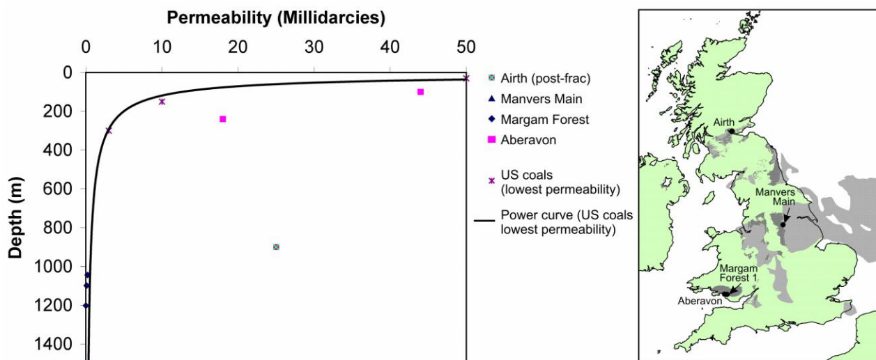
Fig. 16 A plot of UK coal permeability and the lowest permeability values of US coals vs. depth.
