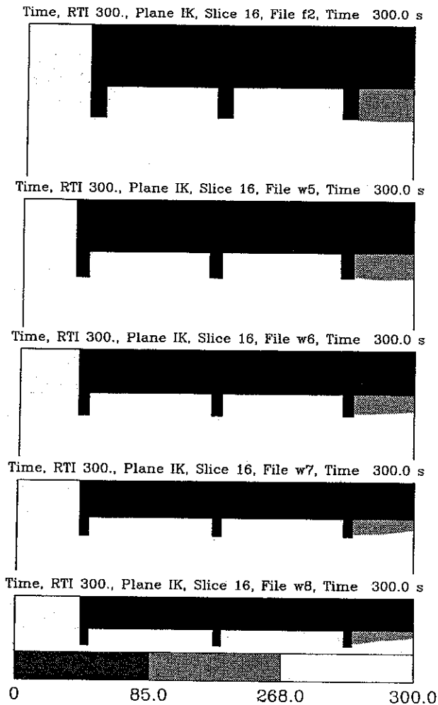
Figure 26: Shaded contour plot of heat detector (RTI = 300) response volumes for various on center beam spacings: 1.2 m (4 ft), 1.5 m (5 ft), 1.8 m (6 ft), 2.1 (7 ft), 2.4 m (8 ft) with 0.305 m (12 in) beam depth, 3.35 m (11 ft) ceiling height and medium fire. Dark and light grey denotes where a sensor activates before the fire reaches 100 kW and 1.0 MW respectively. White denotes where the sensor would not activate. Activation criteria: when the link temperature rises to 57^{\circ}\text{C} ( 135^{\circ}\text{F} ).
