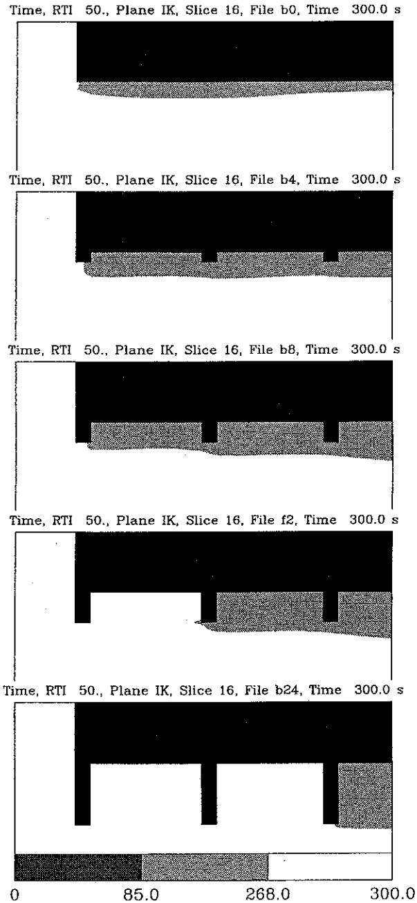
Figure 20: Shaded contour plot of heat detector (RTI = 50) response volumes for various beam depths: 0.0 m (0 in), 0.10 m (4 in), 0.20 m (8 in), 0.30 m (12 in), 0.61 m (24 in) with 3.35 m (11 ft) ceiling height, 1.22 m (4 ft) beam spacing and medium fire. Dark and light grey denotes where a sensor activates before the fire reaches 100 kW and 1.0 MW respectively. White denotes where the sensor would not activate. Activation criteria: when the link temperature rises to 57^{\circ}\text{C} ( 135^{\circ}\text{F} ).
