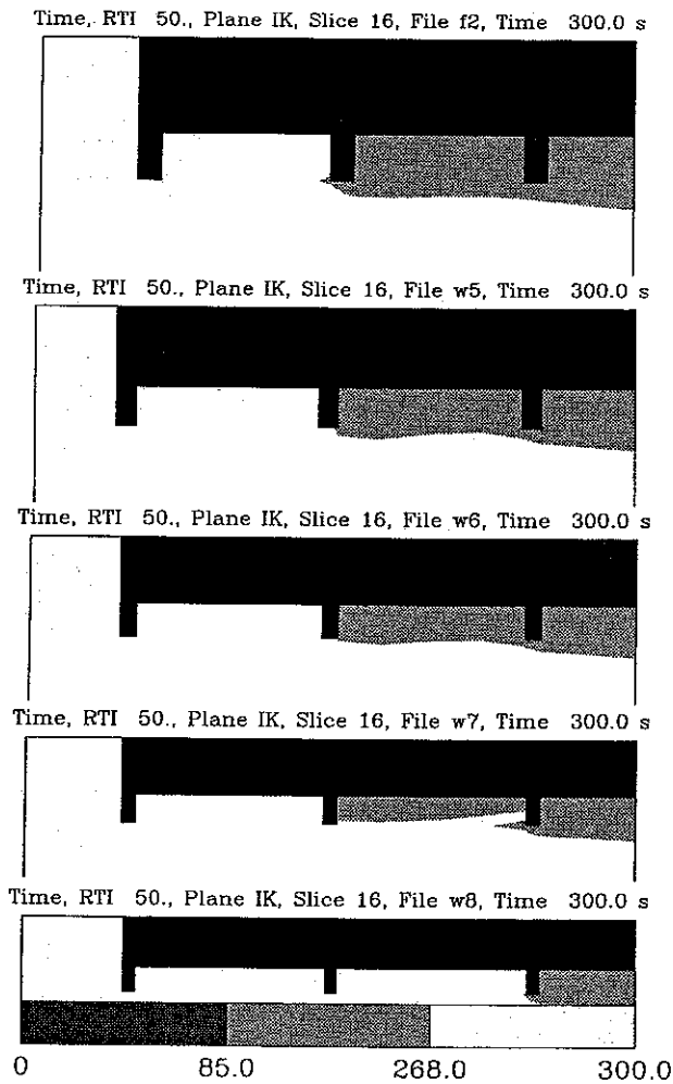
Figure 24: Shaded contour plot of heat detector (RTI = 50) response volumes for various on center beam spacings: 1.2 m (4 ft), 1.5 m (5 ft), 1.8 m (6 ft), 2.1 (7 ft), 2.4 m (8 ft) with 0.305 m (12 in) beam depth, 3.35 m (11 ft) ceiling height and medium fire. Dark and light grey denotes where a sensor activates before the fire reaches 100 kW and 1.0 MW respectively. White denotes where the sensor would not activate. Activation criteria: when the link temperature rises to 57^{\circ}\text{C} ( 135^{\circ}\text{F} ).
