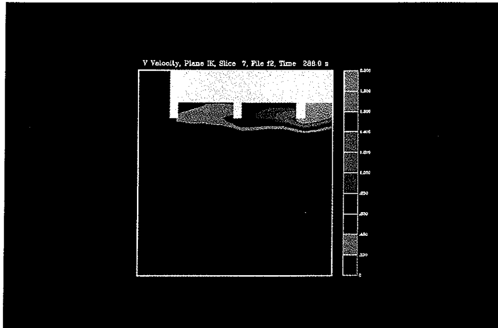
Plate 10. Velocity contours in a plane perpendicular to the floor and the beams for the standard 0.305 m (12 in) beam depth case (F2).
