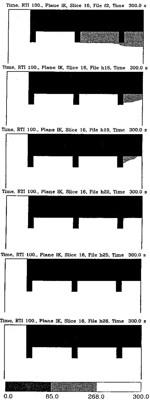
Figure 29: Shaded contour plot of heat detector (RTI = 100) response volumes for various ceiling heights: 3.35 m (11 ft), 4.57 m (15 ft), 5.79 m (19 ft), 6.71 m (22 ft), 7.62 m (25 ft), 8.53 m (28 ft) with 0.305 m (12 in) beam depth, 1.22 m (4 ft) beam spacing and medium fire. Dark and light grey denotes where a sensor activates before the fire reaches 100 kW and 1.0 MW respectively. White denotes where the sensor would not activate. Activation criteria: when the link temperature rises to 57°C (135°F).
