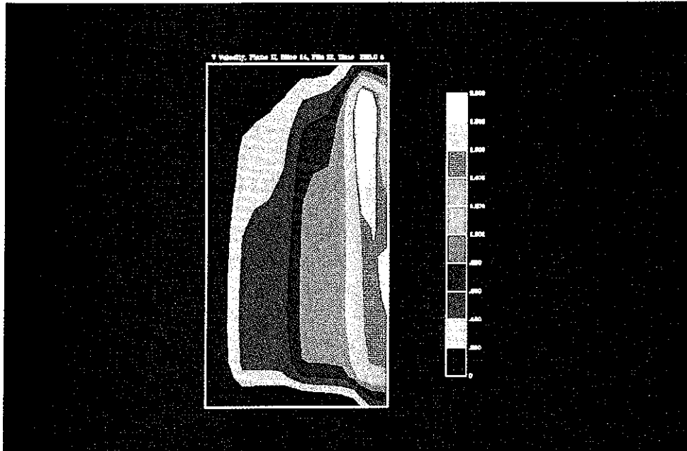
Plate 6. Velocity contours in a plane just below the beams in a 0.305 m (12 in) beamed ceiling (case F2).
