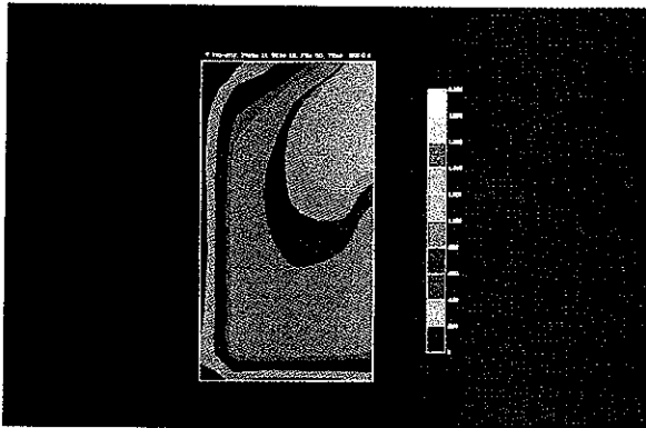
Plate 1. Velocity contours in a plane just below a smooth ceiling (case B0).
