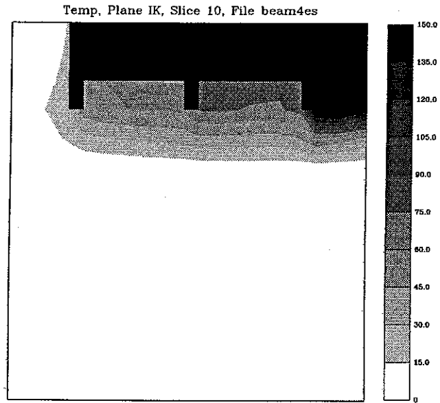
Figure 4: Shaded Temperature Rise Contours ( ^{\circ} C) for Experiment 4 in a Vertical Plane Perpendicular to the Beams 3.05 m (10 ft) from the Fire at 300 seconds
