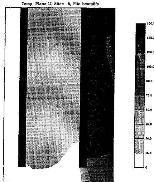
Figure 9: Shaded Temperature Rise Contours (° C) for Experiment 16 in a Plane Parallel and 0.152 m (6 in) Below the Ceiling at 300 seconds
