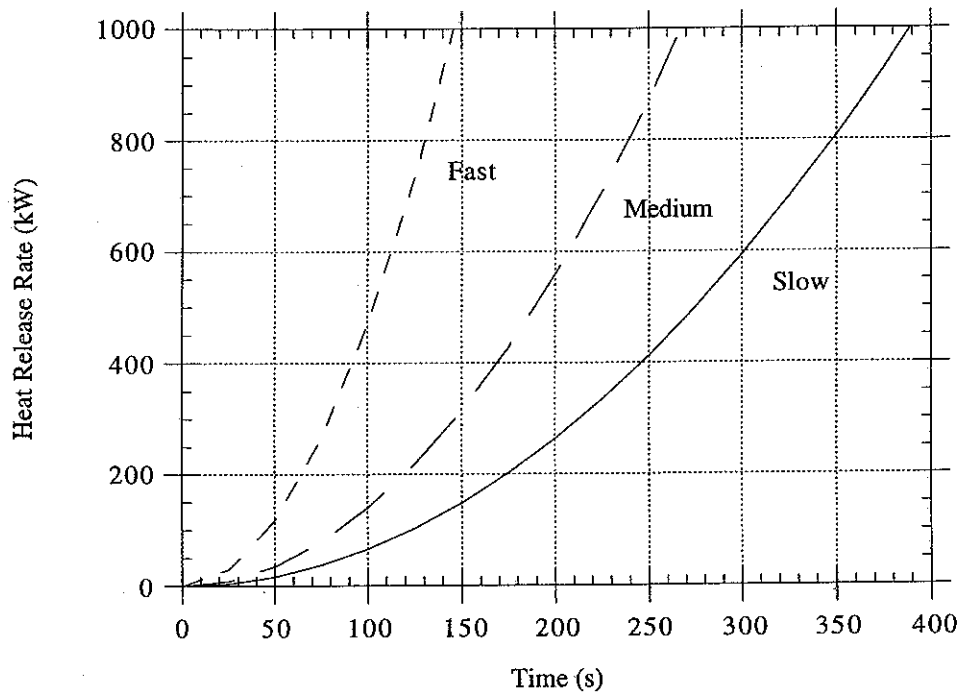
Figure 11: Plot of slow, medium and fast fires versus time
