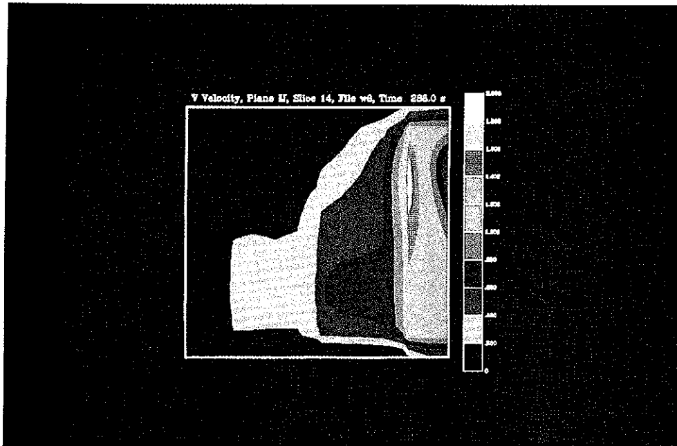
Plate 9. Velocity contours in a plane just below a 0.305 m (12 in), 2.44 m (8 ft) spaced beamed ceiling (case W8).
