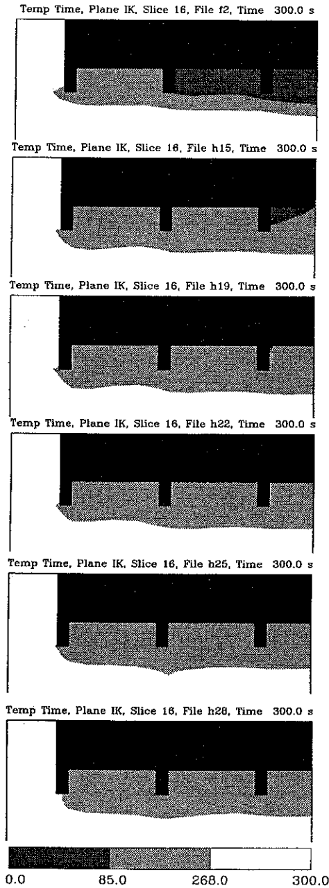
Figure 27: Shaded contour plot of smoke detector response volumes for various ceiling heights: 3.35 m (11 ft), 4.57 m (15 ft), 5.79 m (19 ft), 6.71 m (22 ft), 7.62 m (25 ft), 8.53 m (28 ft) with 0.305 m (12 in) beam depth, 1.22 m (4 ft) beam spacing and medium fire. Dark and light grey denotes where a sensor activates before the fire reaches 100 kW and 1.0 MW respectively. White denotes where the sensor would not activate. Activation criteria: when the gas temperature rises 13^{\circ}\text{C} above ambient.
