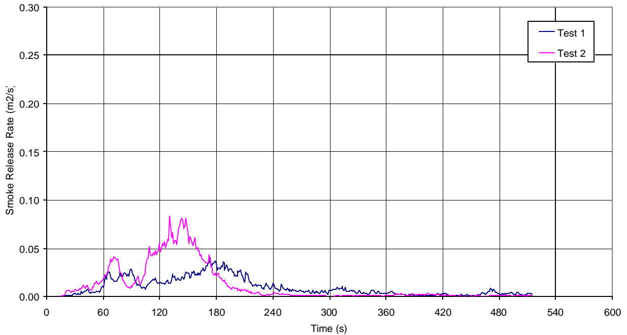
Figure 37 – Heat (top) and smoke (bottom) release for cotton/poly sheet wrapped PU foam
