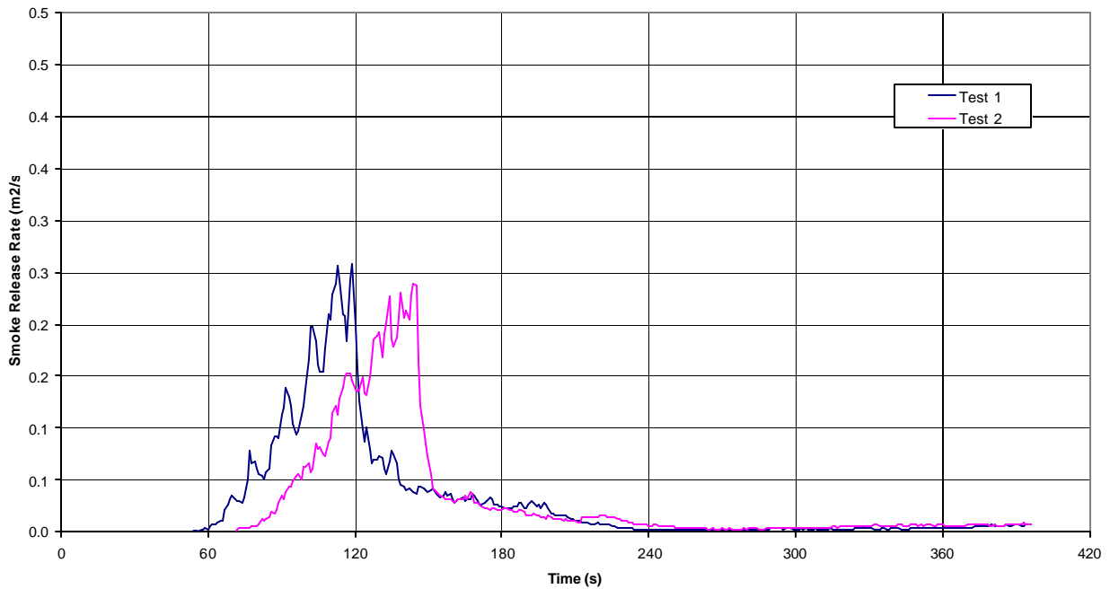
Figure 33 – Heat (top) and smoke (bottom) release rate for Douglas fir
