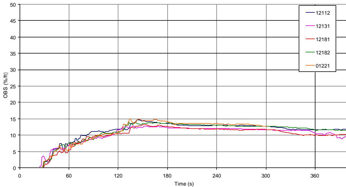
15 Figure 52 – Smoke OBS for heptane/toluene mixture in flaming combustion
