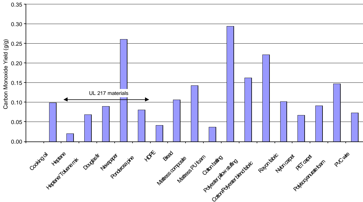
Figure 19 – Carbon monoxide yield for flaming combustion
