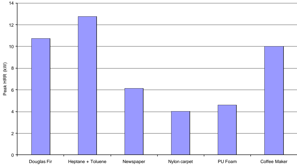
Figure 43 – Peak HRR for flaming combustion tests
