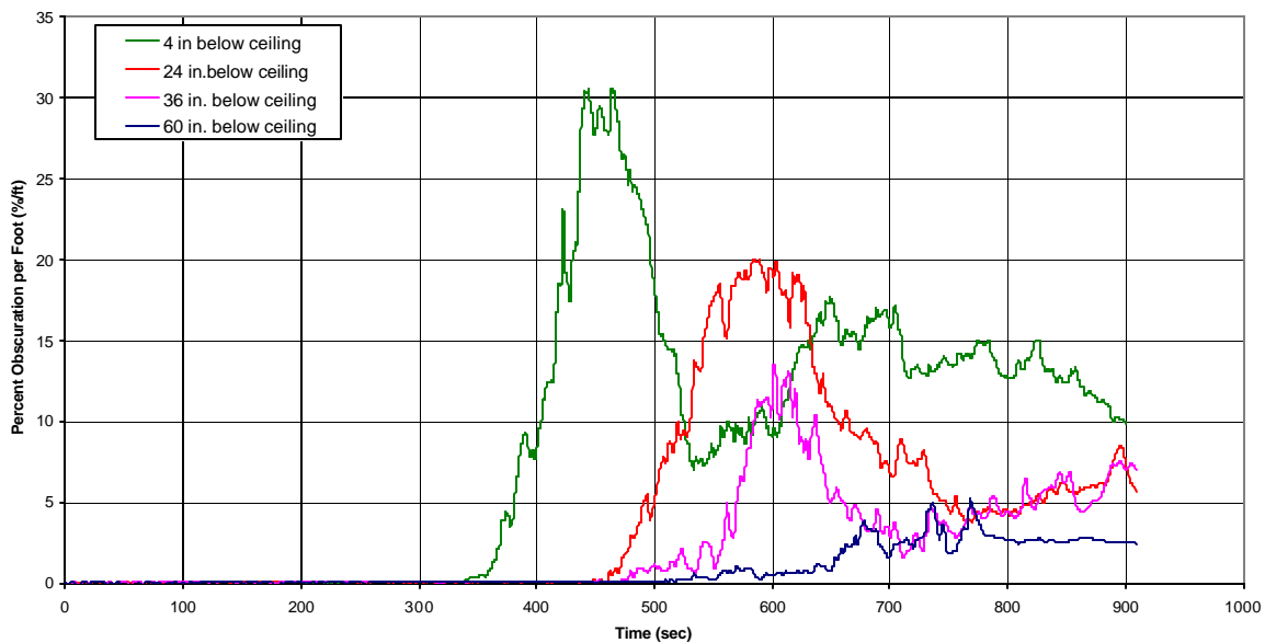
Figure 86 – OBS changes in the test room for bread
