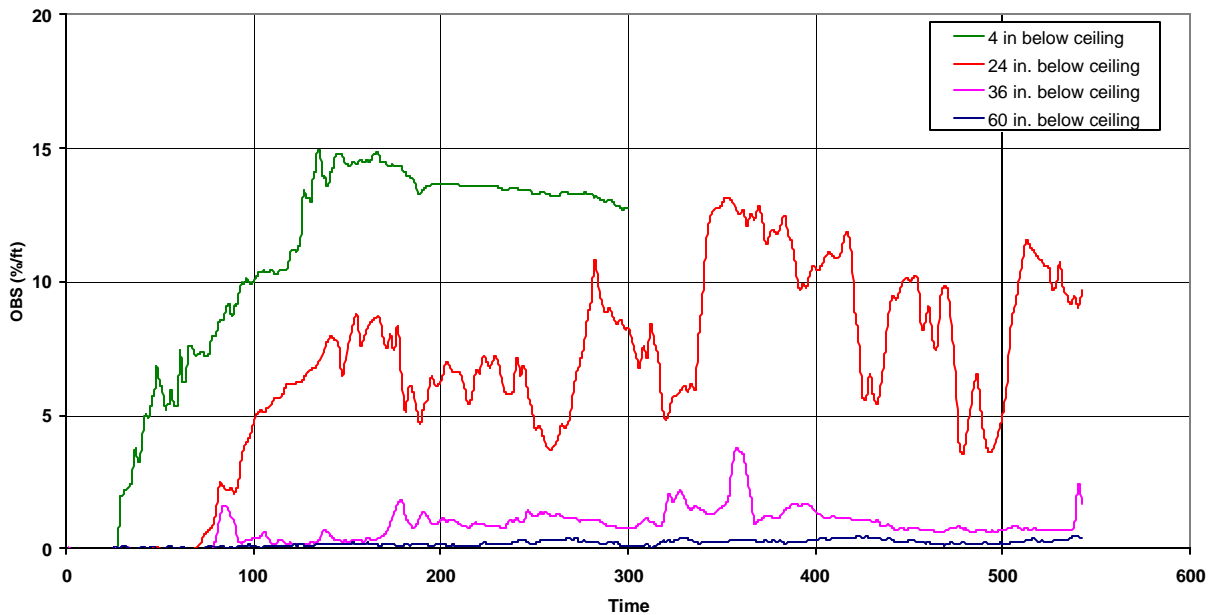
Figure 85 – OBS changes in the test room for heptane/toluene mixture
