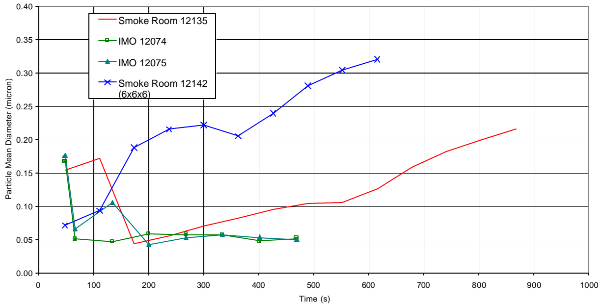
Figure 118 – IMO and Fire Test Room smoke particle mean diameter for flaming PU foam tests
