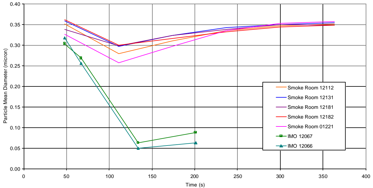
Figure 115 – IMO and Fire Test Room smoke particle mean diameter for flaming heptane/toluene mixture tests
