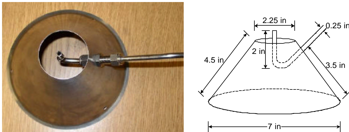
Figure 27 – Intermediate calorimeter evolved smoke and gas sampling cone and tube
