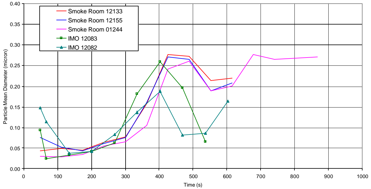
Figure 121 – IMO and Fire Test Room smoke particle mean diameter for non-flaming bread tests
