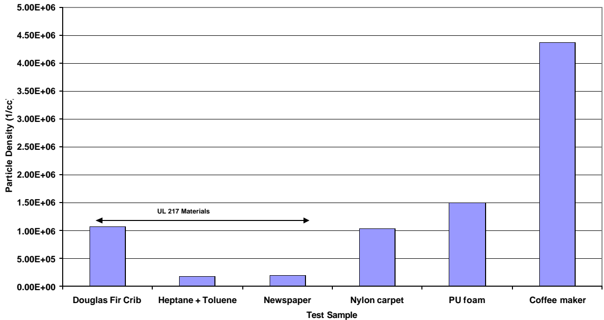
Figure 48 – Average smoke particle density for flaming combustion tests
