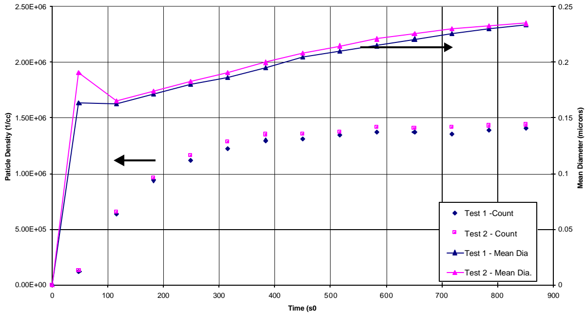
Figure 4 – UL 217 Smoke Box mean smoke particle size diameter for non-flaming cotton wick
