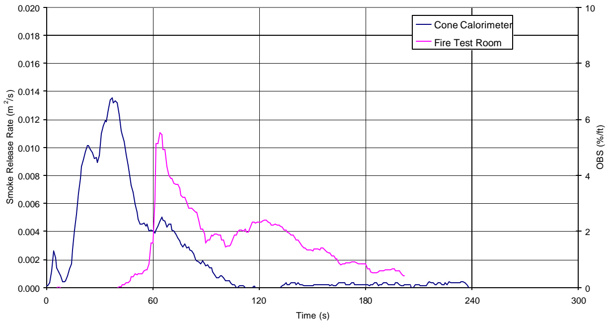
Figure 111 – Small-scale smoke release rate versus Fire Test Room obscuration for flaming PU foam tests
