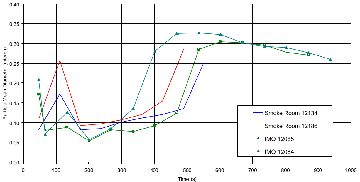
Figure 119 – IMO and Fire Test Room smoke particle mean diameter for flaming coffee maker tests
