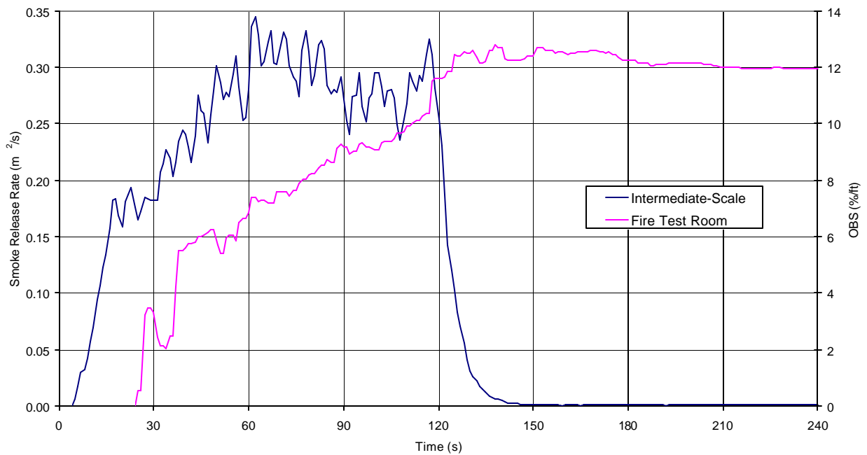
Figure 112 – Intermediate-scale smoke release rate versus Fire Test Room obscuration for flaming heptane/toluene mixture tests
