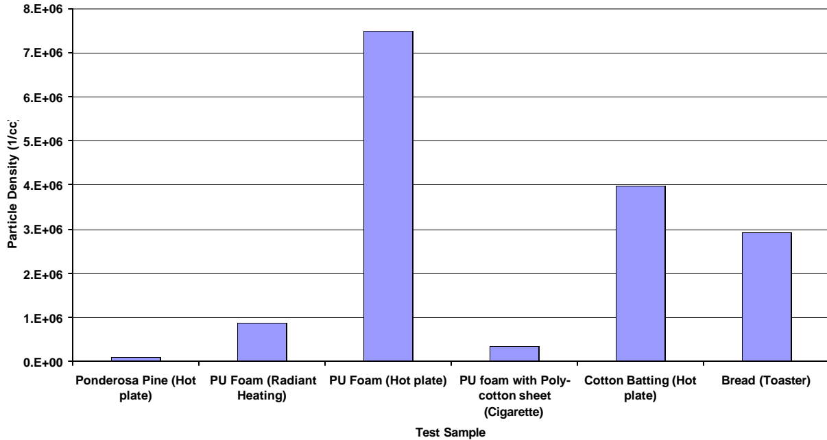
Figure 50 – Average particle count for non-flaming combustion tests
