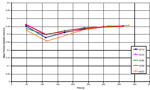
Figure 66 – Mean smoke particle diameter and count for flaming heptane/toluene tests
