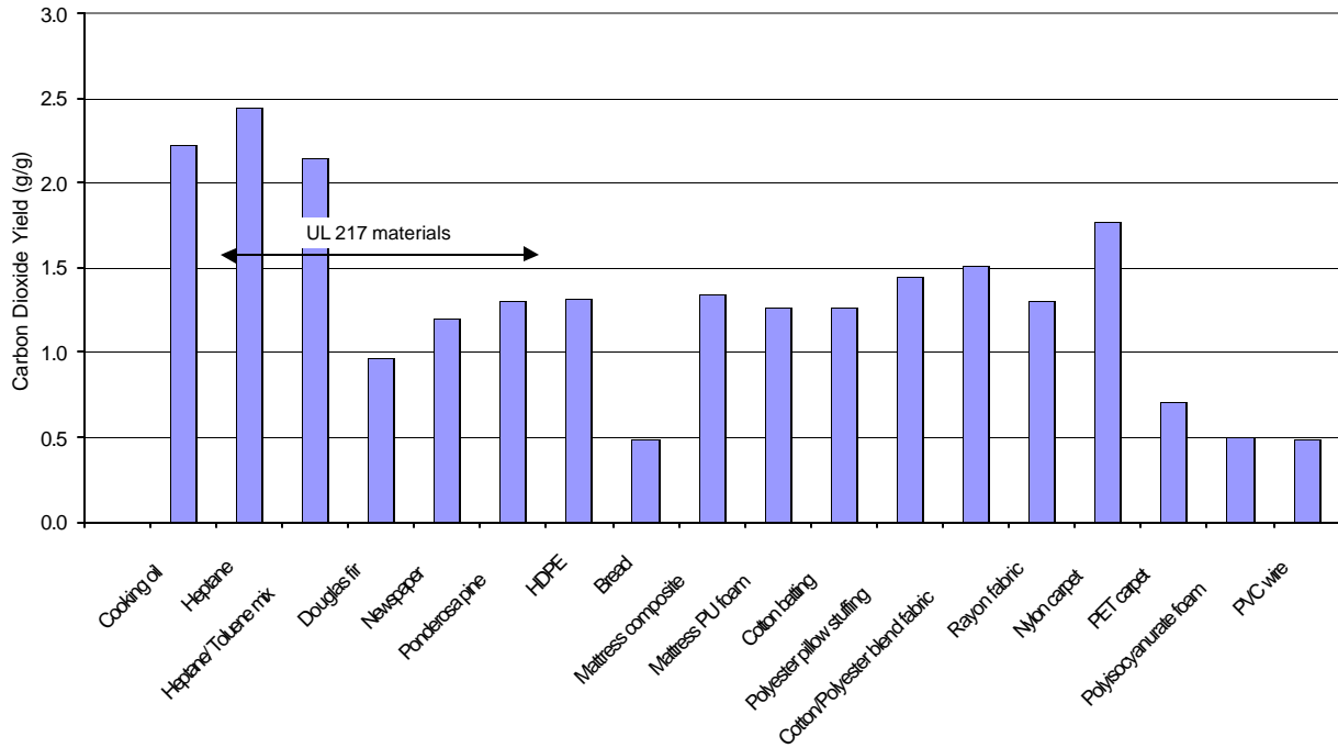
Figure 18 – Carbon dioxide yield for flaming combustion
