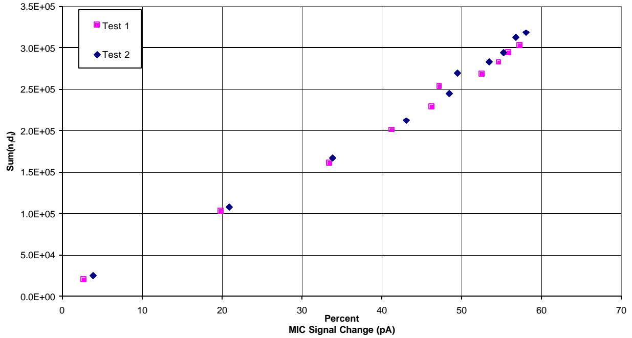
Figure 7 – Relationship between the MIC signal and particle density in the UL 217 Smoke Box for non-flaming cotton wick
