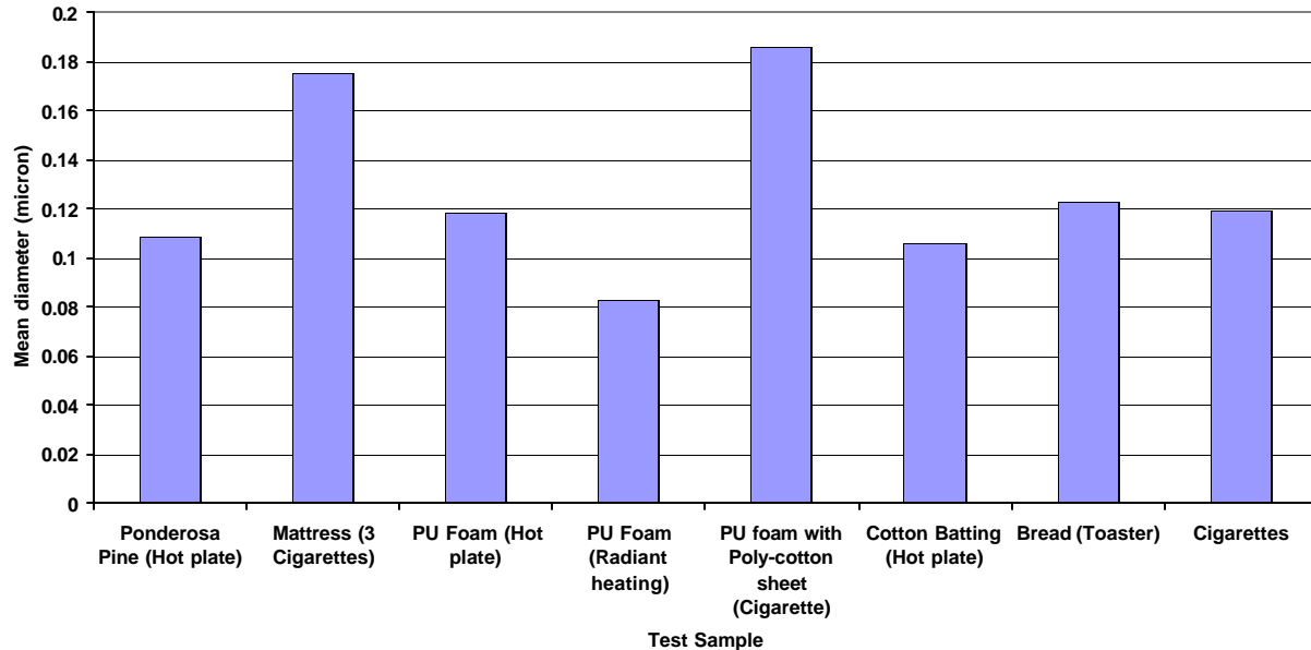
Figure 49 – Mean smoke particle diameter for non-flaming tests
