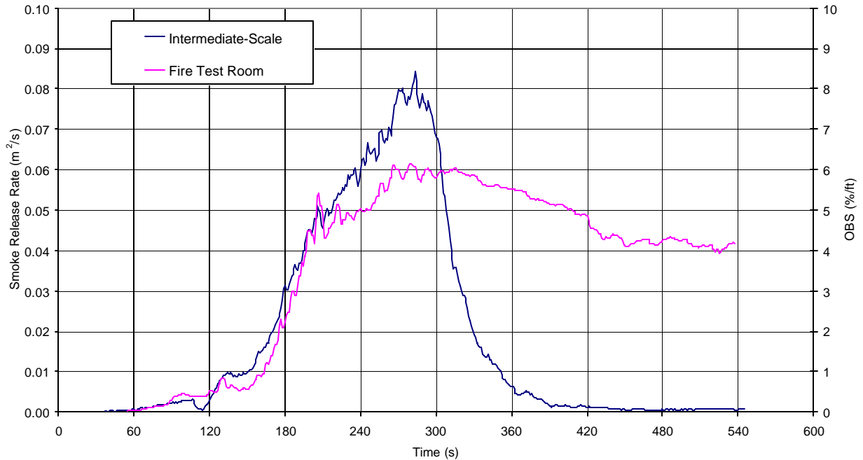
Figure 113 – Intermediate-scale smoke release rate versus Fire Test Room obscuration for flaming nylon carpet tests
