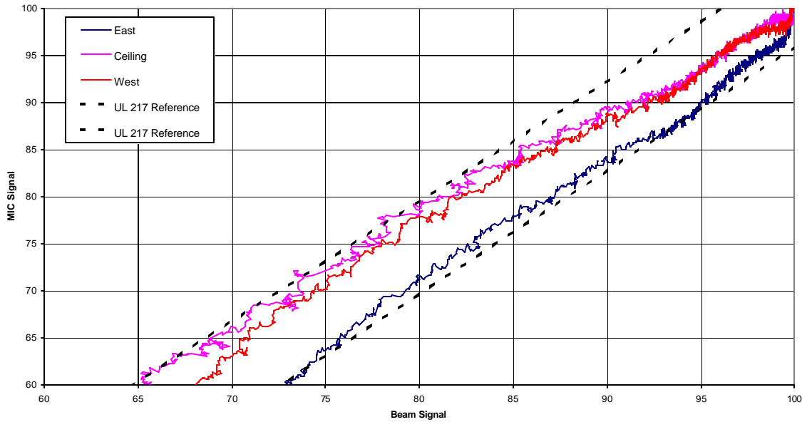
10 Figure 80 – Beam vs. MIC response: Ponderosa pine
