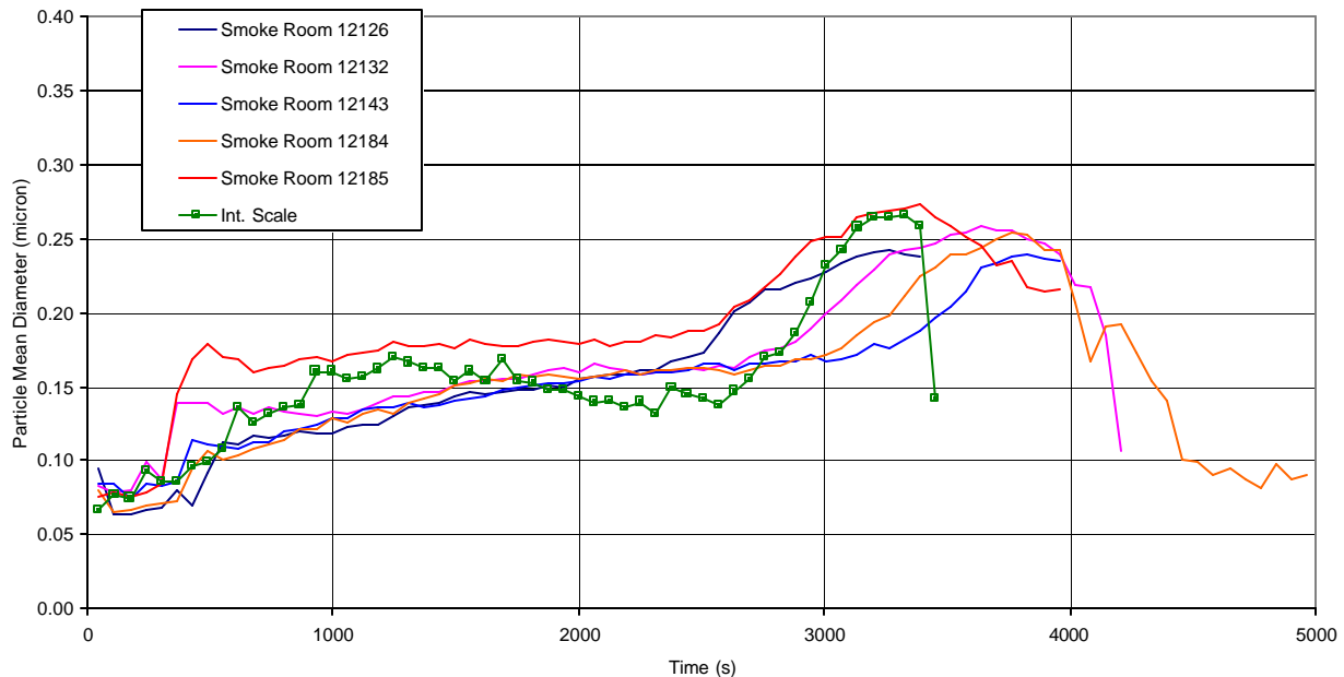
Figure 120 – Intermediate-scale and Fire Test Room smoke particle mean diameter for non-flaming Ponderosa pine tests
