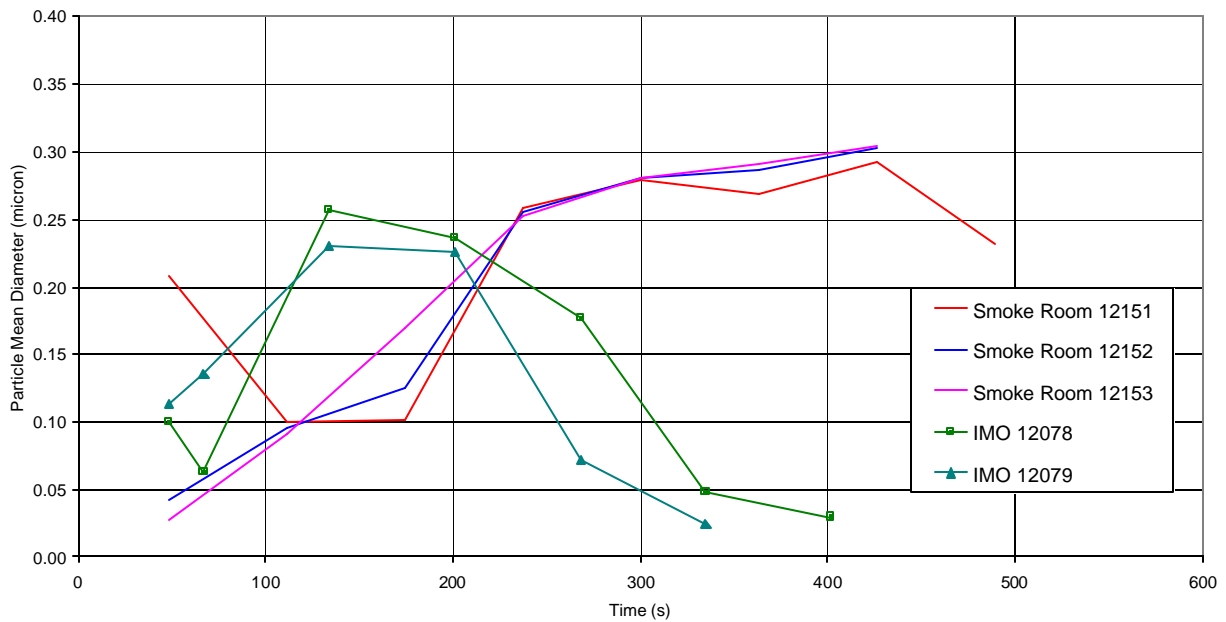
Figure 122 – IMO and Fire Test Room smoke particle mean diameter for flaming nylon carpet tests
