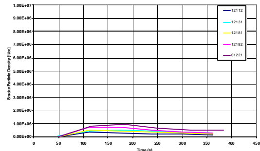
Figure 66 – Mean smoke particle diameter and count for flaming heptane/toluene tests
