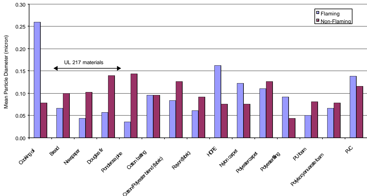
Figure 100 – Mean particle diameter for small-scale flaming and non-flaming combustion
