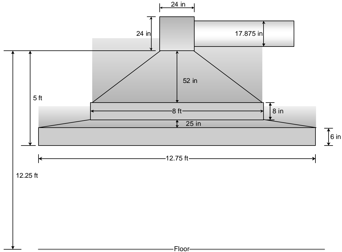
Figure 25 – Schematic of NEBS calorimeter
