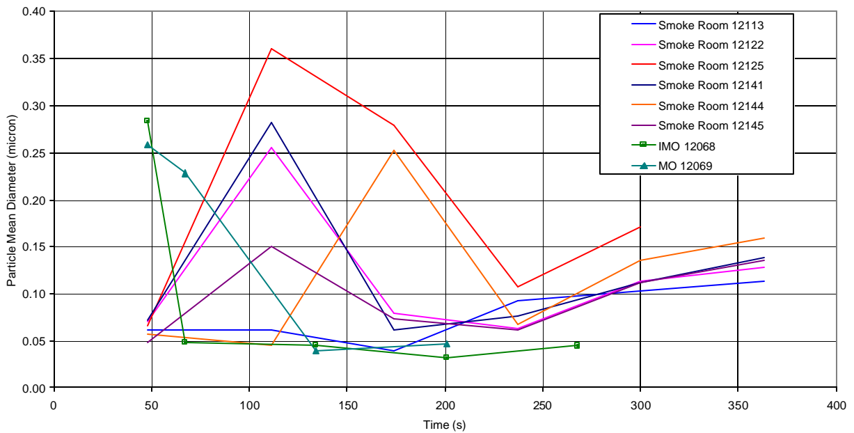
10 Figure 117 – IMO and Fire Test Room smoke particle mean diameter for flaming newspaper tests
