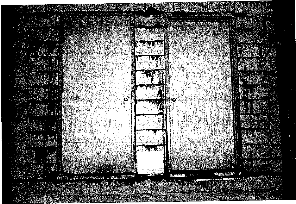
EXPOSED SIDE PRIOR TO FIRE TEST
