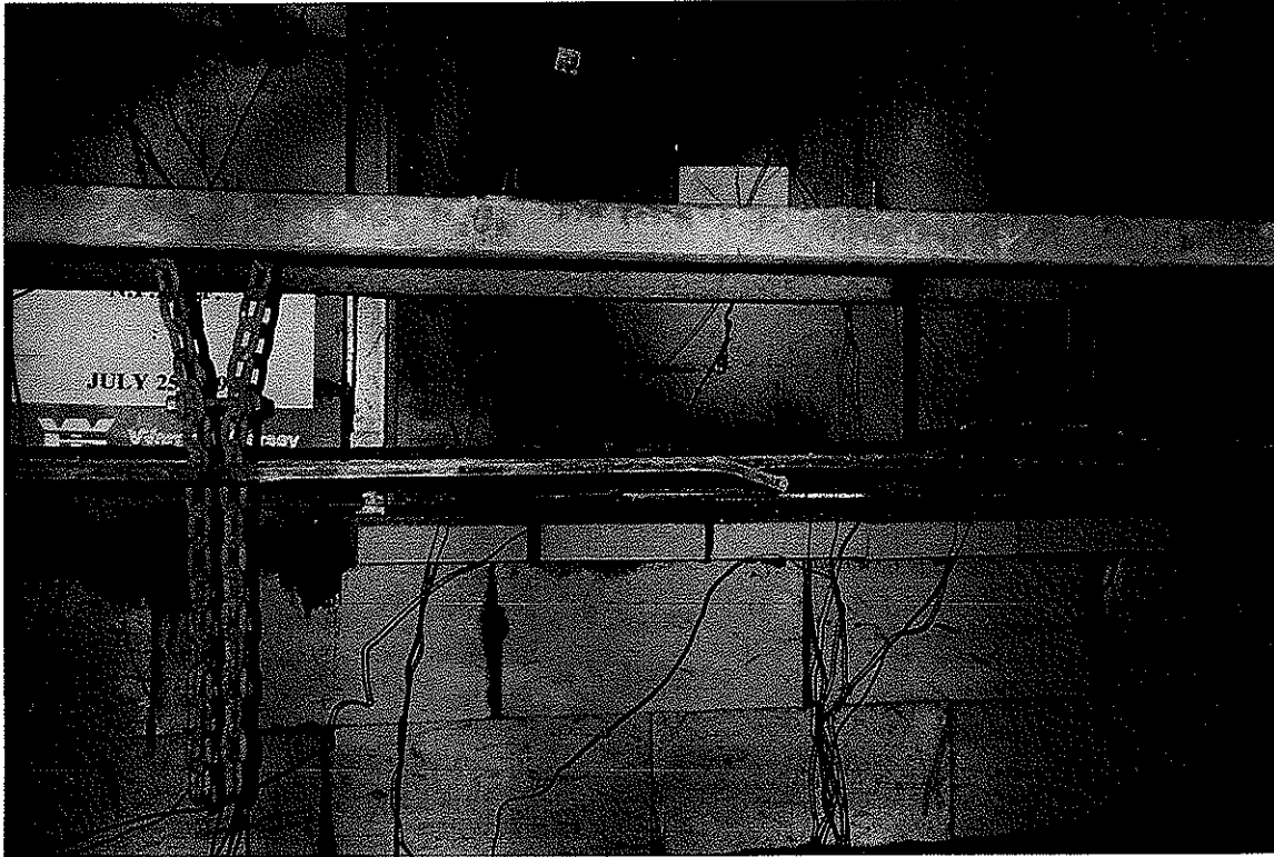
VENTING AT SILL
