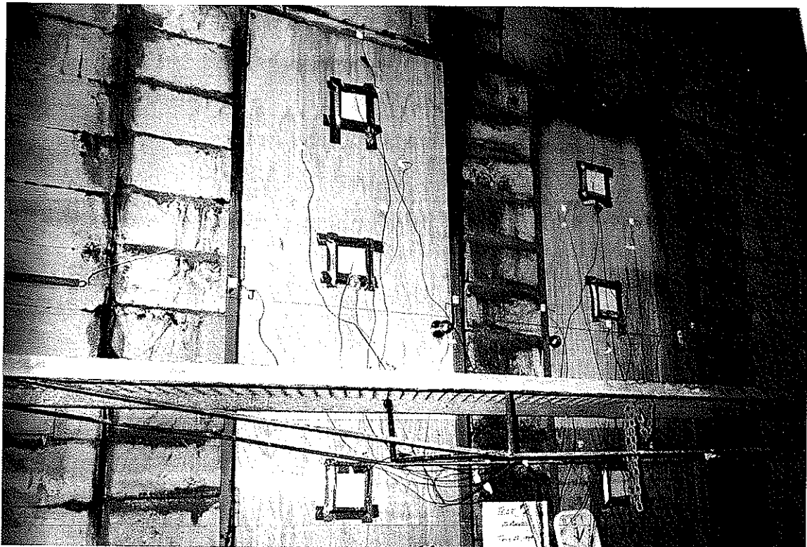
UNEXPOSED SIDE DURING FIRE TEST
