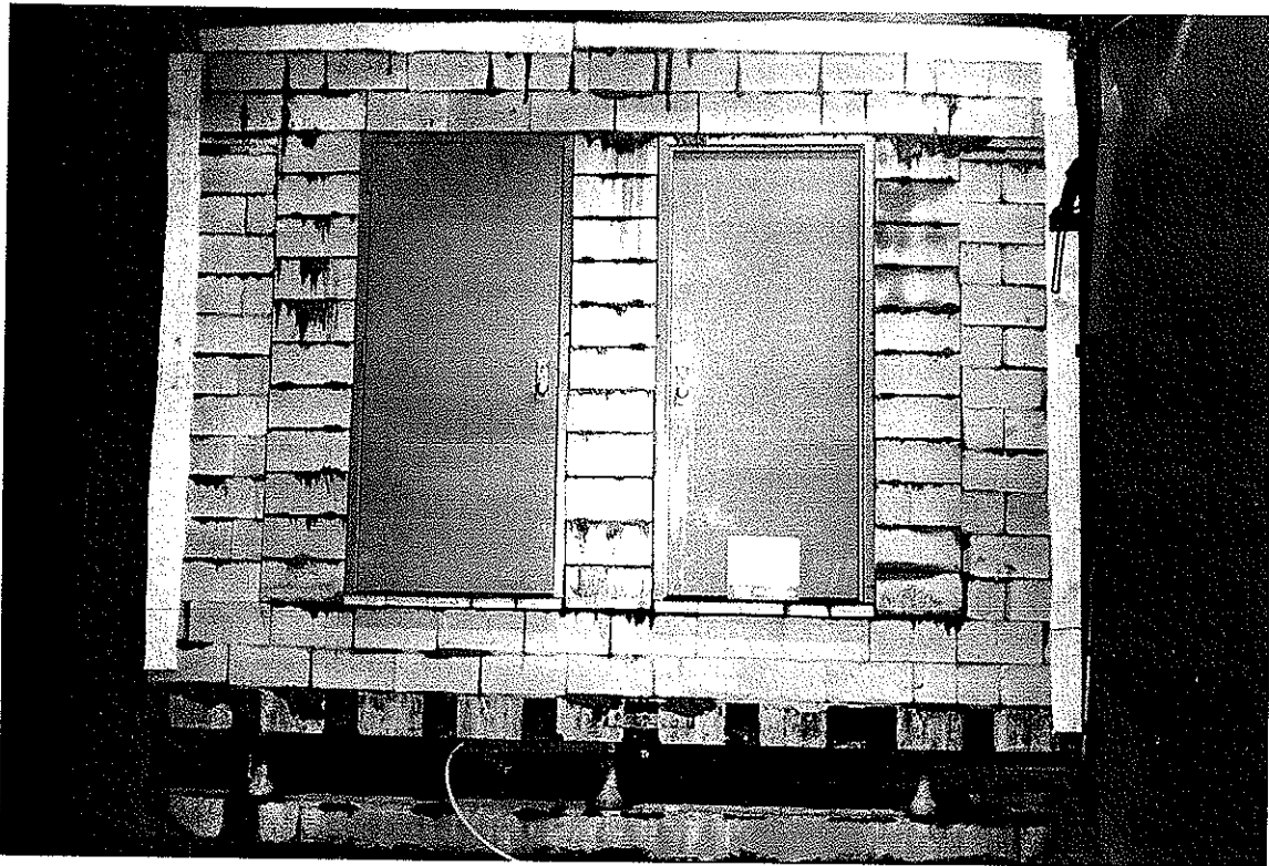
EXPOSED SIDE PRIOR TO FIRE TEST
