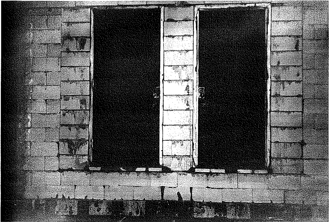
EXPOSED SIDE AFTER HOSE STREAM TEST
