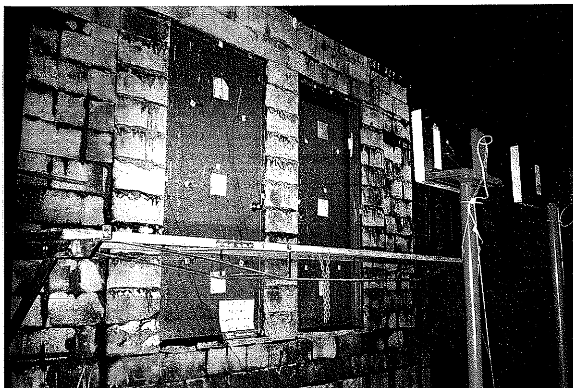
UNEXPOSED SIDE PRIOR TO FIRE TEST
