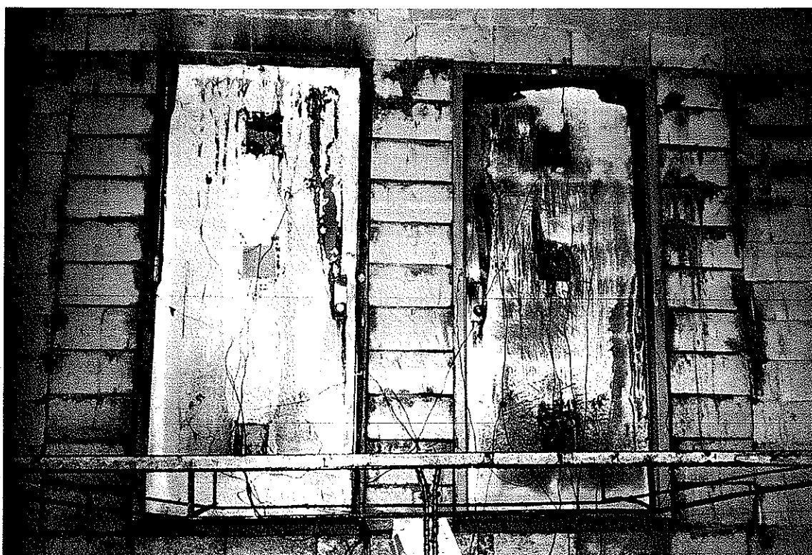
UNEXPOSED SIDE AFTER HOSE STREAM TEST
