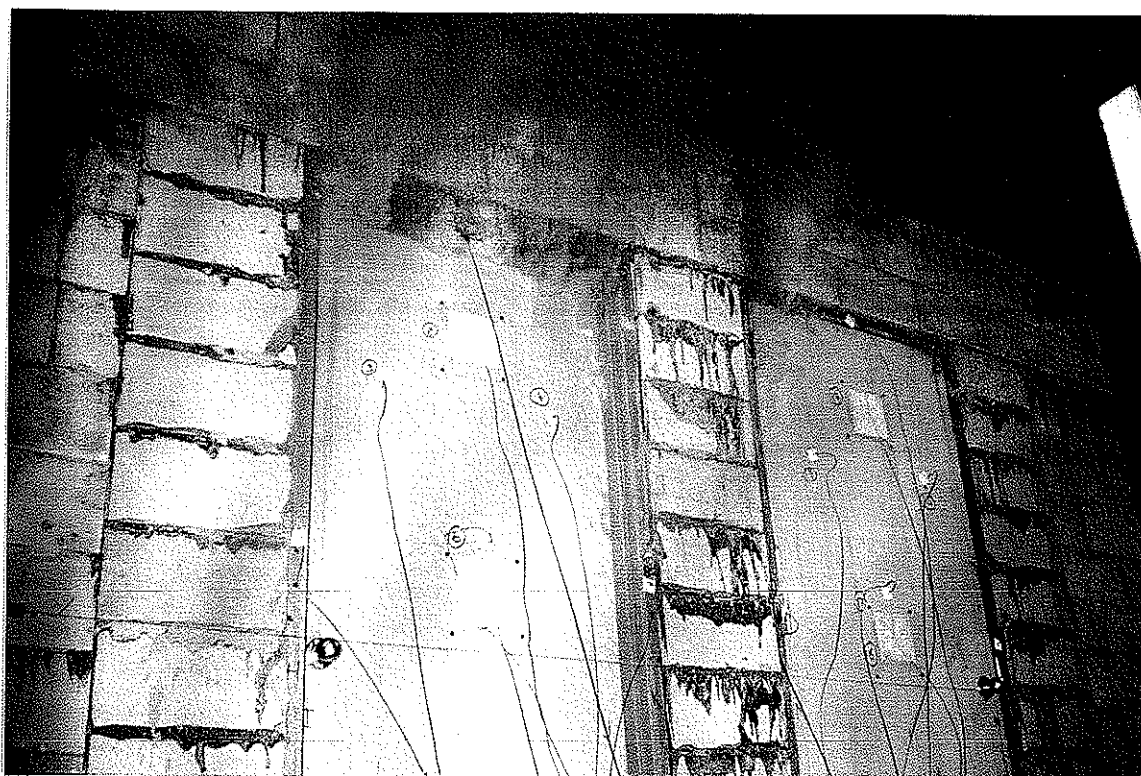
VENTING AT TOP RAIL AND SILL
