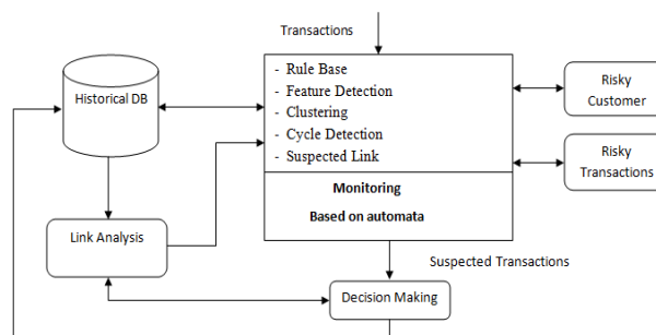
Figure 1: The Monitor Framework Architecture
