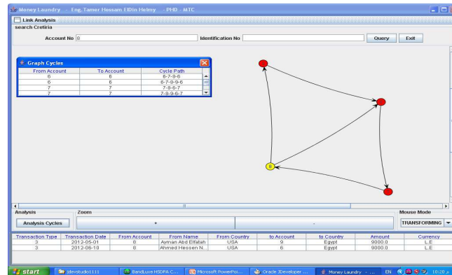
Figure 4: Cycle Detection Phase
