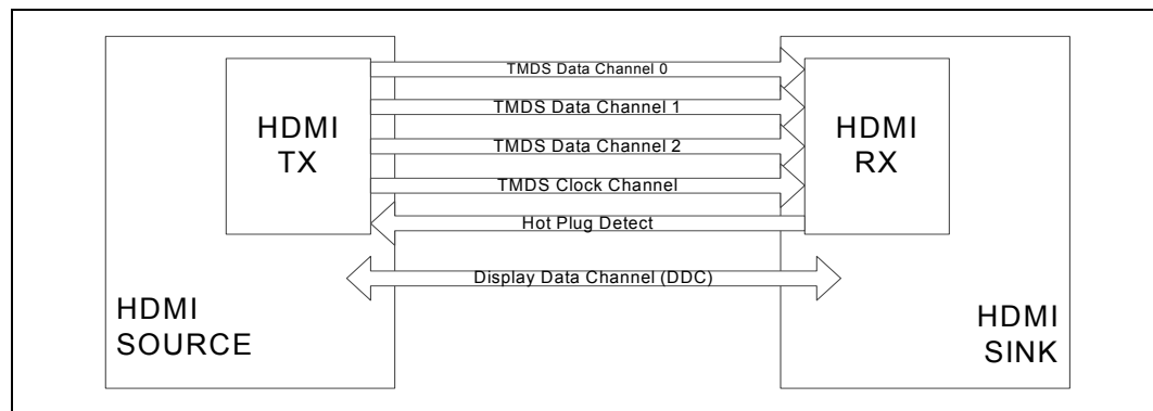
Figure 14. HDMI Overview
