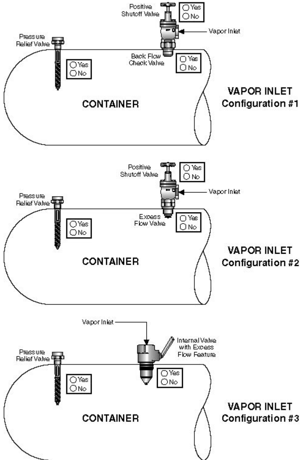
Figure 5-2: Vapor Inlet Appurtenances on Containers of Water Capacity Greater Than 2,000 Gallons
