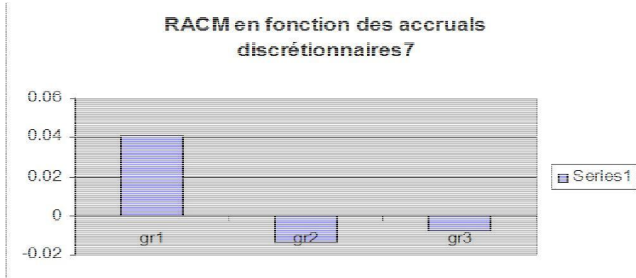
Figure 7. RACM in terms of discretionary accruals computed with model (7).
