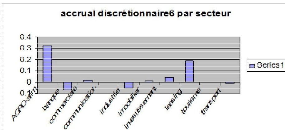
Figure 3. Discretionary accruals by sector computed with model (6).
