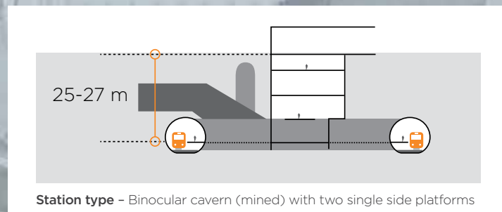
Station type - Binocular cavern (mined) with two single side platforms
