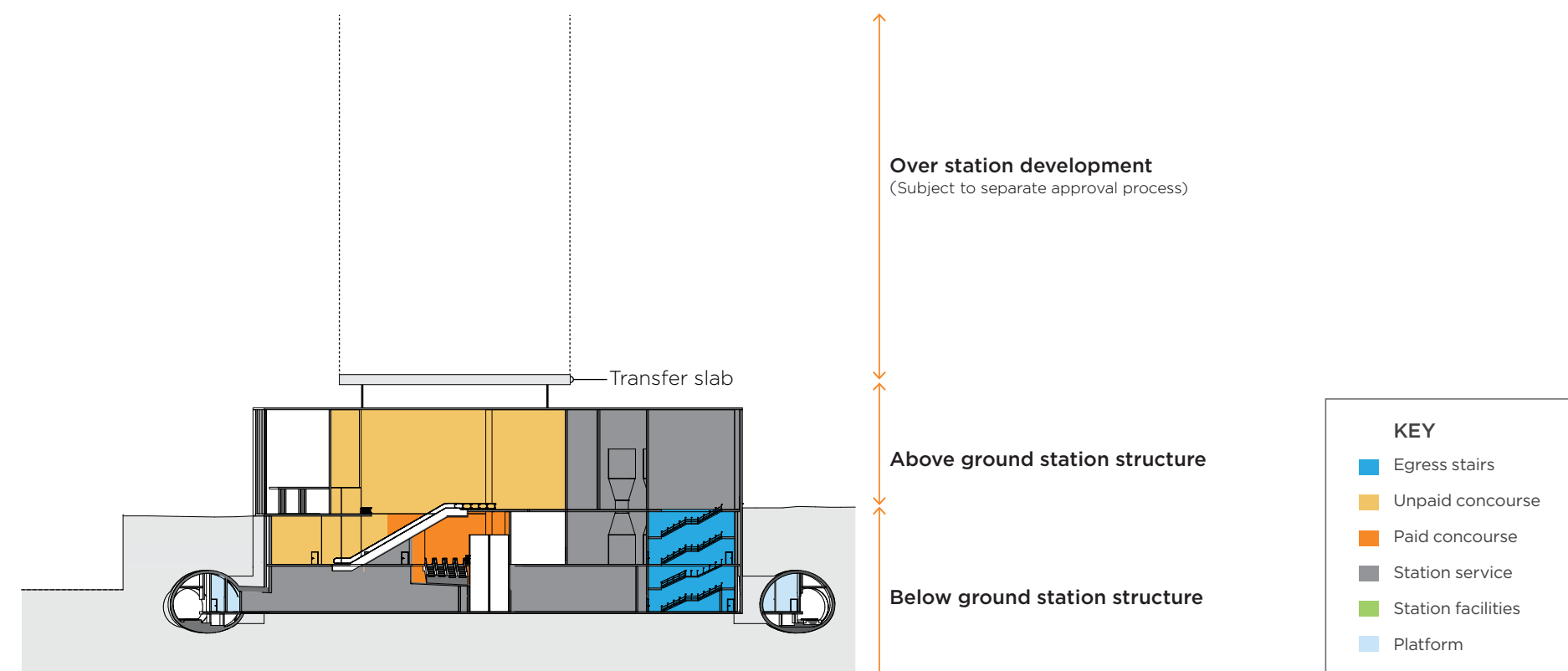
Typical over station development interface
