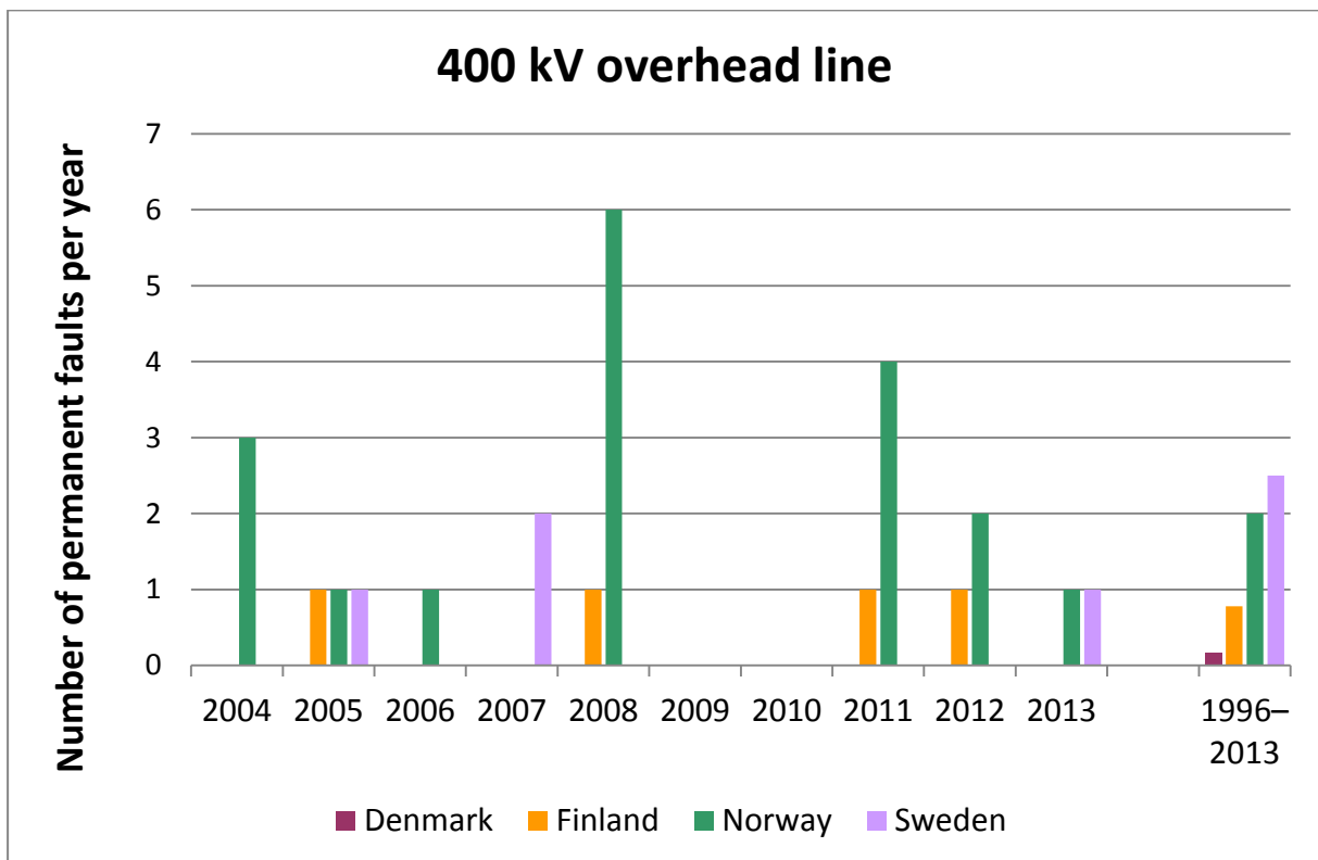
FIGURE 5.3.2 ANNUAL DIVISION OF PERMANENT FAULTS DURING THE PERIOD 2004–2013
