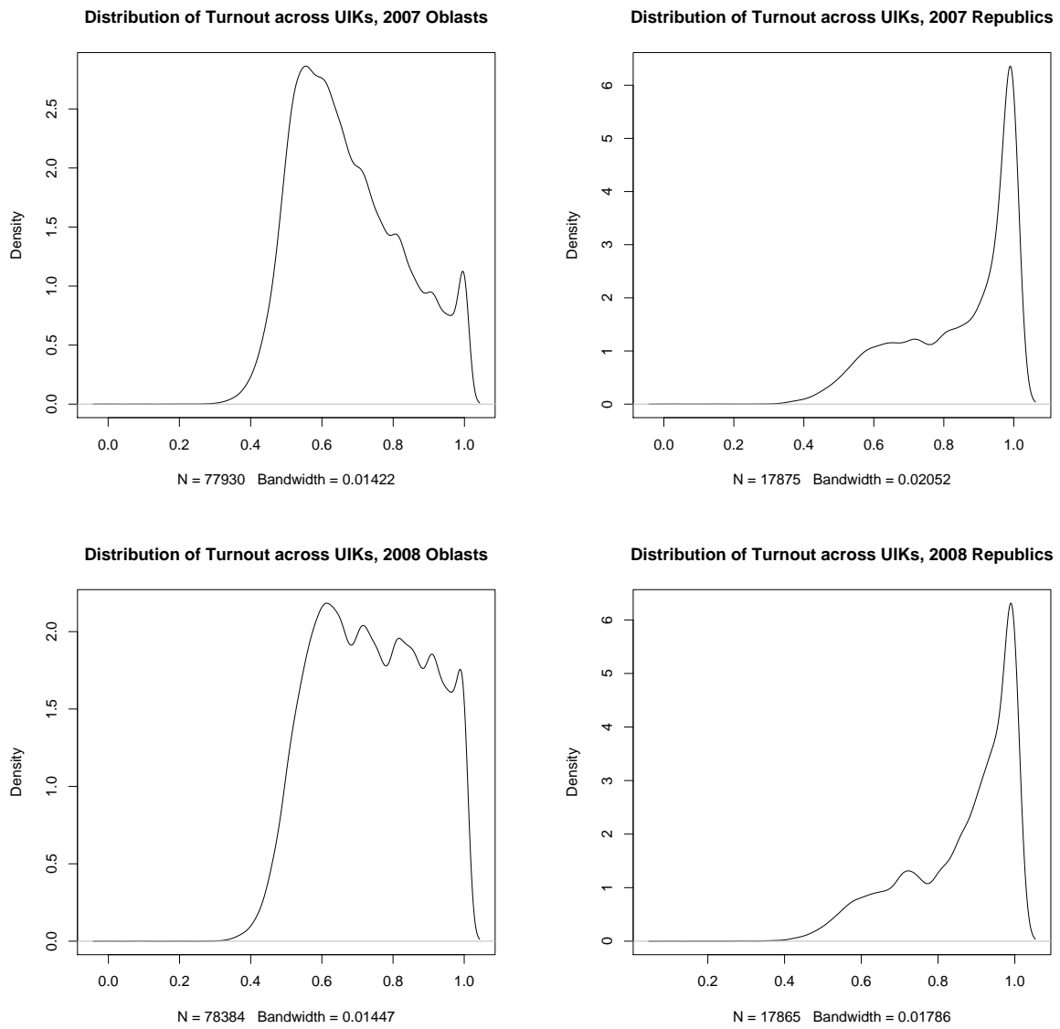
Figure 2: UIK turnout, 2007 and 2008
