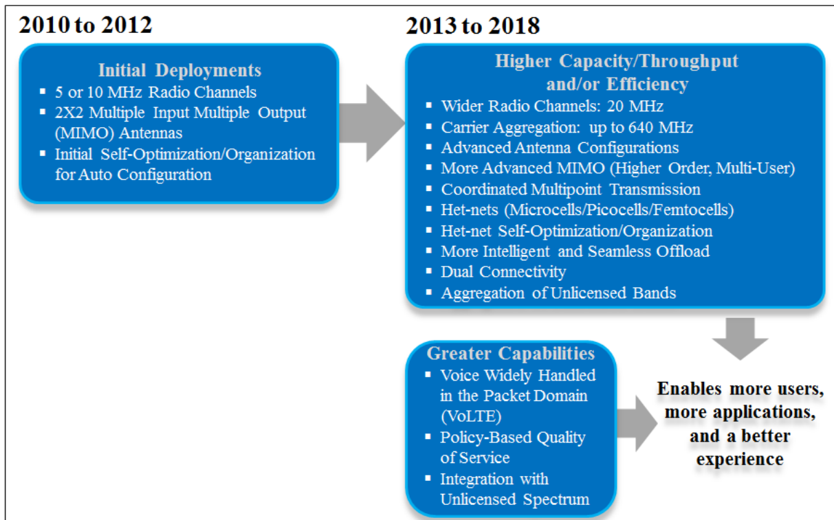
Figure 10: LTE to LTE-Advanced Pro Migration 24
