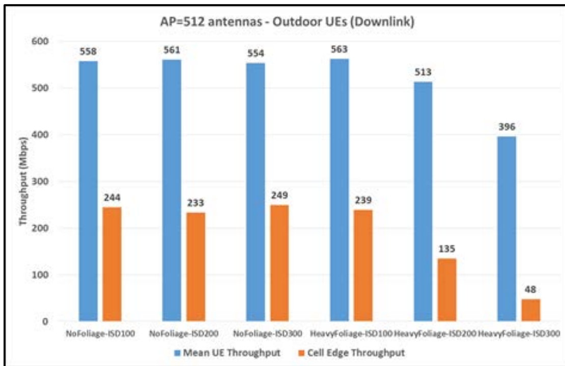
Figure 51: Downlink Performance, Different ISDs, Foliage vs. None 127
