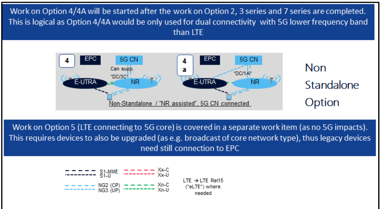
Figure 47: De-Prioritized 5G Network Architecture Options in 3GPP Release 15
