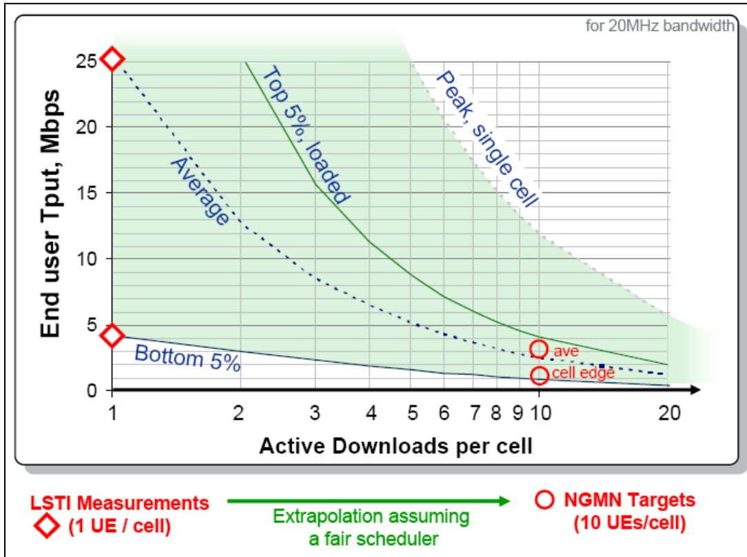
Figure 76: LTE Actual Throughput Rates Based on Conditions 163
