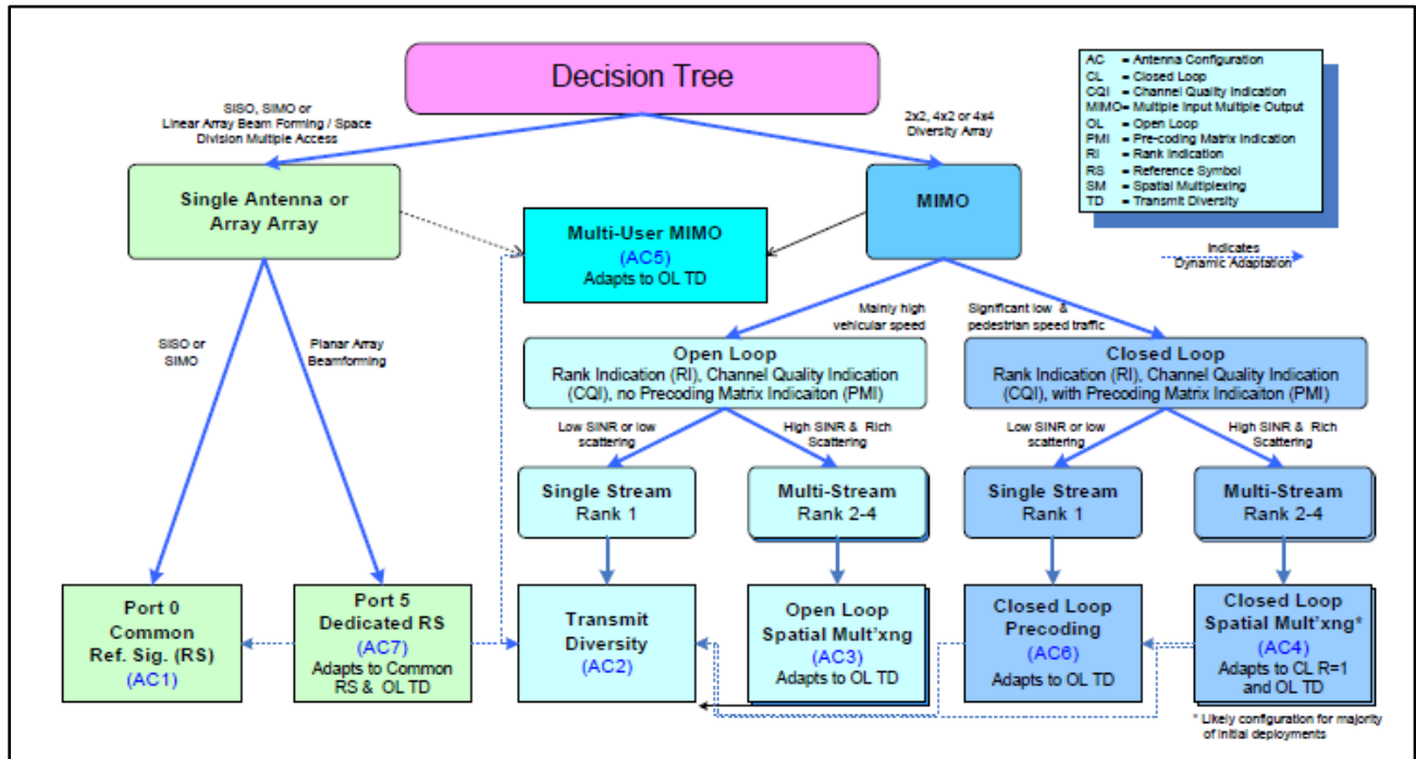
Figure 59: Decision Tree for Different Antenna Schemes 134
