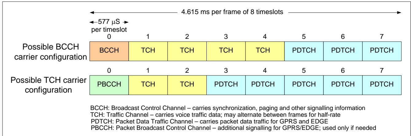
Figure 115: Example of GSM/EDGE Timeslot Structure 213
