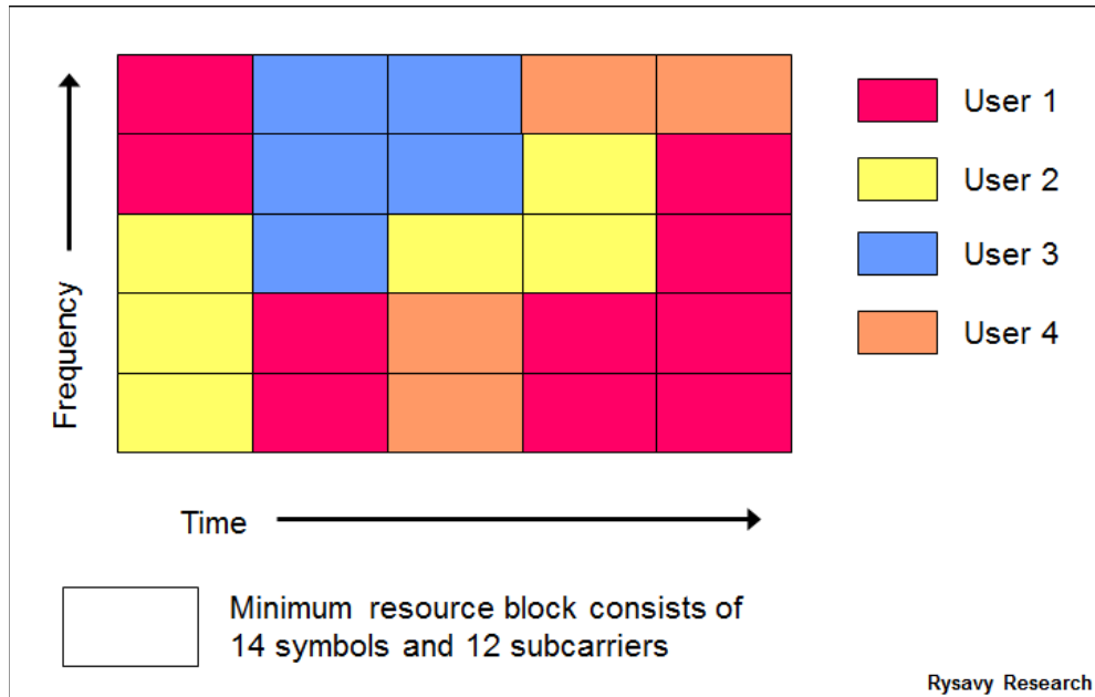
Figure 57: LTE OFDMA Downlink Resource Assignment in Time and Frequency
