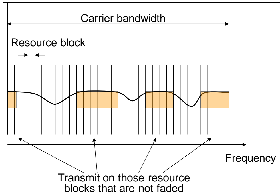
Figure 58: Frequency Domain Scheduling in LTE 132
