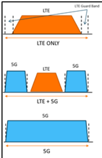
Figure 49: Frequency Domain Coexistence of LTE and NR 125
