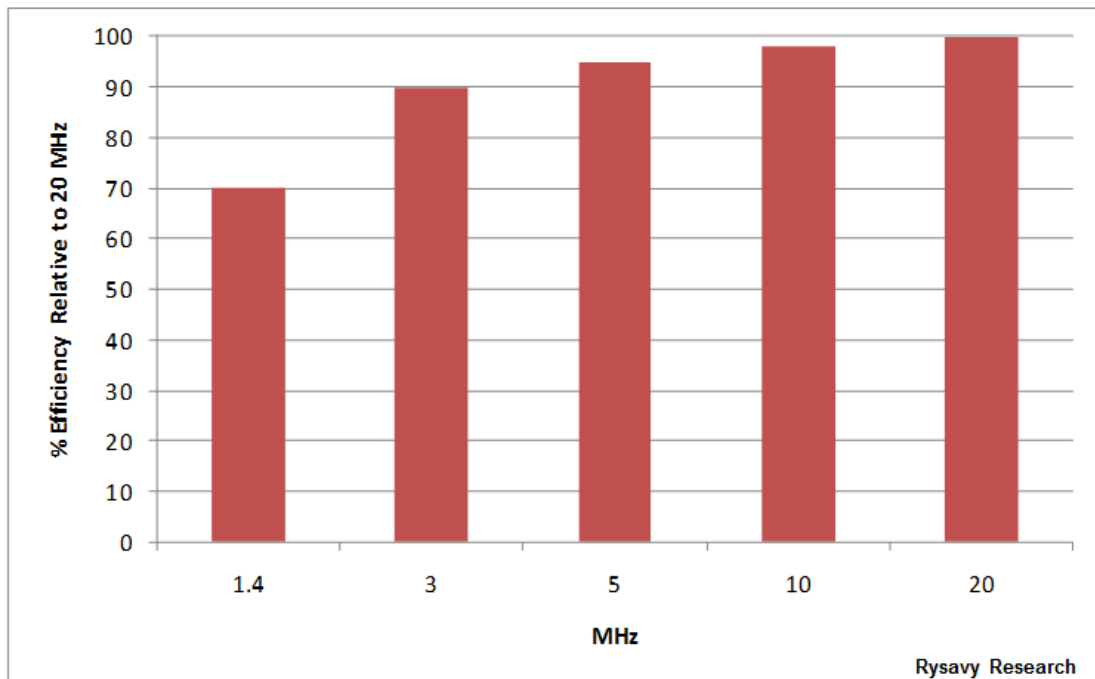
Figure 34: LTE Spectral Efficiency as Function of Radio Channel Size 90
