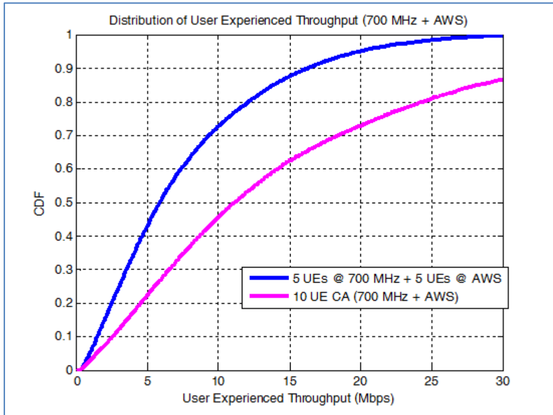
Figure 69: Gains from Carrier Aggregation 146
