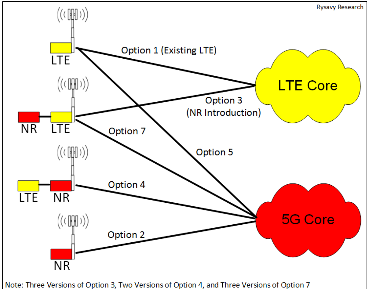
Figure 18: Release 15 Non-Standalone and Standalone Options
