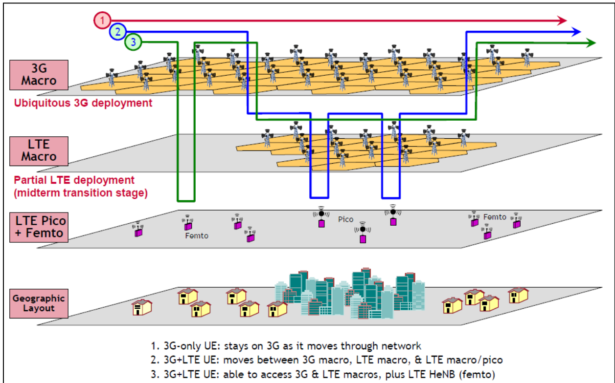
Figure 82: Load Balancing with Heterogeneous Networks 175
