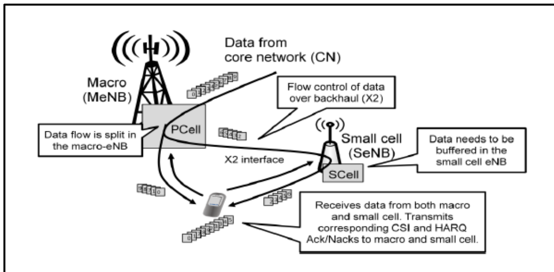
Figure 90: Dual Connectivity 183
