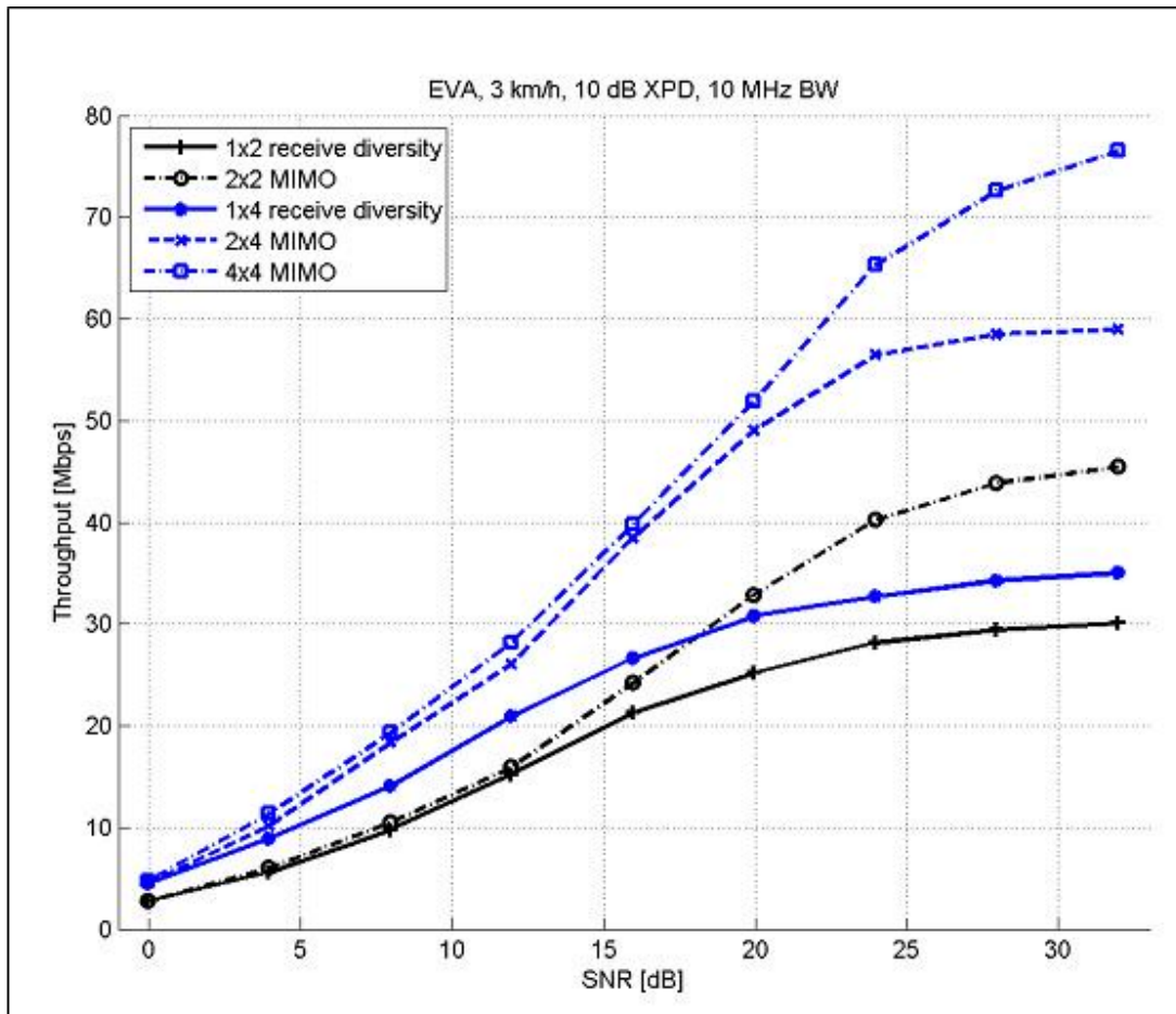
Figure 75: LTE Throughput in Various Modes 162
