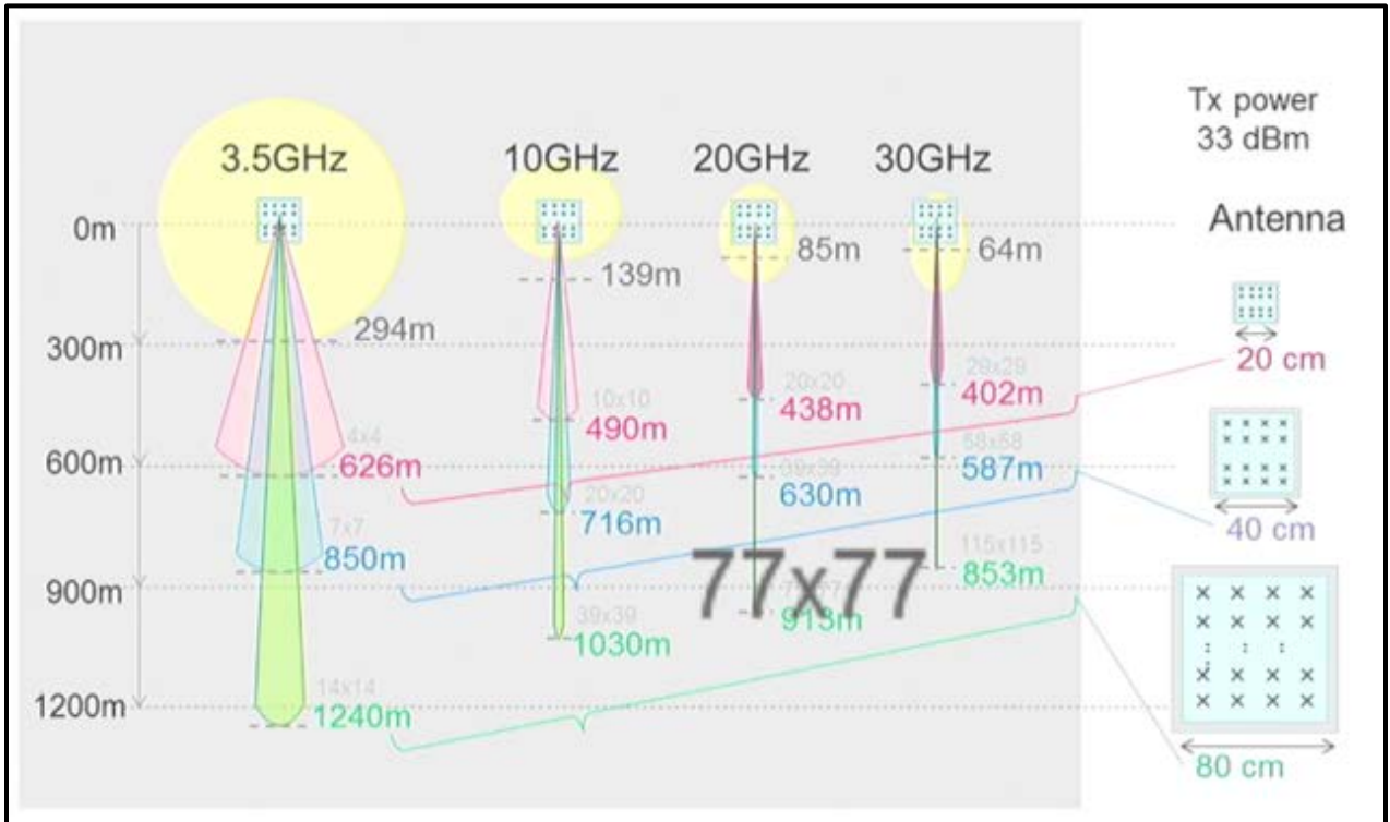
Figure 20: Range Relative to Number of Antenna Elements 37
