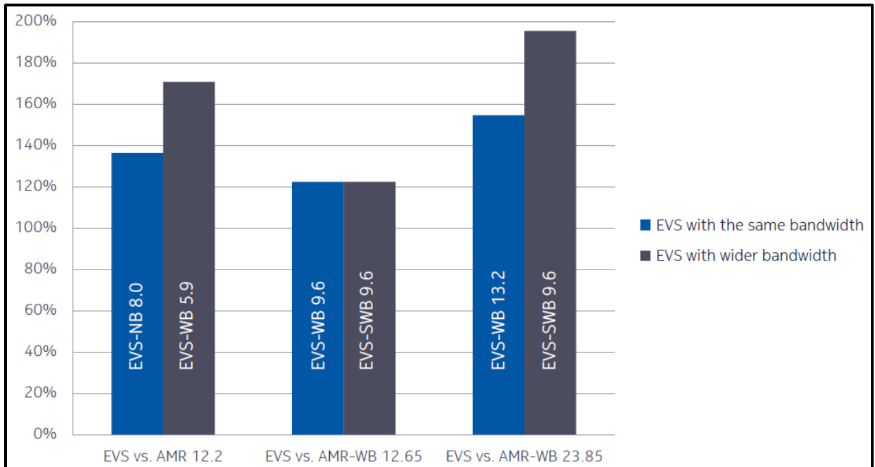
Figure 80: EVS Voice Capacity Compared to AMR and AMR-WB 173
