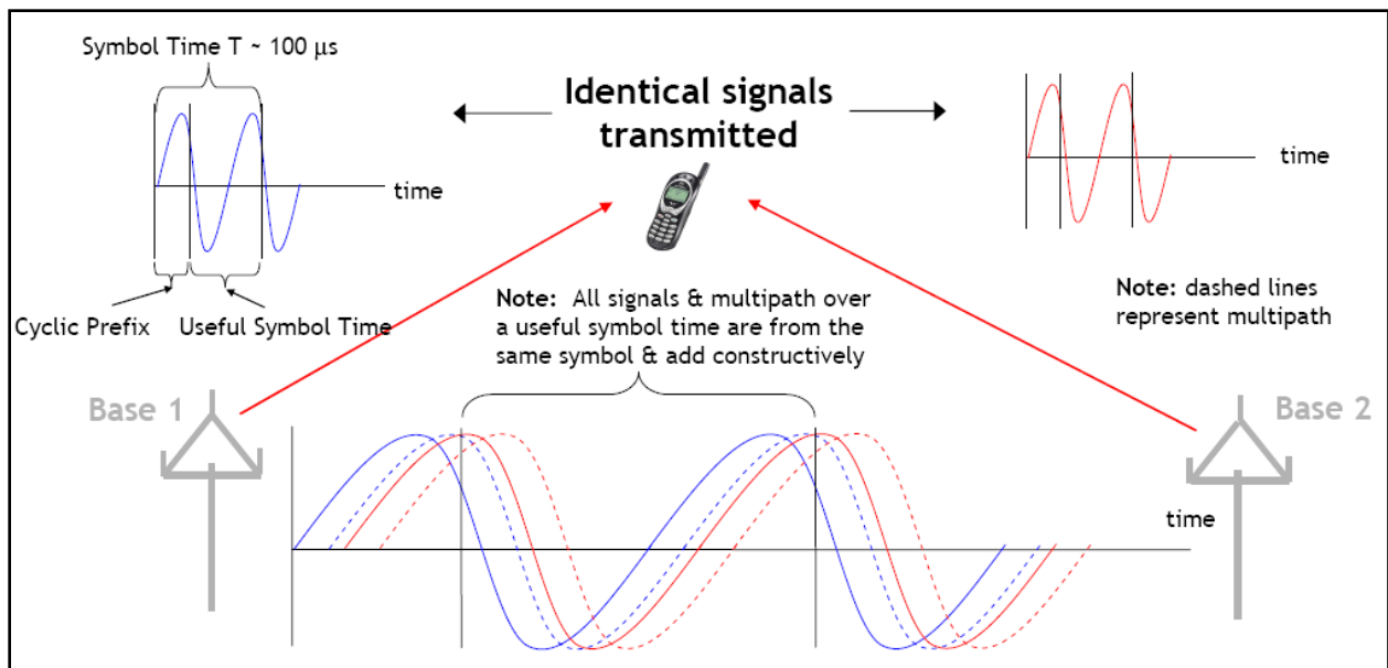
Figure 103: OFDM Enables Efficient Broadcasting
