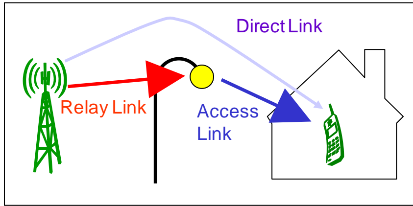
Figure 73: LTE-Advanced Relay 155
