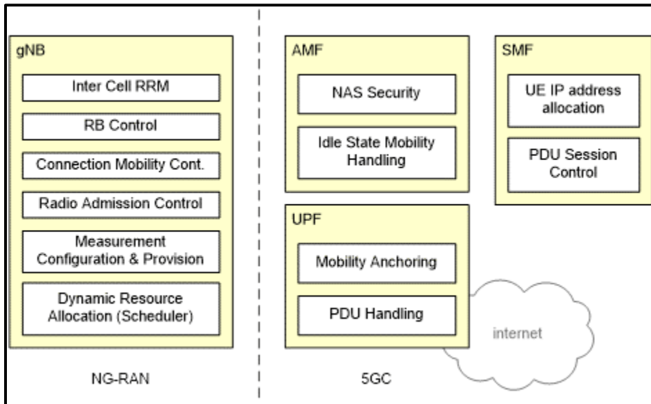
Figure 45: Functional Split between NG-RAN and 5G 123
