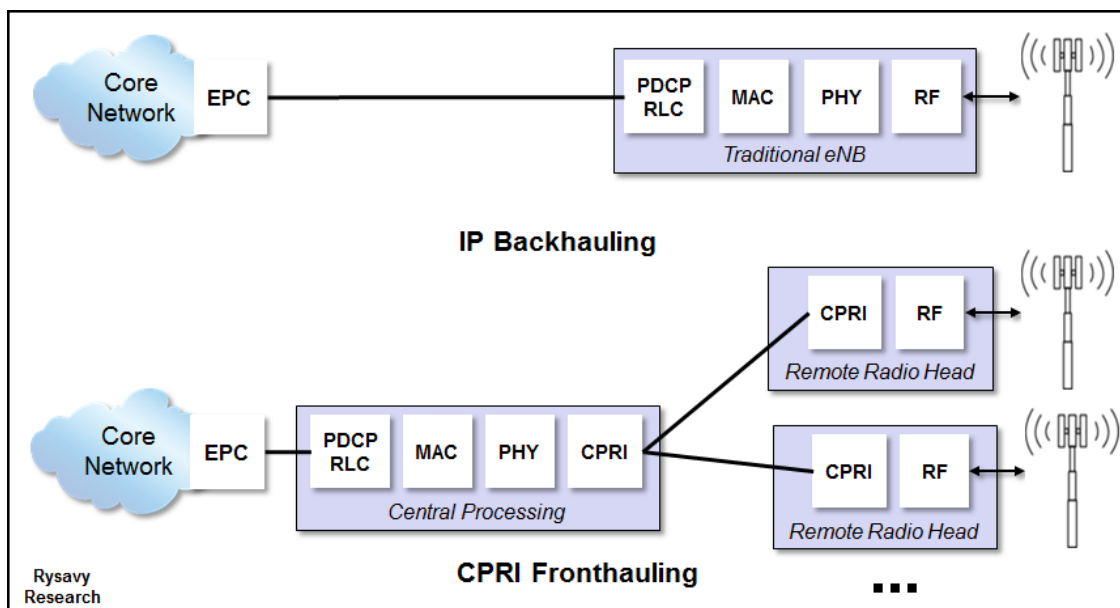
Figure 93: Potential Cloud RAN Approach
