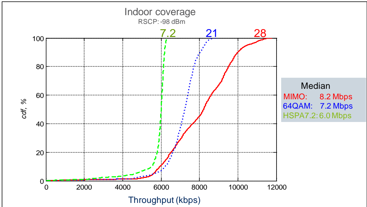
Figure 111: HSPA+ Performance Measurements Commercial Network (5+5 MHz) 207
