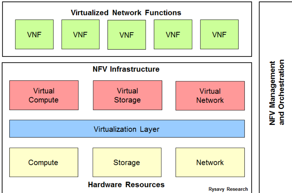
Figure 26: ETSI NFV High-Level Framework
