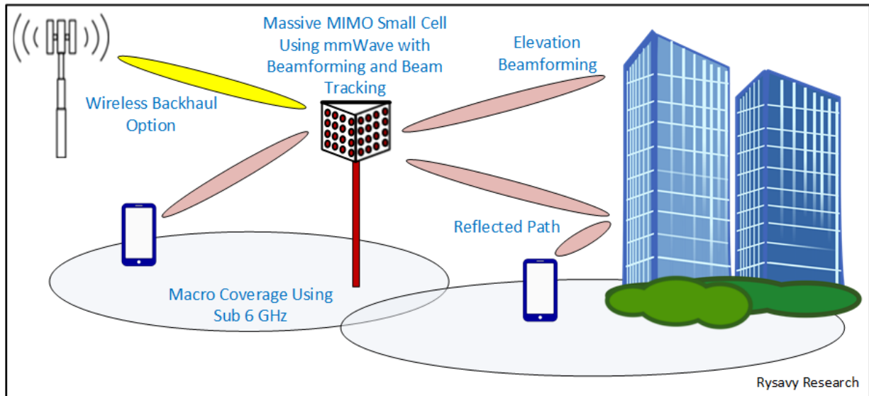
Figure 21: 5G Architecture for Low-Band/High-Band Integration
