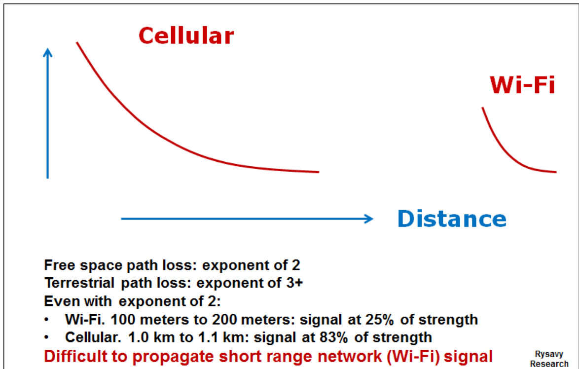
Figure 35: Propagation Losses of Cellular vs. Wi-Fi 95
