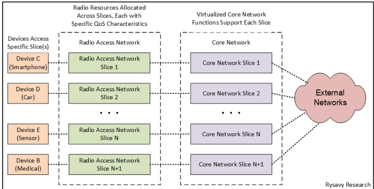
Figure 22: Network Slicing Architecture
