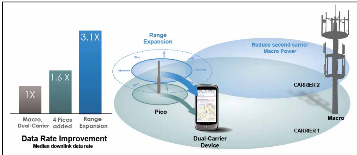
Figure 110: HSPA+ HetNet Using Multipoint Transmission 205
