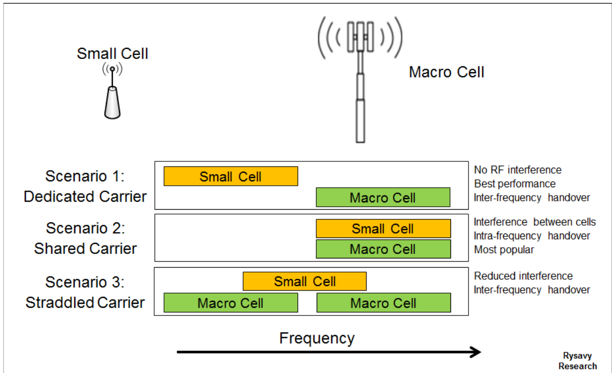
Figure 83: Scenarios for Radio Carriers in Small Cells
