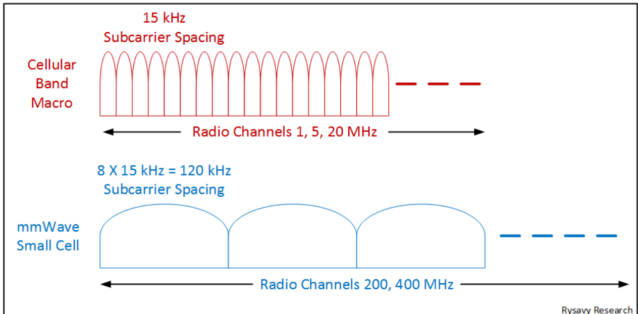
Figure 17: Hypothetical Example of 5G Numerology
