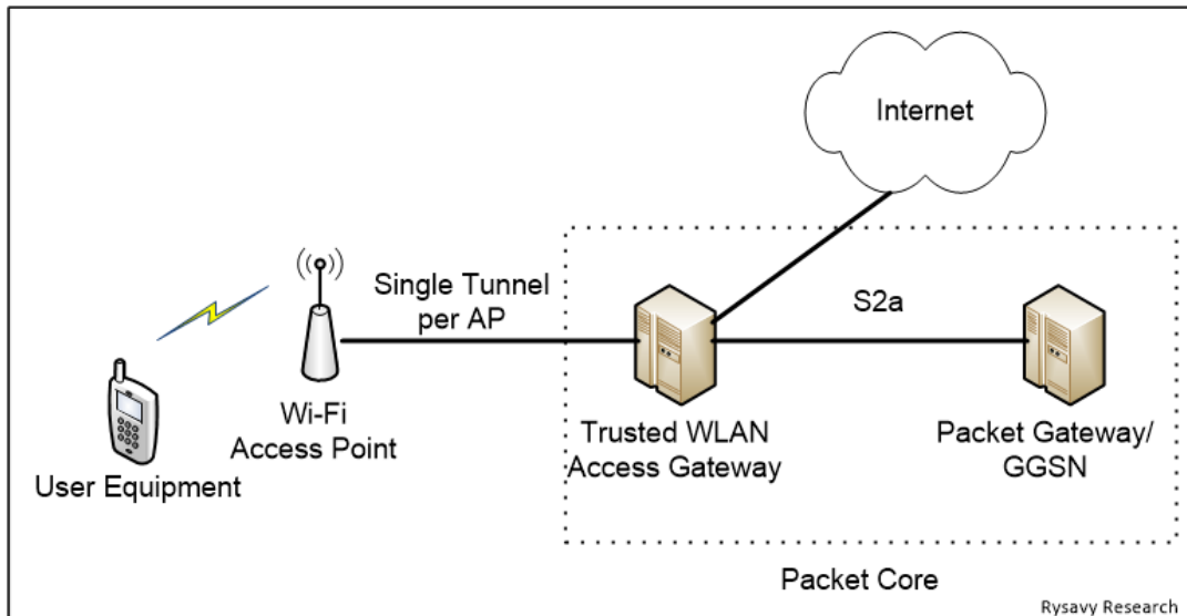
Figure 96: Release 11 SaMOG-based Wi-Fi Integration
