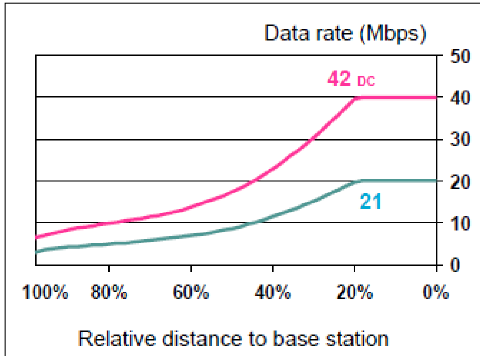
Figure 112: Dual-Carrier HSPA+ Throughputs 208
