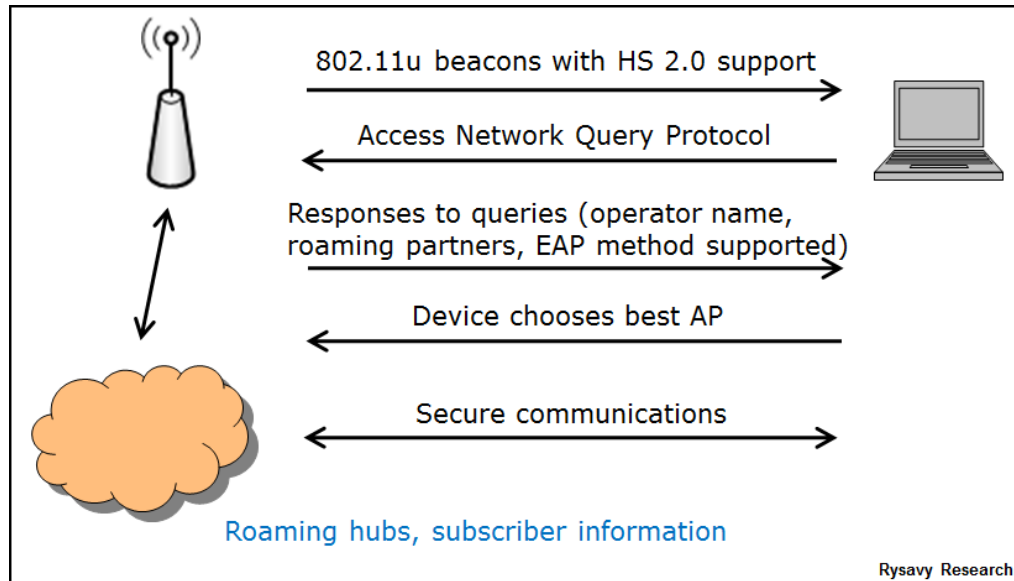
Figure 100: Hotspot 2.0 Connection Procedure
