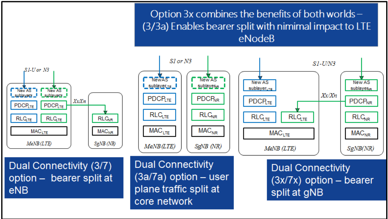
Figure 48: Dual-Connectivity Options with LTE as Master
