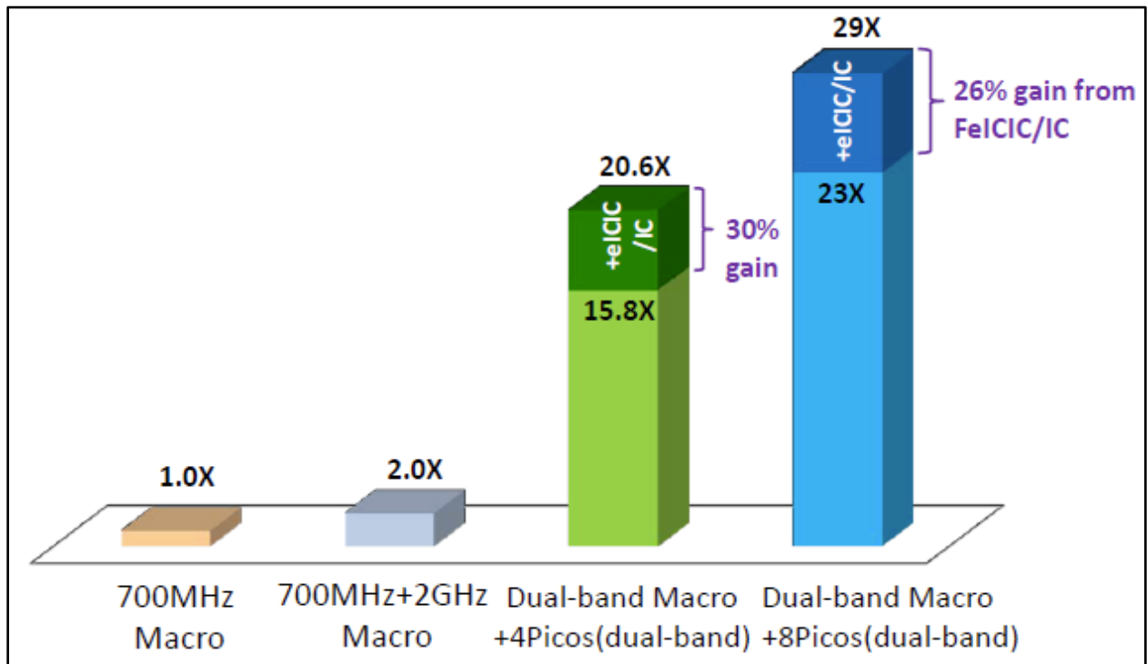
Figure 86: Median Throughput Gains in Hotspot Scenarios 178
