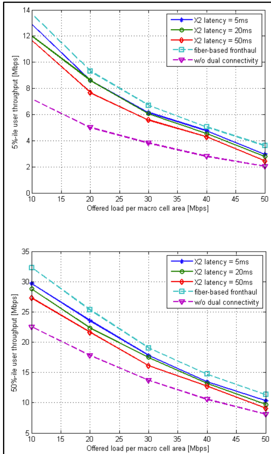
Figure 91: Dual Connectivity User Throughput 184
