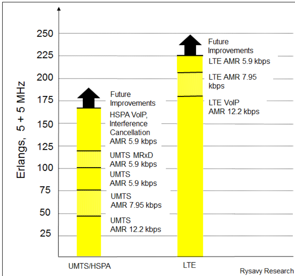
Figure 43: Comparison of Voice Spectral Efficiency 118
