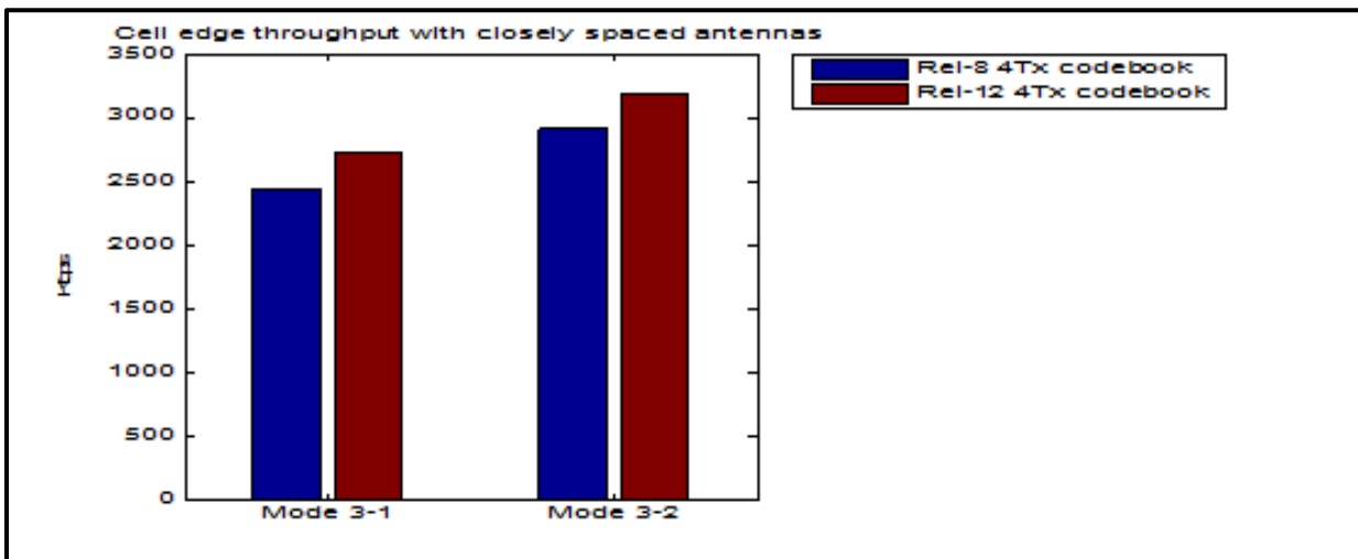
Figure 63: Cell-Edge Throughput of Feedback Mode 3-2 and New Codebook 138
