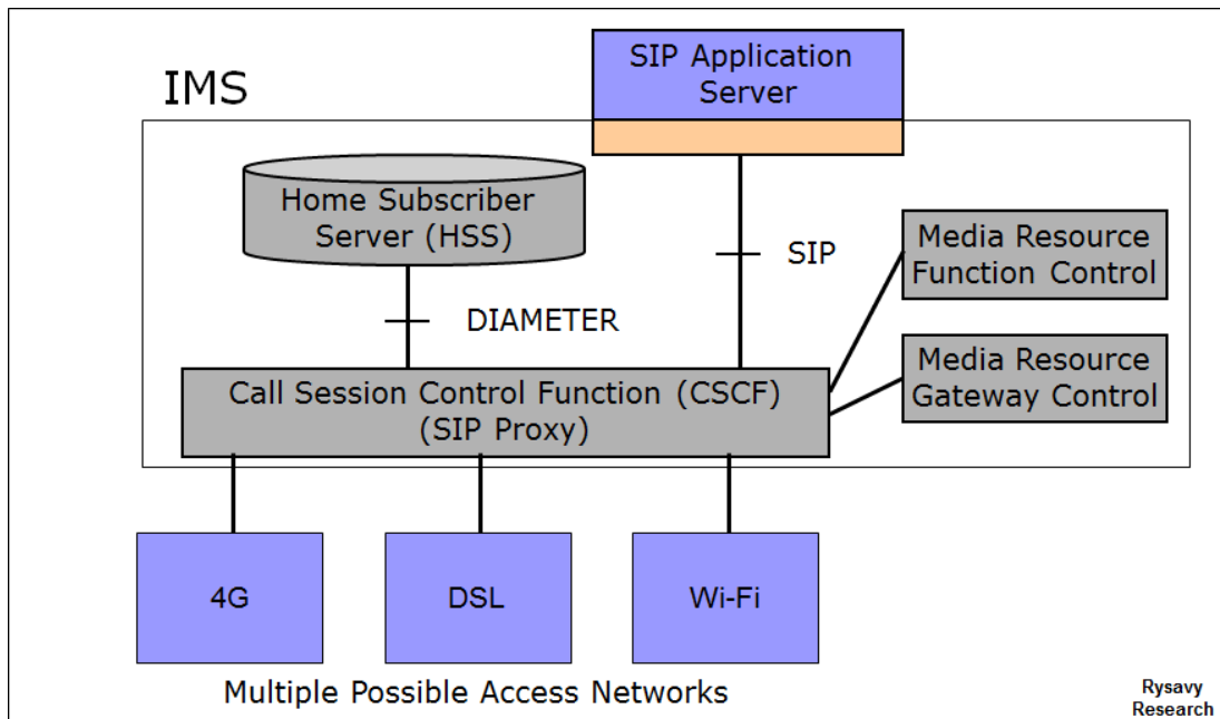
Figure 102: IP Multimedia Subsystem
