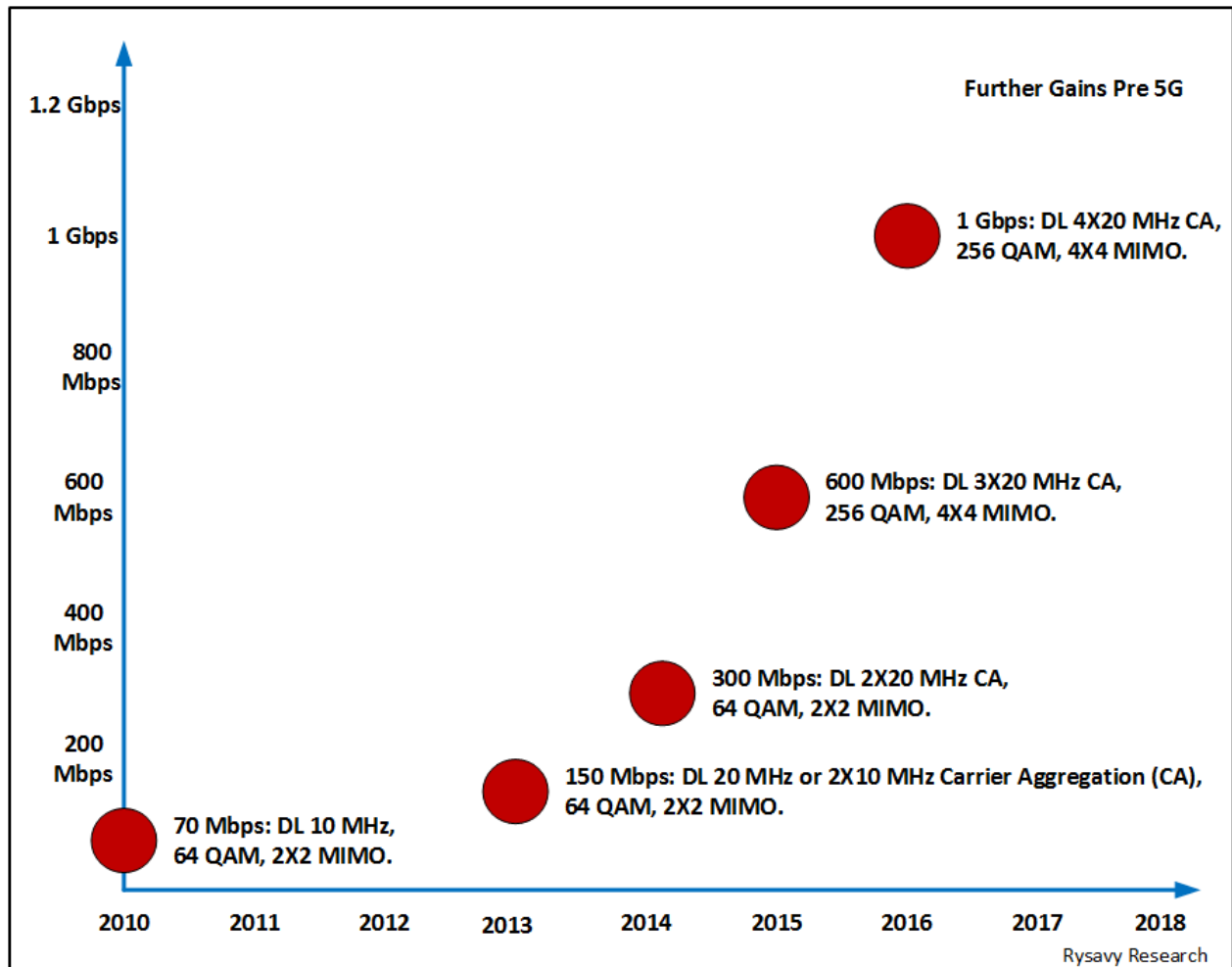
Figure 11: Successive Gains in Peak LTE Downlink Throughput 25
