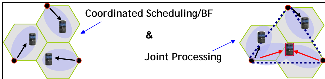
Figure 71: Coordinated Scheduling/BF and Joint Processing CoMP Approaches 148
