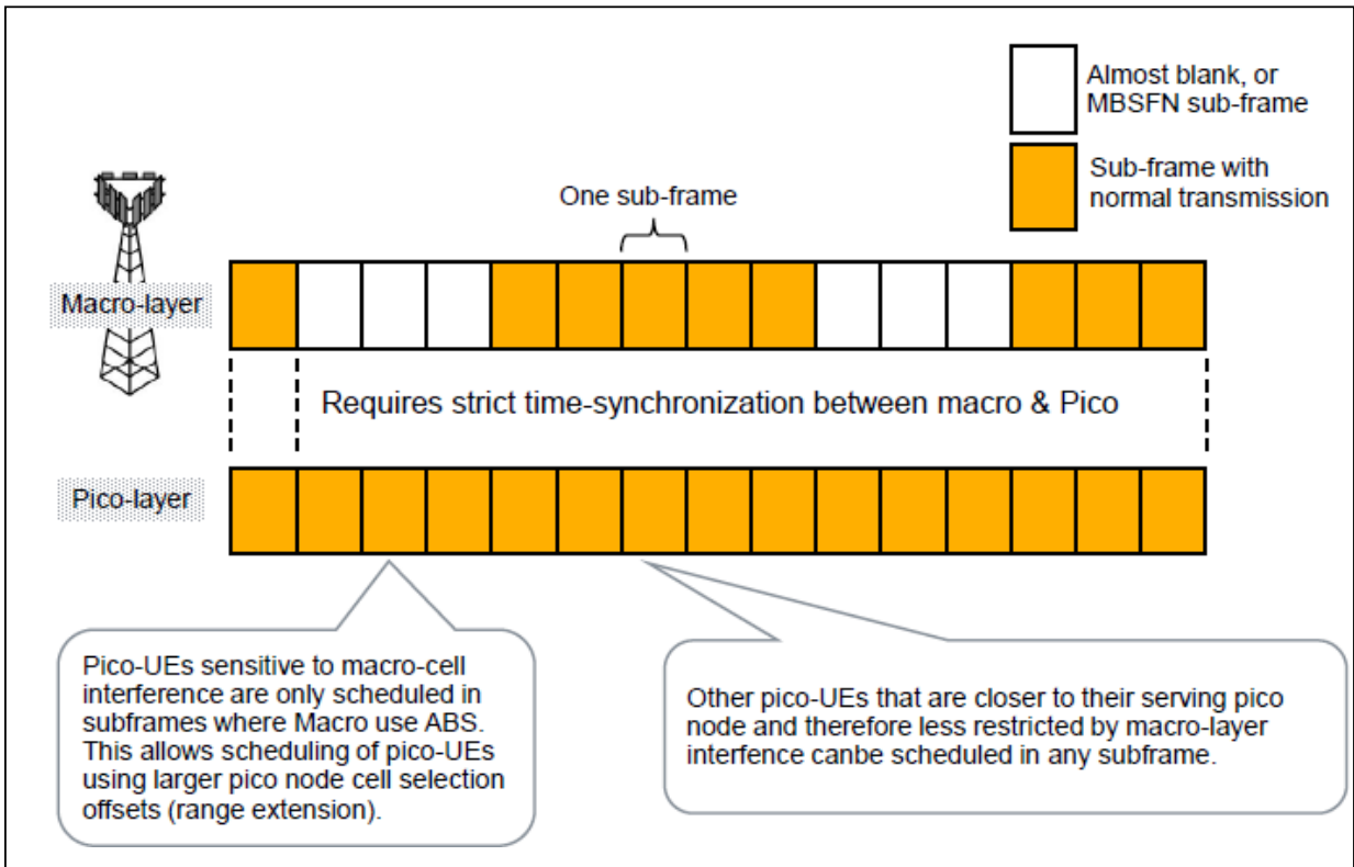
Figure 85: Example of Enhanced Inter-cell Interference Coordination 177
