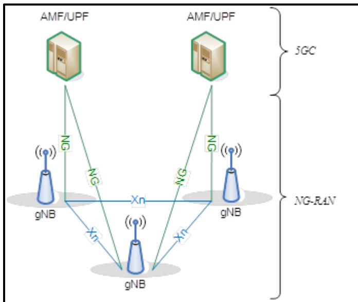
Figure 44: 5G Architecture 122
