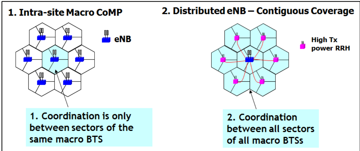
Figure 70: Different Coordination Levels for CoMP 147
