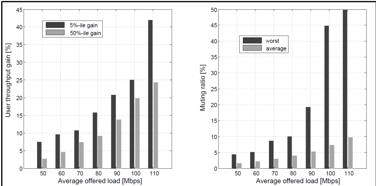
Figure 88: Throughput Gain of Time-Domain Interference Coordination 181
