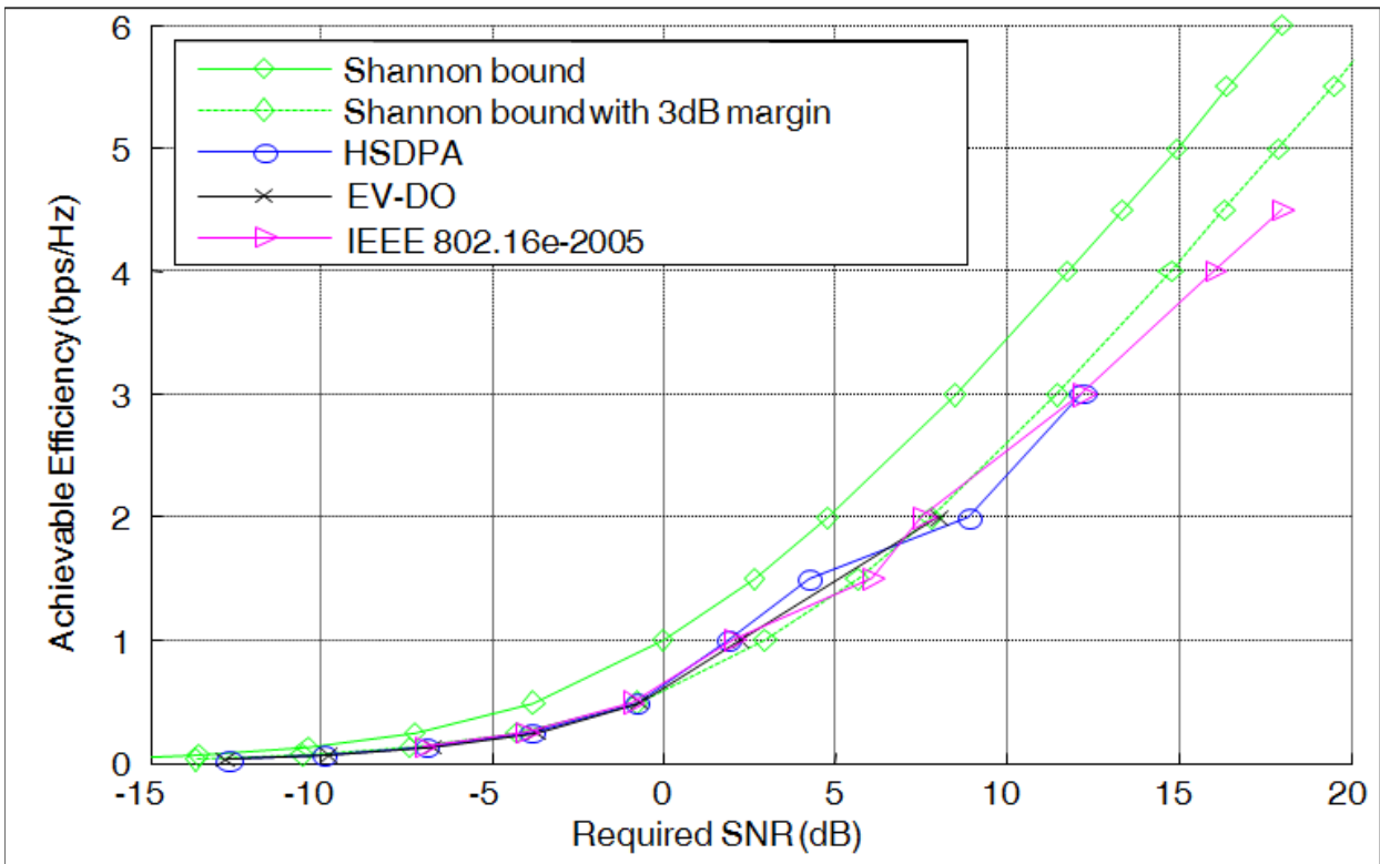
Figure 40: Performance Relative to Theoretical Limits for HSDPA, EV-DO, and WiMAX (IEEE 802.16e-2005) 113
