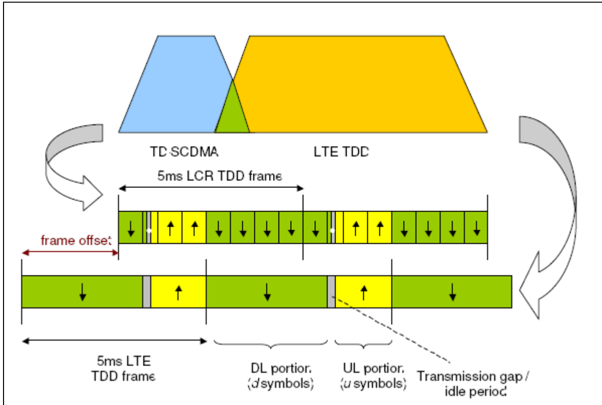
Figure 72: TDD Frame Co-Existence between TD-SCDMA and LTE TDD 152
