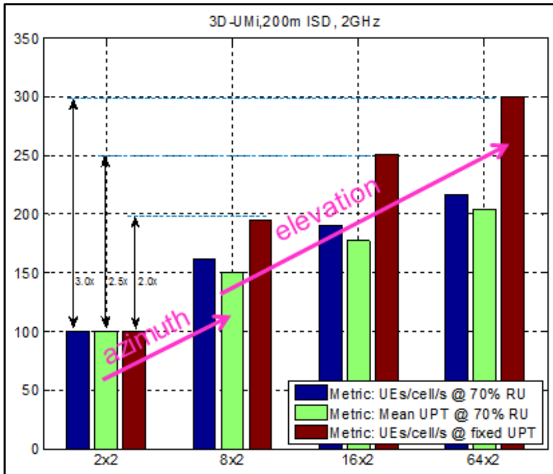
Figure 64: Performance Gains with FD-MIMO Using 200 Meter ISD 139
