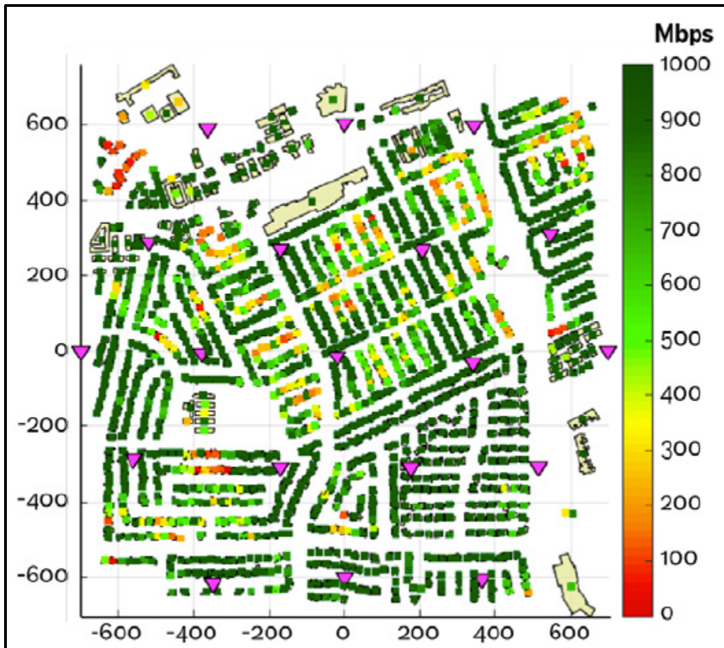
Figure 52: Throughput Map of Suburban Area at Low Load 128
