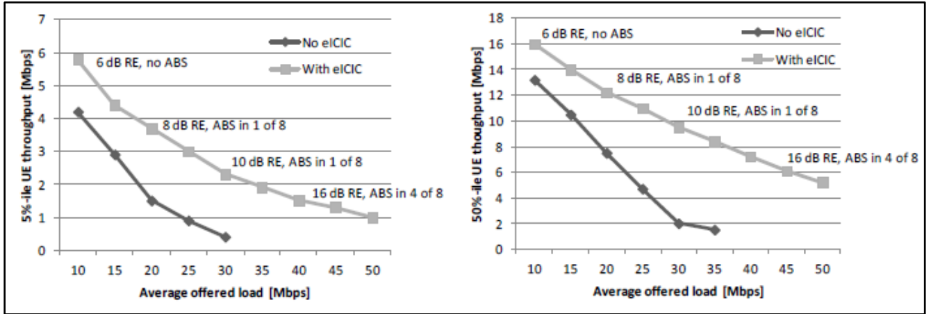
Figure 87: User Throughput Performance With/Without eICIC for Dynamic Traffic vs. Average Offered Load per Macro Cell Area 180
