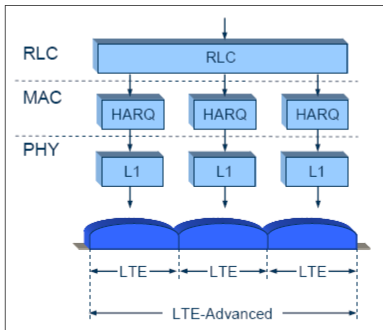
Figure 68: Carrier Aggregation at Different Protocol Layers 145
