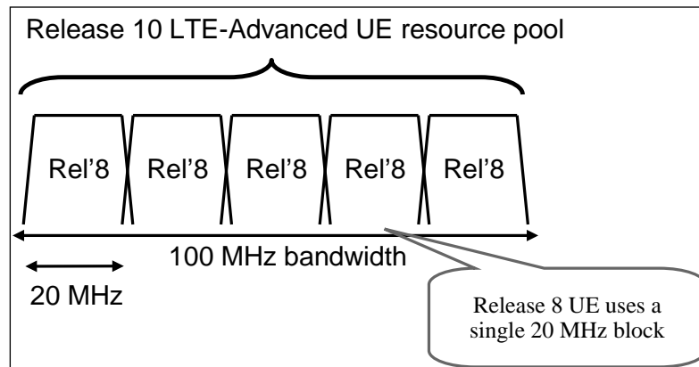
Figure 67: Release 10 LTE-Advanced Carrier Aggregation 144
