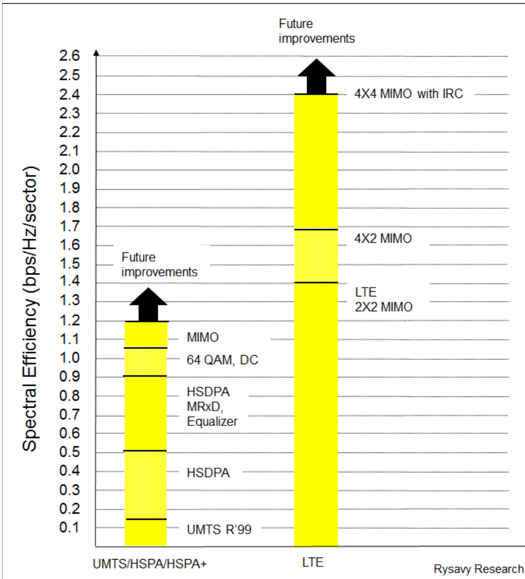
Figure 41: Comparison of Downlink Spectral Efficiency 114
