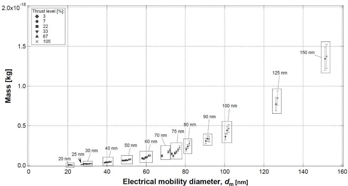
Figure 3.3 Electrical mobility diameter ( d_m ) vs. mass ( m ) from PM exhaust from a CFM56-7B26/3 engine. The data points are grouped into boxes each showing the measured masses for a certain d_m at different thrust. They are depicted with a slight offset in x-direction such that the thrust in one box increases from left to right.
