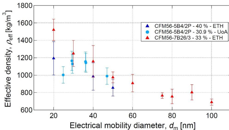
Figure 3.7 Comparison of effective densities derived by our measurements (triangles) from a CFM56-7B26/3 (red) and a CFM56-5B4/2P (dark blue) engine to literature values measured by Johnson et al. (2015) (circles) from a CFM56-5B4/2P engine at similar thrust levels.
