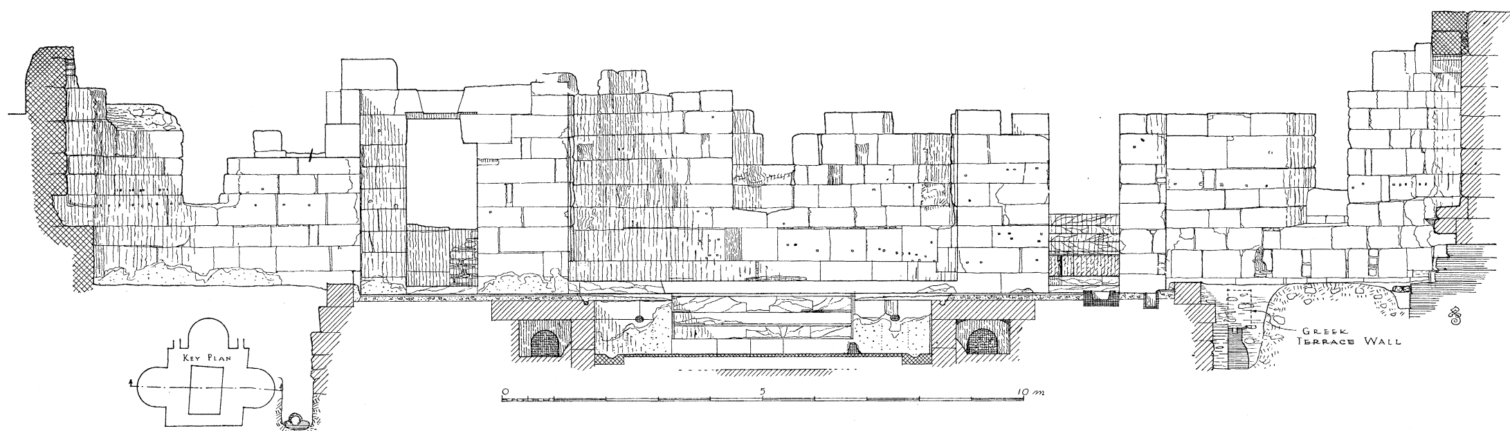
I. PEIRENE: ELEVATION OF NORTH SIDE OF COURT AND SECTION THROUGH WEST AND EAST EXEDRAE, PRESENT STATE
