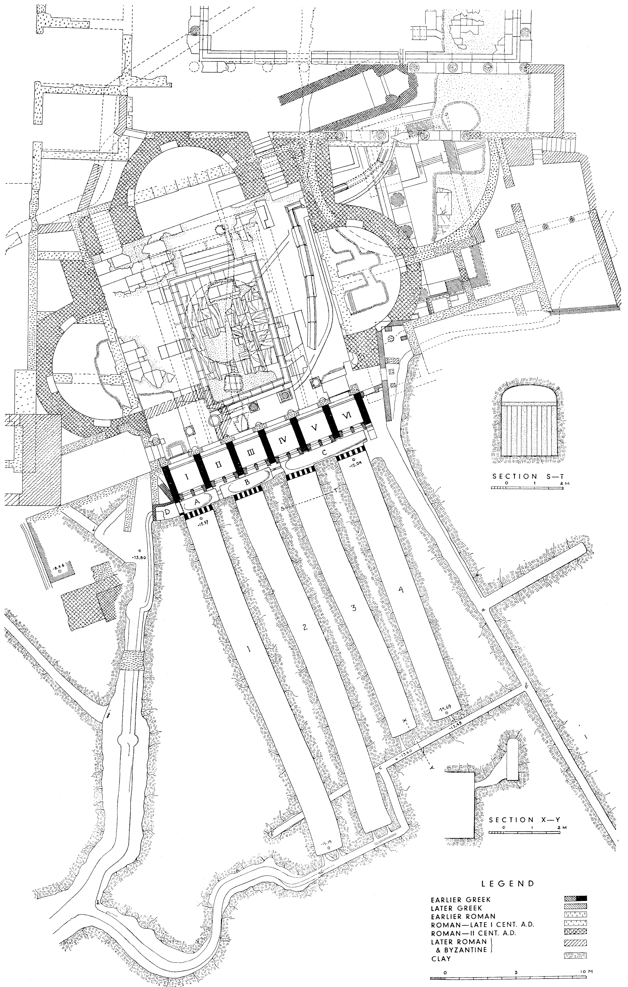
PEIRENE: PLAN SHOWING PERIODS
