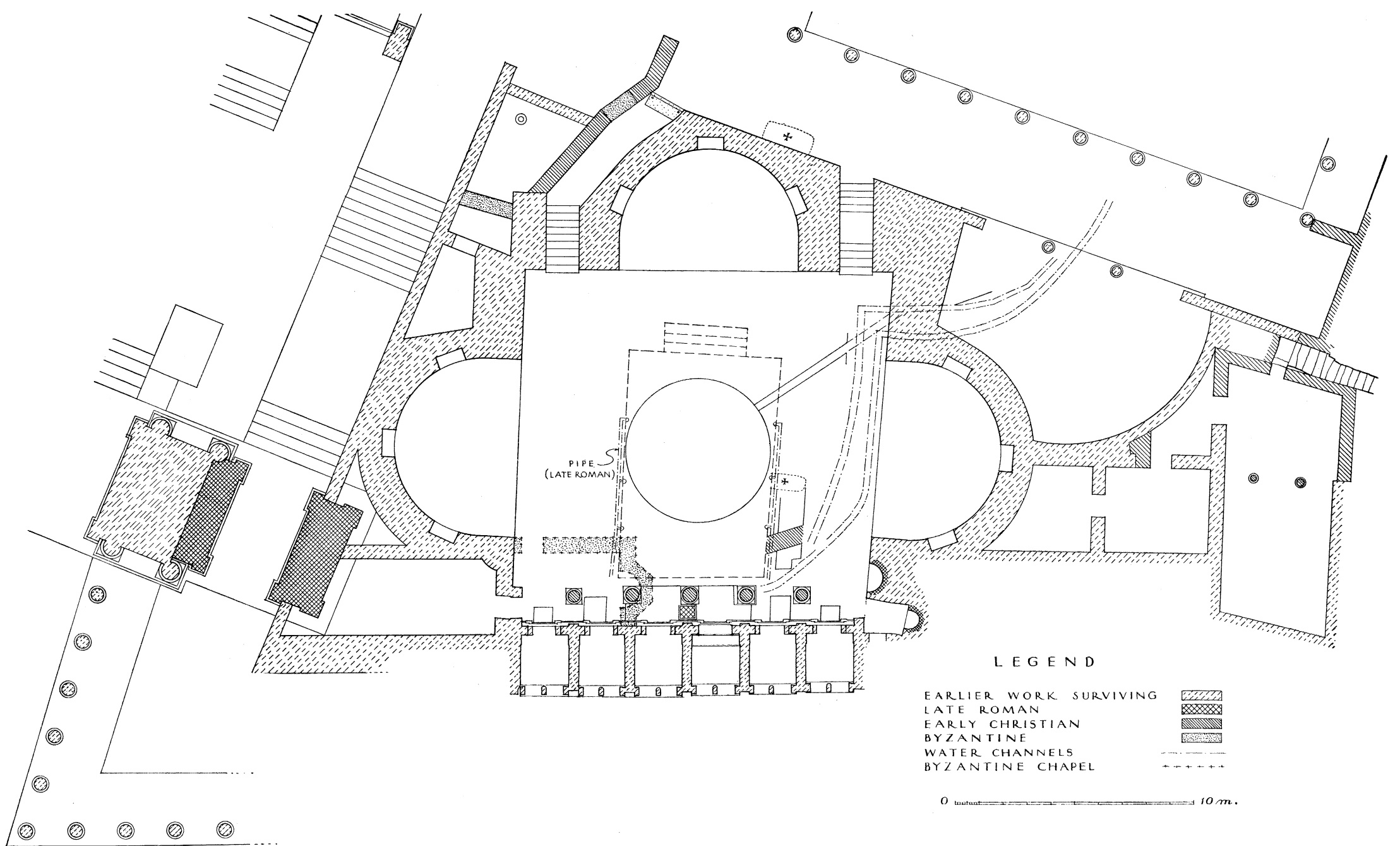
2. PEIRENE: RESTORED PLAN, LATE ROMAN AND BYZANTINE PERIODS
