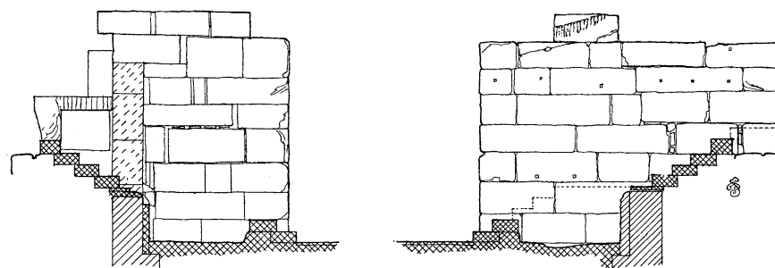
2. PEIRENE: SECTION THROUGH NORTH ENTRANCES, PRESENT STATE
