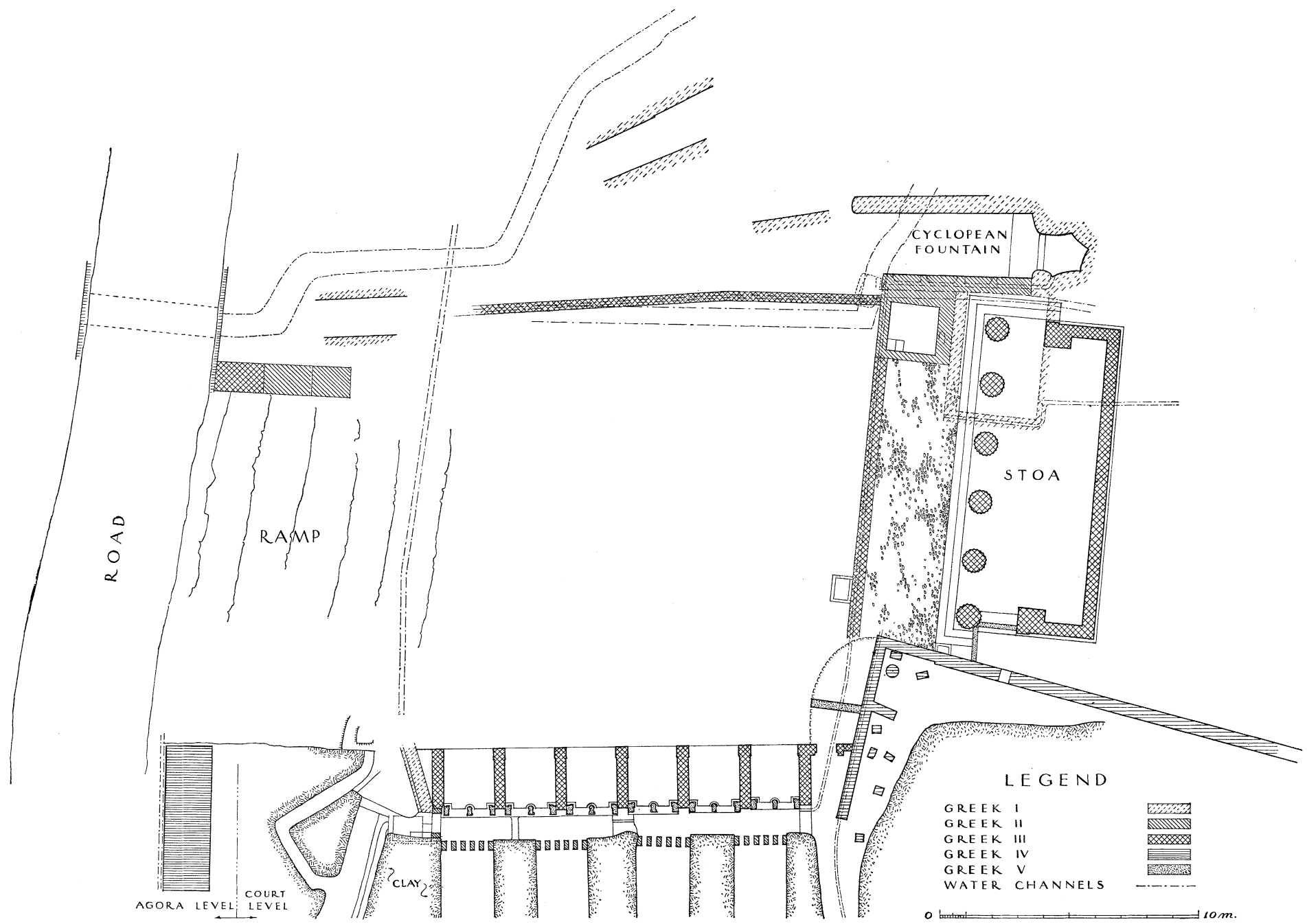
1. PEIRENE: RESTORED PLAN, GREEK PERIOD
