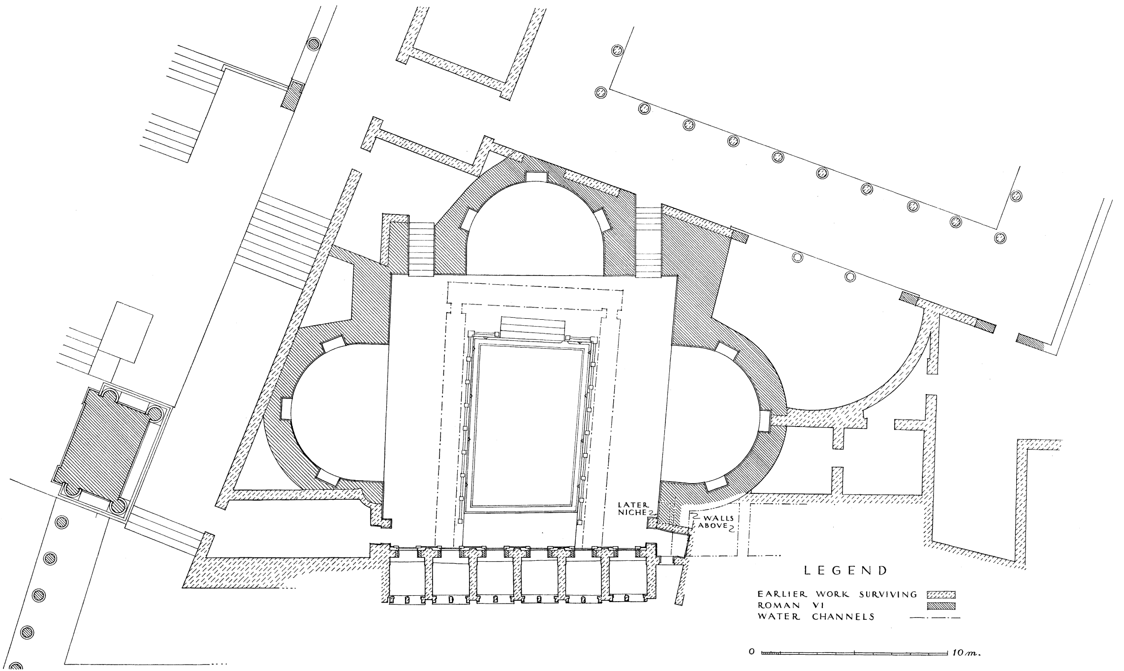
1. PEIRENE: RESTORED PLAN, PERIOD OF HERODES ATTICUS
