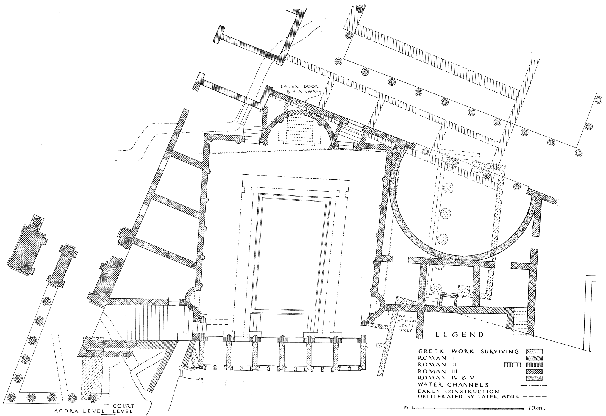
2. PEIRENE: RESTORED PLAN, EARLY ROMAN PERIOD
