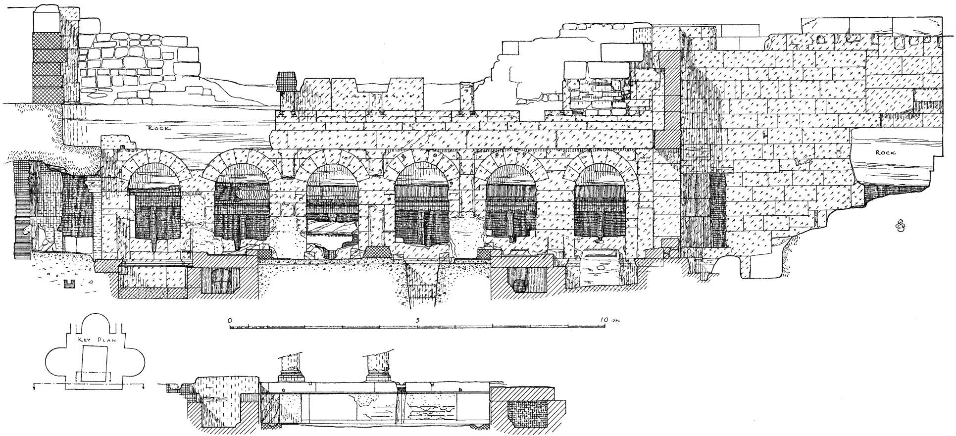
I. PEIRENE: ELEVATION OF FAÇADE AND SECTION THROUGH HYPAITHROS KRENE, PRESENT STATE
