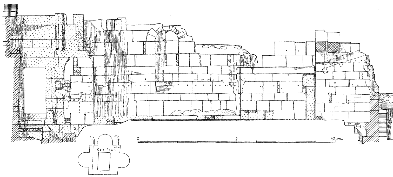
3. PEIRENE: ELEVATION OF WEST SIDE OF COURT, PRESENT STATE
