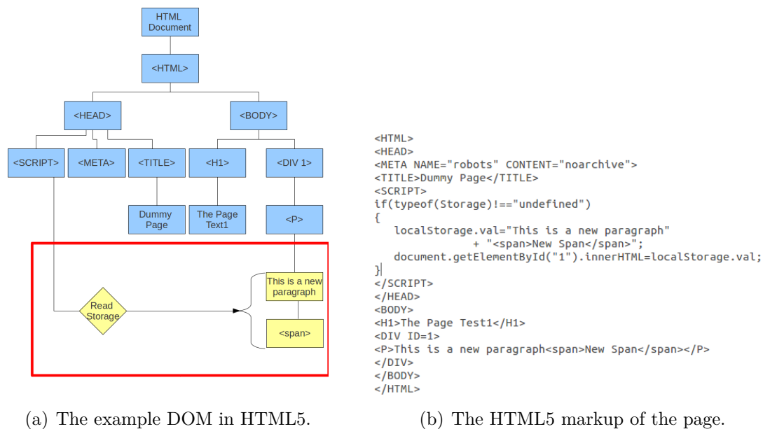
FIG. 19: Extending the example in Figure 15, HTML5 can read from local storage and modify the DOM.
