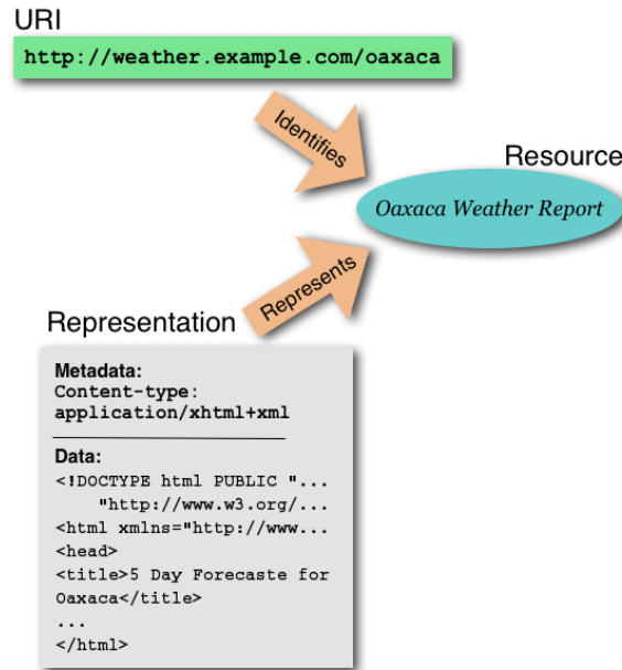
FIG. 9: An example from W3C of the URI-representation-resource relationship [135].
