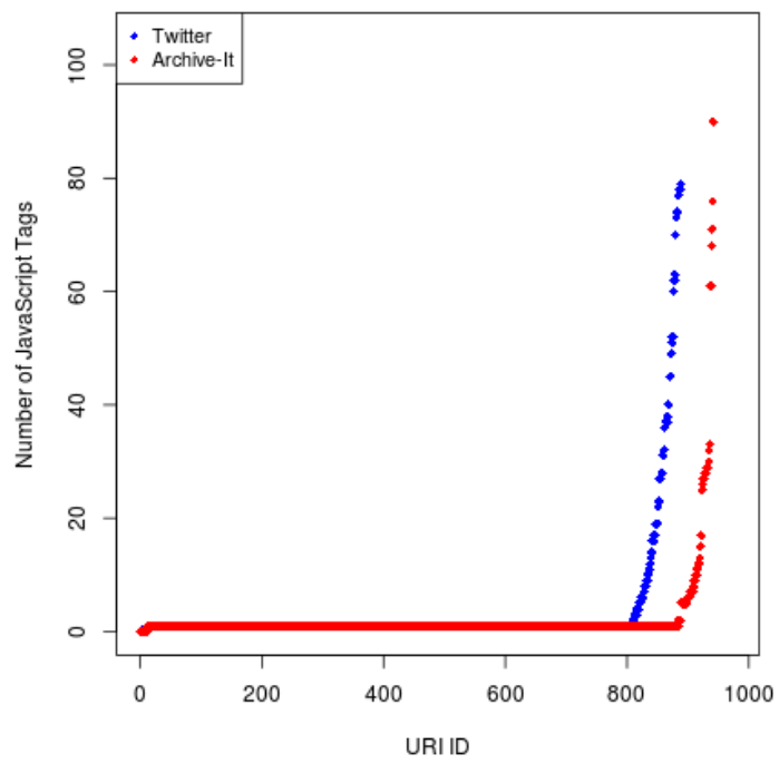
FIG. 58: CC of the HTML.
