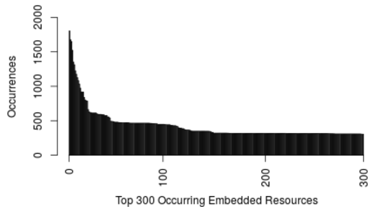
FIG. 100: The occurrence of embedded resources loaded into deferred representation descendants.
