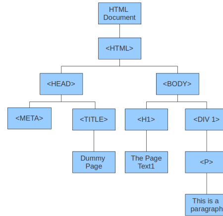
(b) An example HTML DOM for a default page
