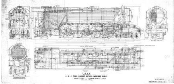
Doncaster Q-96 – L.N.E.R. 4-6-2 Three-Cylinder General Arrangement Passenger Engine General Arrangement [A1]
