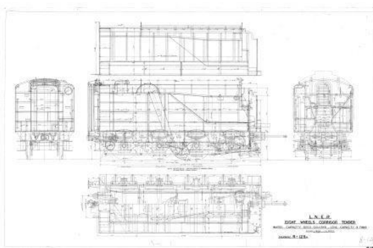
Doncaster R-129- L.N.E.R. Eight Wheels Corridor Tender [A3]
