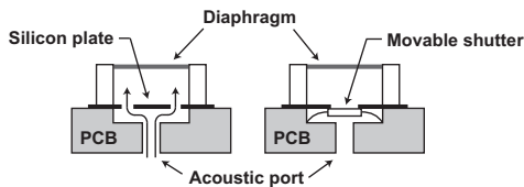
Fig. 13. Designs of MEMS microphone with light-blocking barriers [40]
