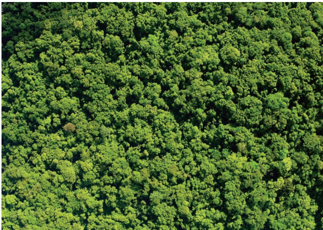
Plate 1: Lowland rainforest in the Middle Ramu area of Madang Province. Note the almost complete canopy cover.
