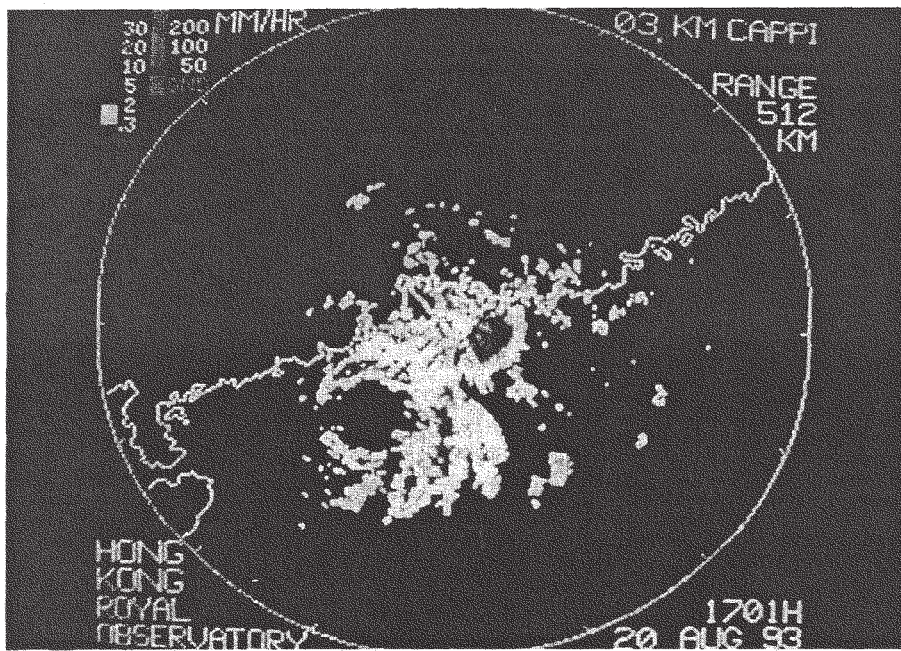
Figure 18. Radar display of the rain echoes of Tasha at 5.01 p.m. on 20 August 1993.
