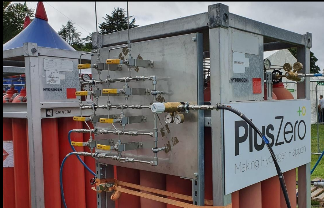
Compressed green H 2 gas storage in MCPs
