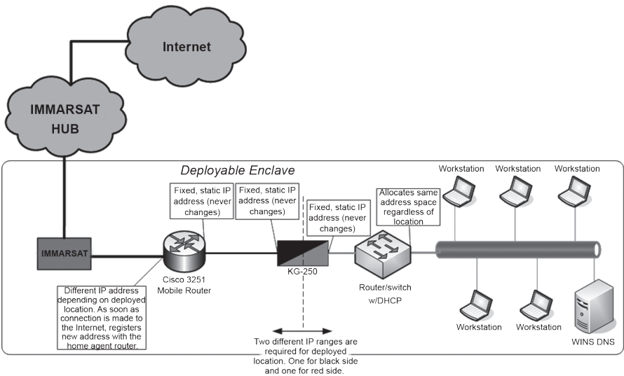
Figure G-5. Deployable Enclave with INMARSAT Connection
