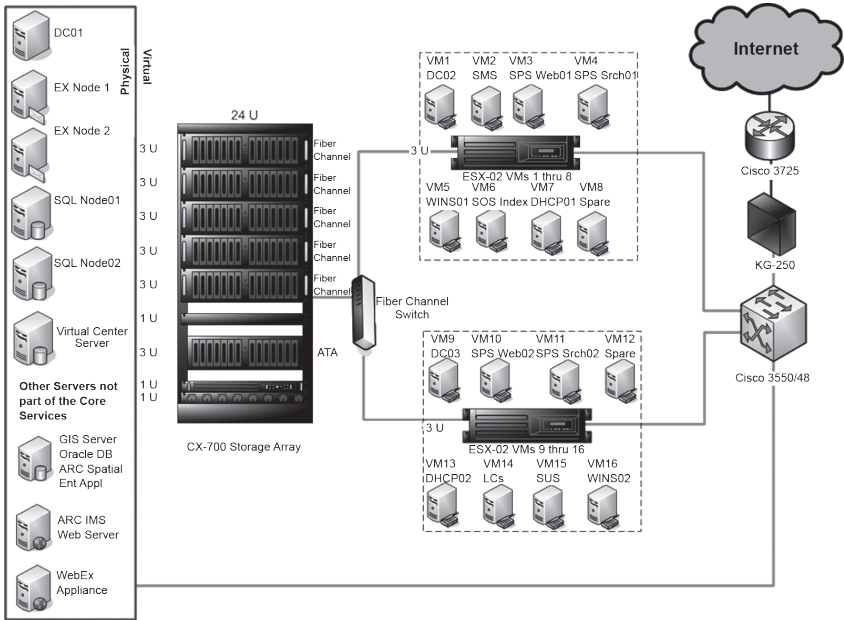
Figure G-2. Server Enclave
