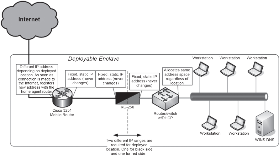
Figure G-4. Deployable Enclave with Direct Internet Connection
