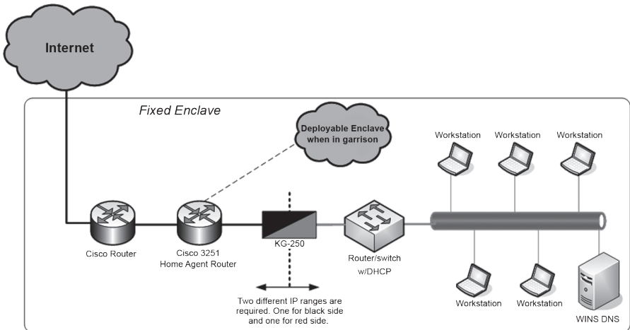
Figure G-3. Fixed Site Enclave
