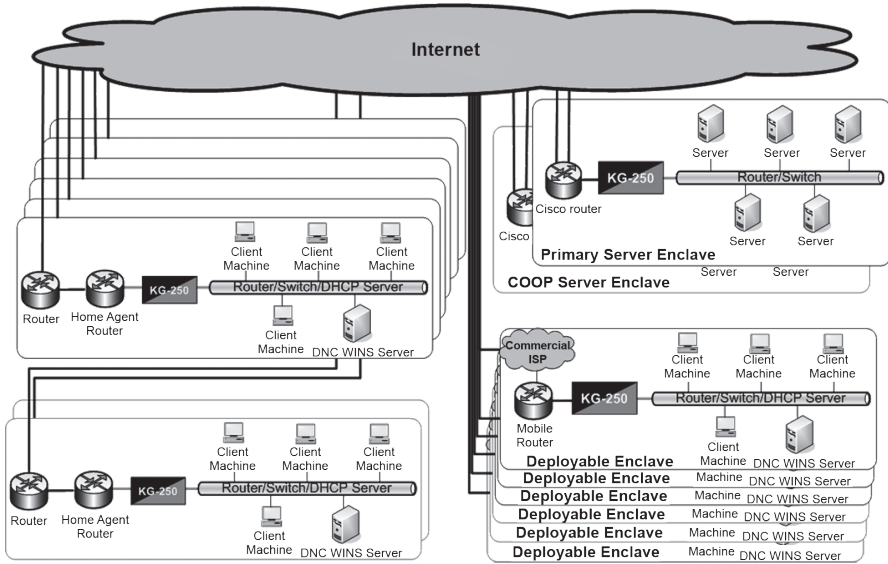
Figure G-1. Network Topology
