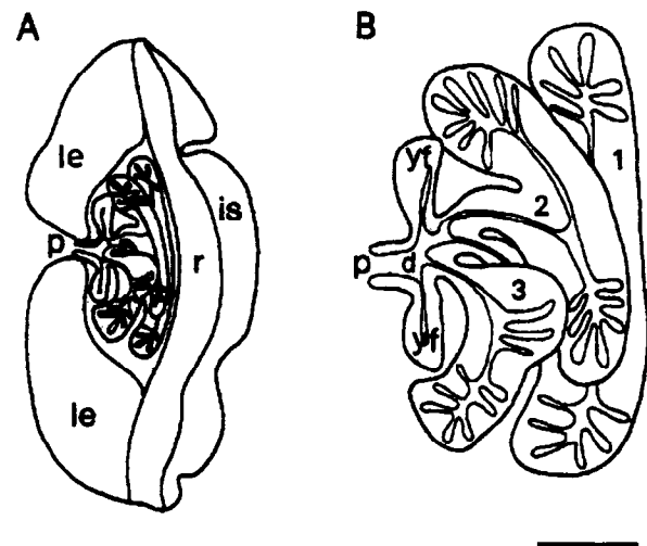
Figure 3. Relationship of the three bacteria-containing crypts (1, 2, and 3) to the ciliated duct (d) and the yellow filters (yf) in the left lobe of a fully differentiated light organ. (A) Frontal section through the left lobe of the light organ. (B) Enlargement of the crypts, yellow filters, and duct illustrated in (A). Diagrams based on examination of serial frontal sections of the light organ of a squid 8.0 mm in mantle length. is, ink sac; le, lens; p, pore; r, reflector. Bar, 250 \mu m.
