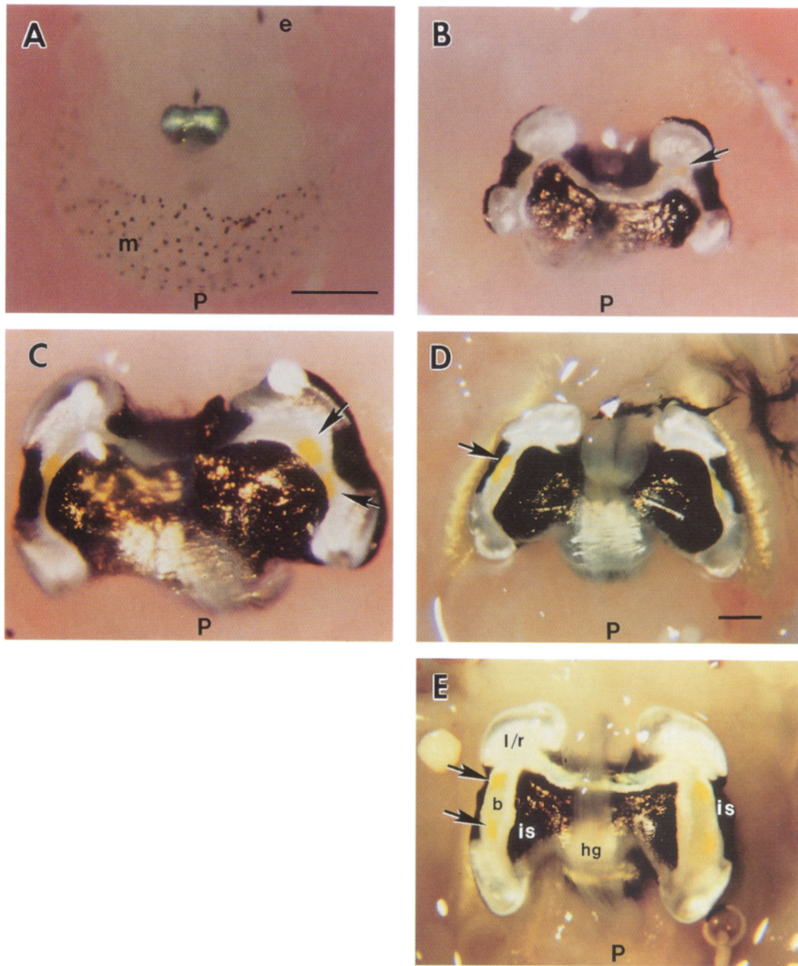
Figure 1. Postembryonic development of the light organ of Euprymna scolopes . [Animals were placed against a pink background to provide contrast to the squid light organ tissues.] Ventral views of the light organ of a (A) newly hatched juvenile 1.6 mm in mantle length; m, mantle; e, eye; (B) juvenile 2.8 mm in mantle length; (C) juvenile 4.0 mm in mantle length; (D) sexually mature male 18 mm, and (E) 20 mm in mantle length. The bacteria-containing tissue (b) is dorsal to the yellow filters (arrows in B–D) and appears opaque against the brilliantly silver reflector. The reflector and the lens (l/r), which occurs ventral to the reflector, run much of the length of each lobe. Diverticula of the ink sac (is) expand and contract over the bacteria-containing tissue to control the intensity of light emission. Bar (A–C), 500 \mu m, (D–E), 1 mm; hg, hindgut; P, posterior.
