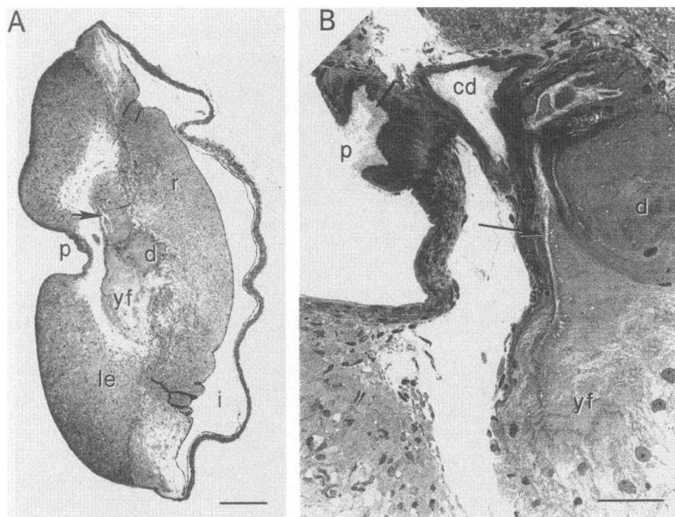
Figure 5. The yellow filters (yf) appear as a fibrous tissue outpocketing from the ciliated duct in these Richardson-stained frontal sections through one lobe of a mature light organ. (A) The posterior filter is shown fully in this section. The arrow indicates the lumen of the ciliated duct leading into the posterior filter. Bar, 250 \mu\text{m} . (B) This section reveals a portion of the ciliated duct (arrow) that leads from the pore region into the posterior filter (for orientation, see Fig. 3B). Bar, 50 \mu\text{m} . cd, ciliated duct; d, duct; le, lens; p, pore; r, reflector.
