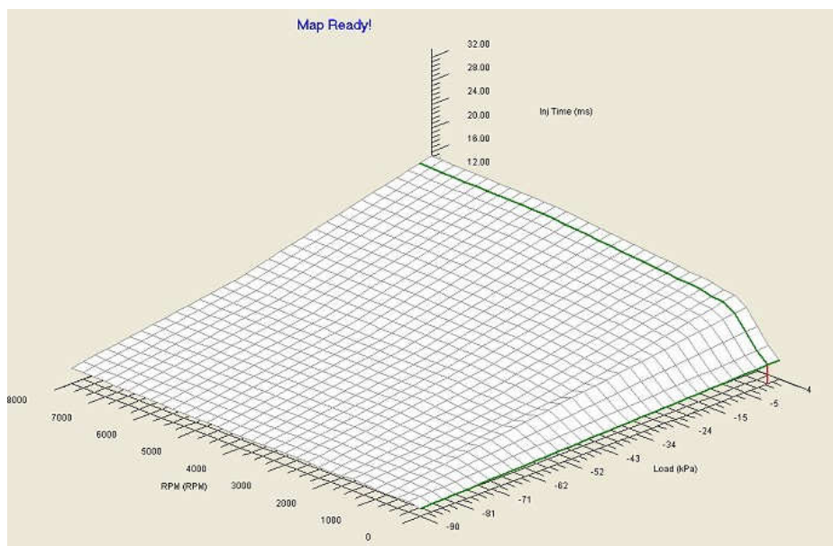
Above is the 3D fuel map used under the dyno testing performed in this report.
