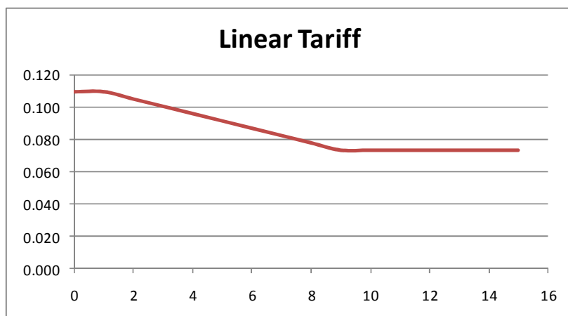
Figure A1: Linear tariff: hydro 1 >= 8MW
