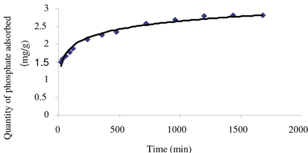
Fig. (4). Adsorption kinetics of phosphate on Ad-brut.
