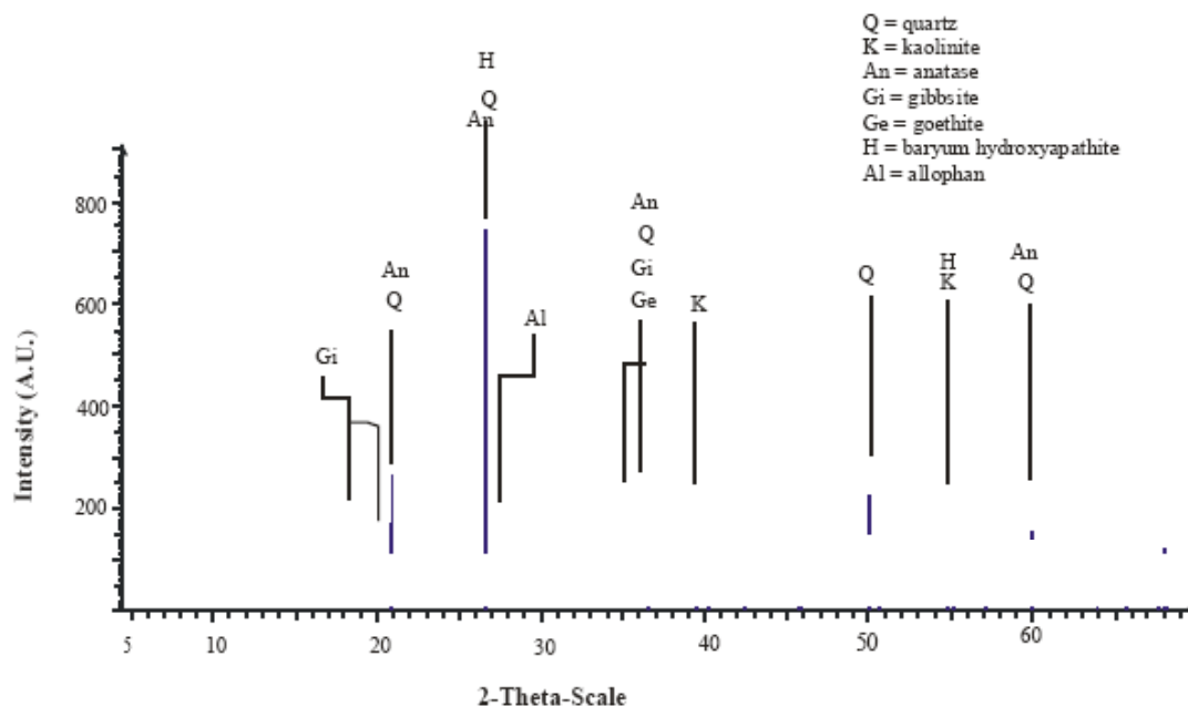
Fig. (2). X-ray diffractogram of Ad-brut.
