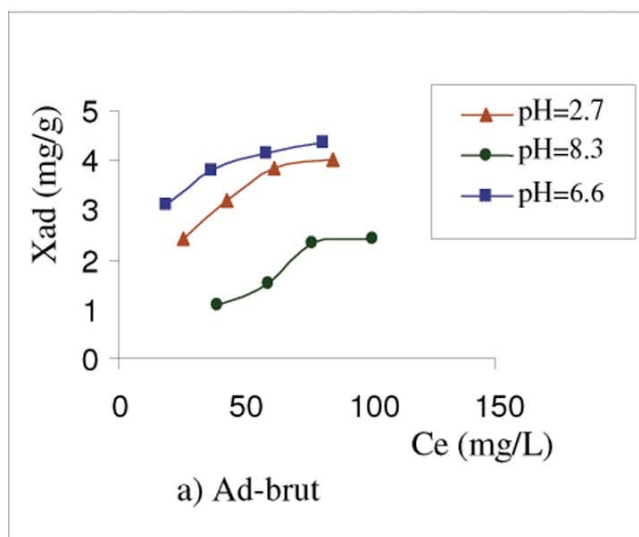
Figs. (8a and b). pH influence on phosphate ions adsorption over Ad-brut and Ad-H 2 O 2 samples.
