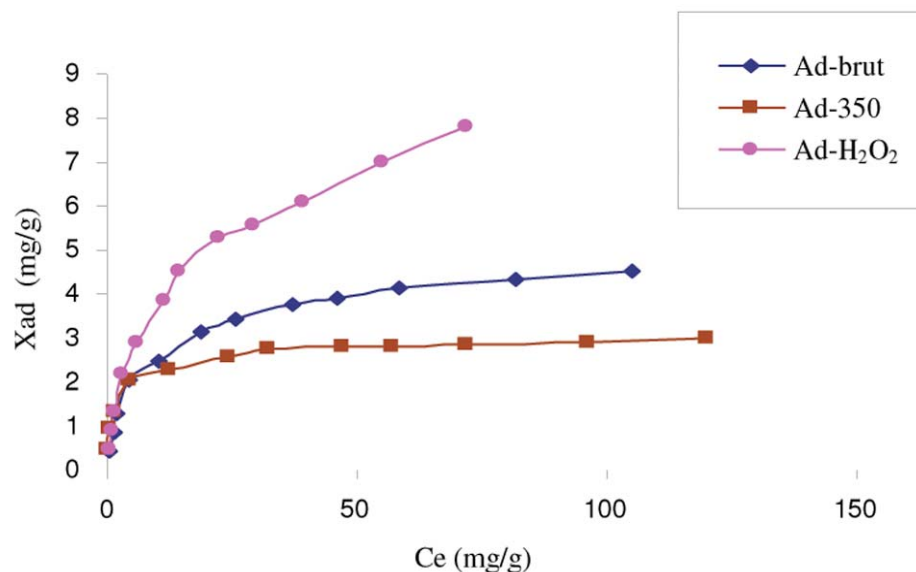
Fig. (7). Phosphate ions adsorption isotherms on each sample with the results fitted to the Langmuir equation.
