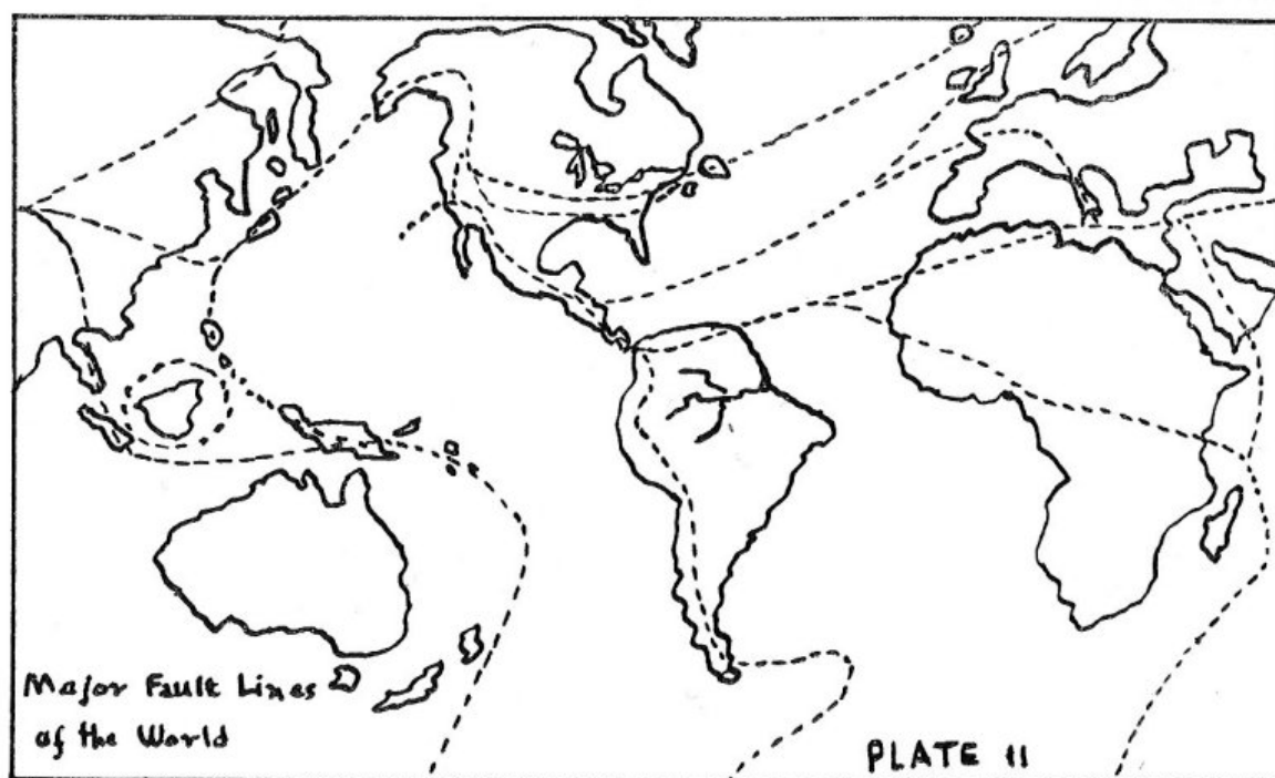
Plate II. Major Fault Lines of the World
